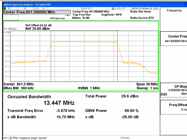
Band26 Part22 / 15MHz / 64QAM/ High CH
