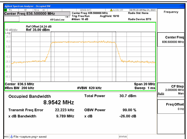
Band26 Part22 / 10MHz / 16QAM/ Mid CH
