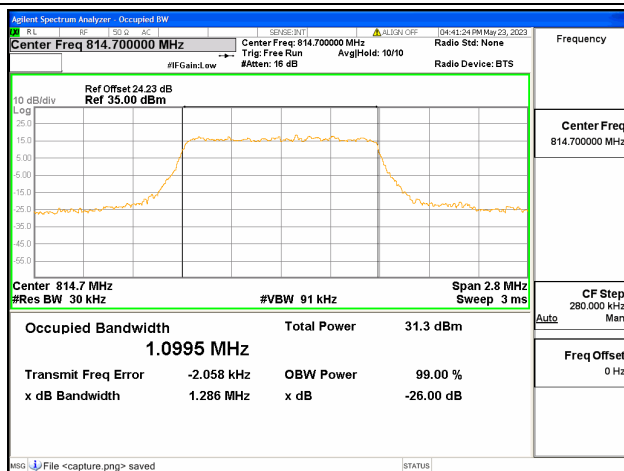
Band26 Part90 / 1.4MHz / QPSK/ Low CH
