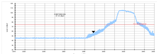
802.11g-Channel 3 Peak
