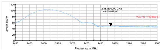
802.11b-Channel 11 Peak
