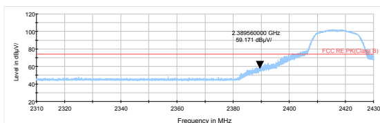
802.11g-Channel 2 Peak
