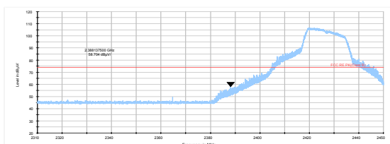
802.11g-Channel 4 Peak
