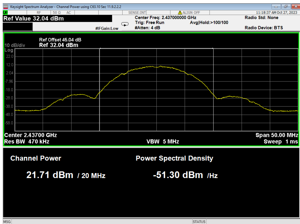
Figure 4 – Radiated Average Power Measurement, 802.11b
