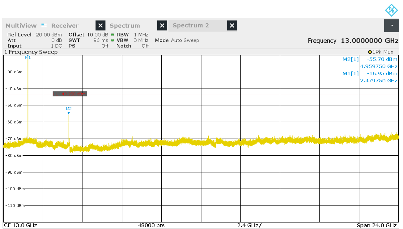
Figure 28: Chart of emissions test from 1 GHz to 25 GHz on highest channel, Pk
