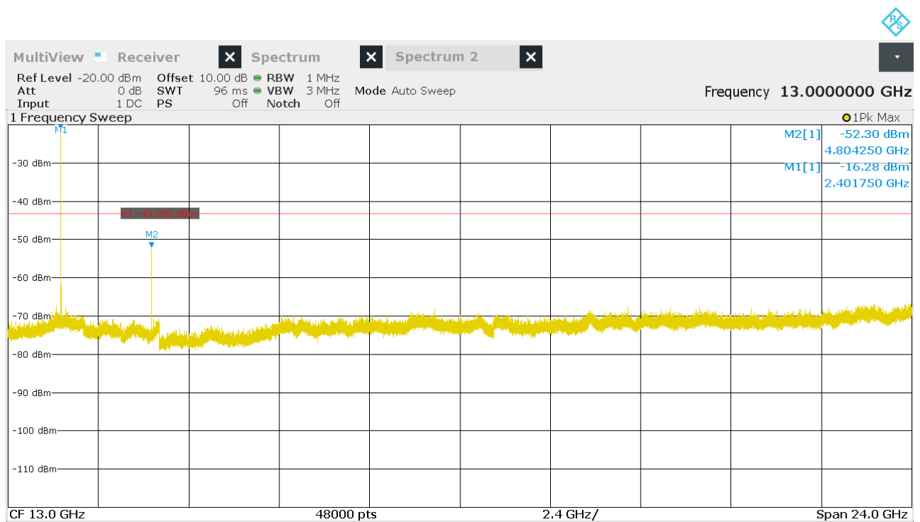
Figure 24: Chart of emissions test from 1 GHz to 25 GHz on lowest channel, Pk
