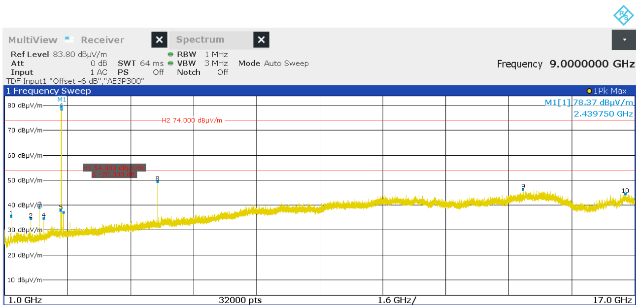
Figure 33: Chart of radiated emissions pre-measurement from 1 GHz to 17 GHz on middle channel, EUT position X, antenna polarization horizontal
