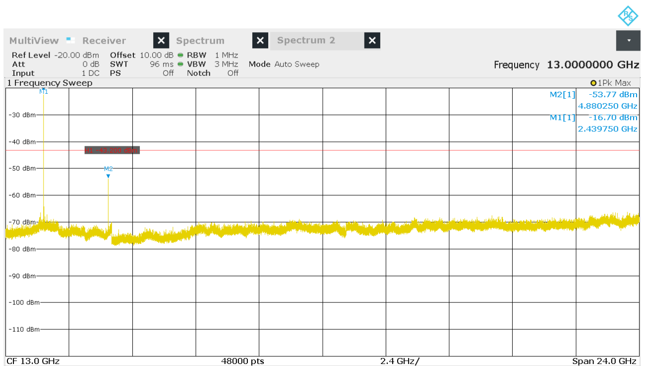
Figure 26: Chart of emissions test from 1 GHz to 25 GHz on middle channel, Pk
