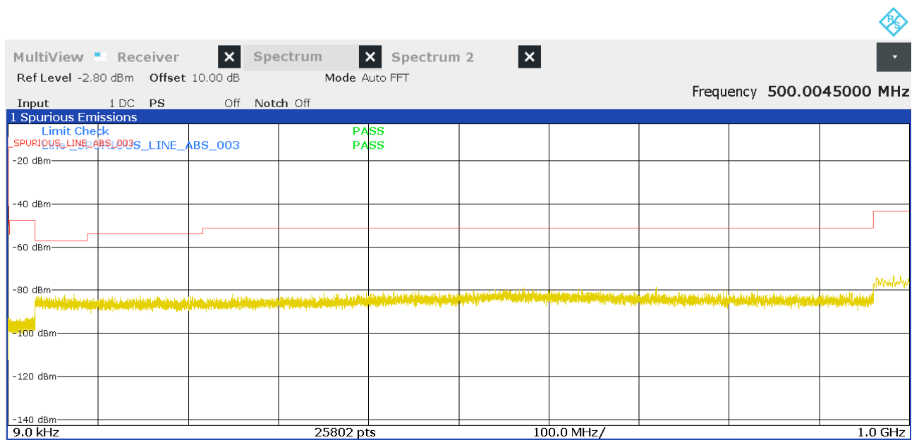
Figure 25: Chart of emissions test from 9 kHz to 1 GHz on middle channel, PK
