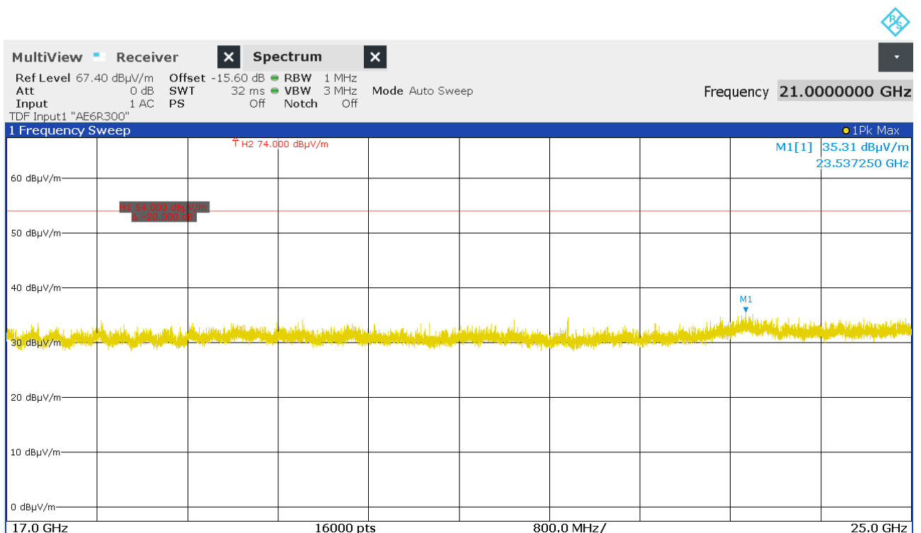
Figure 34: Chart of exploratory emissions measurement from 17 GHz to 25 GHz on middle channel, EUT position X, antenna polarization horizontal
