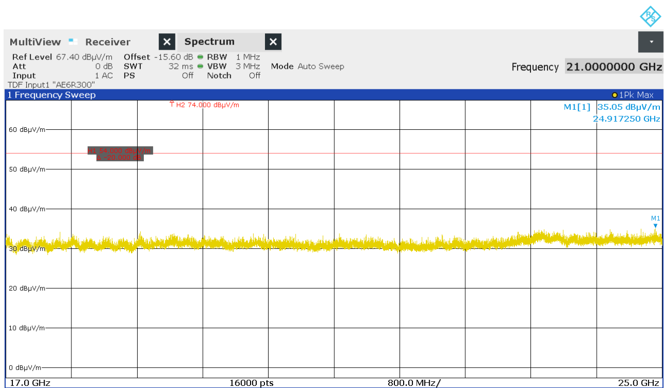
Figure 36: Chart of exploratory emission test from 17 GHz to 25 GHz on highest channel at 0.5 m, EUT position X, antenna polarization horizontal
