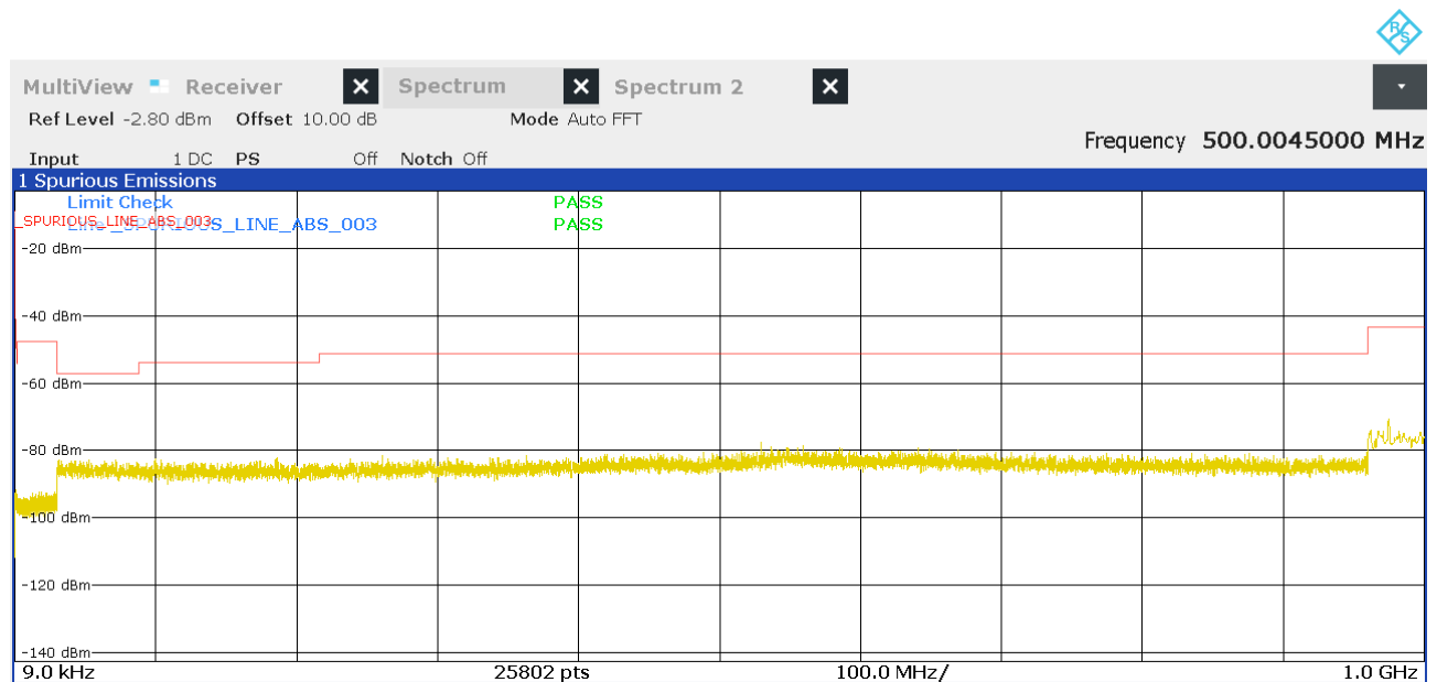
Figure 23: Chart of emissions test from 9 kHz to 1 GHz on lowest channel, PK
