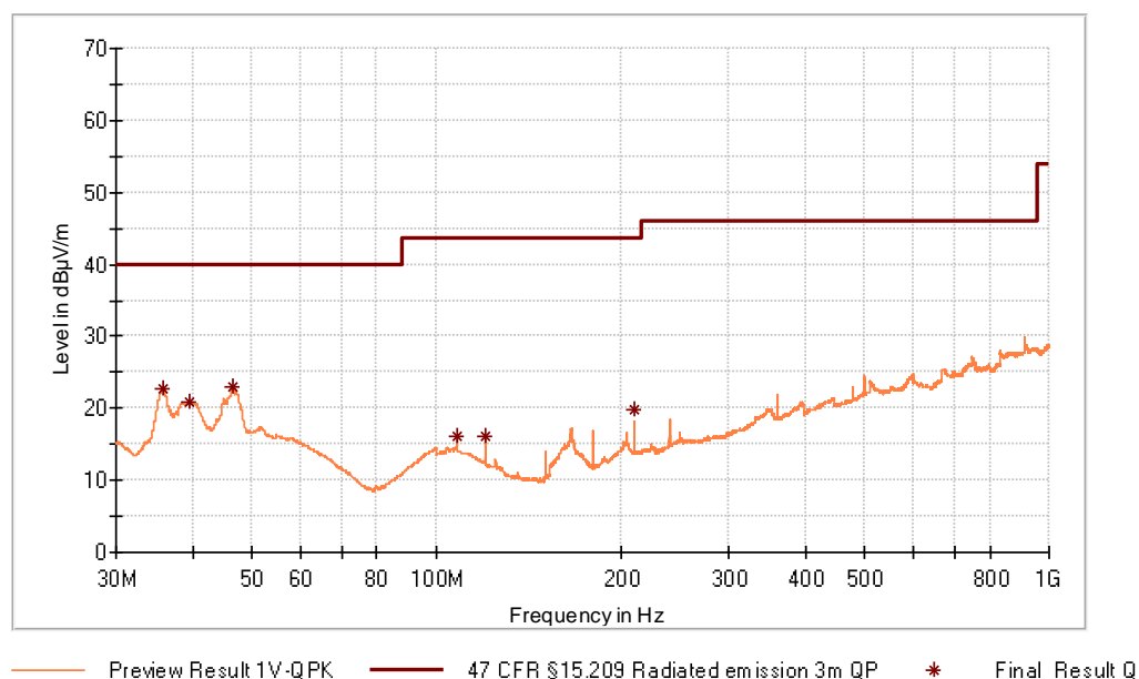
Figure 30: Chart of radiated emissions test from 30 MHz to 1 GHz on highest channel, EUT position Z, antenna polarization vertical
