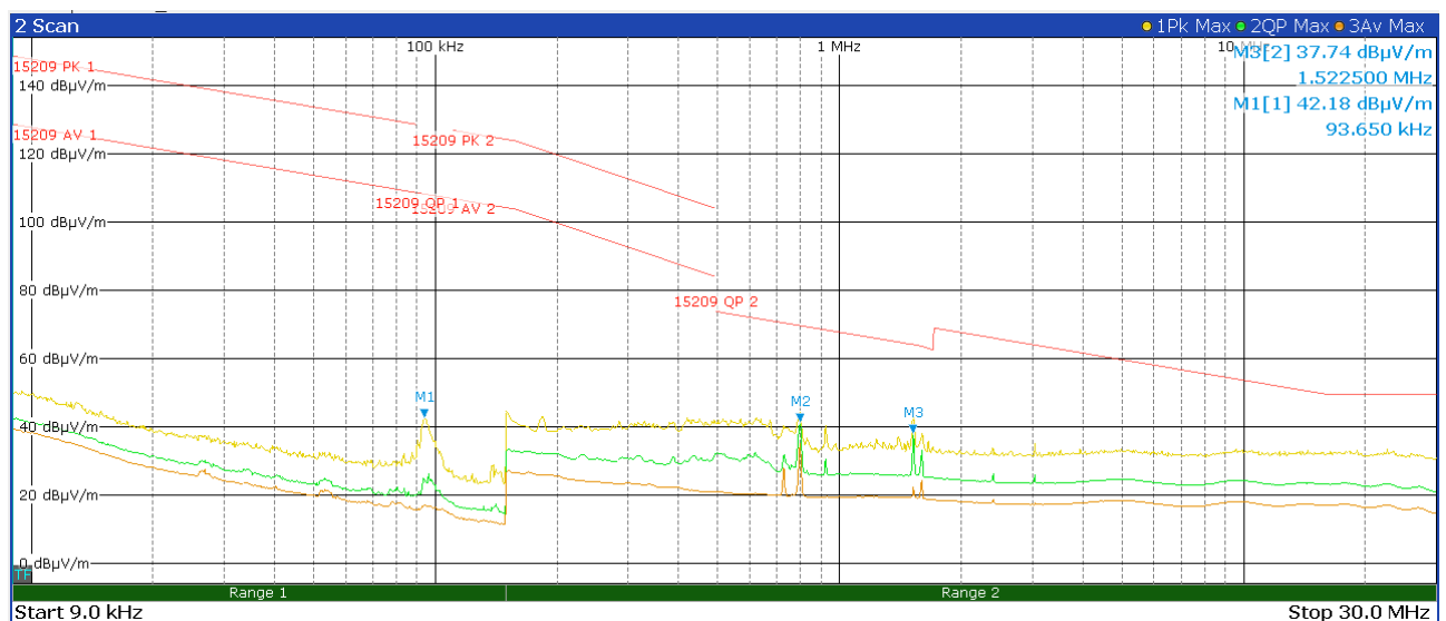
Figure 29: Chart of emissions test below 30 MHz on lowest channel, EUT position Y, antenna parallel
