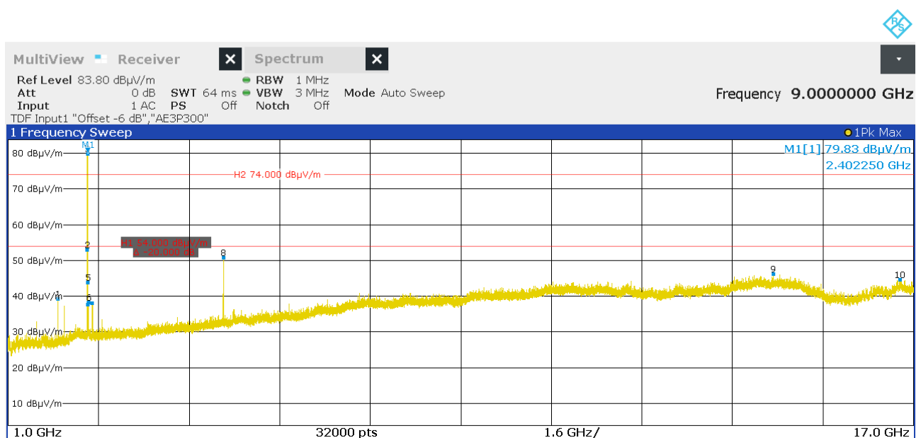
Figure 31: Chart of radiated emissions pre-measurement from 1 GHz to 17 GHz on lowest channel, EUT position X, antenna polarization horizontal
