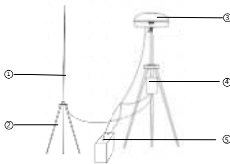
Figure 2.1.1-1 External radio of base station
