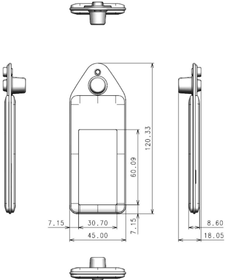
Figure 3 Mechanical Dimension
