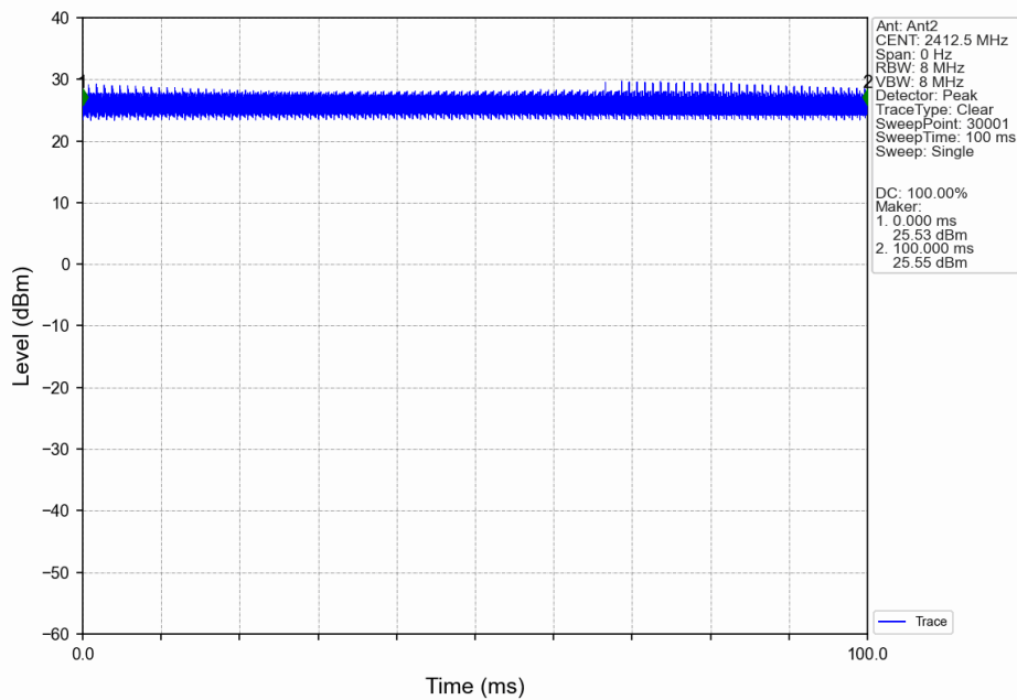
20M_LCH_2412.5MHz_Ant2_NTNV
