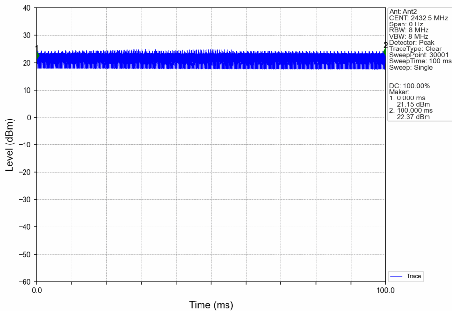
60M_LCH_2432.5MHz_Ant2_NTNV
