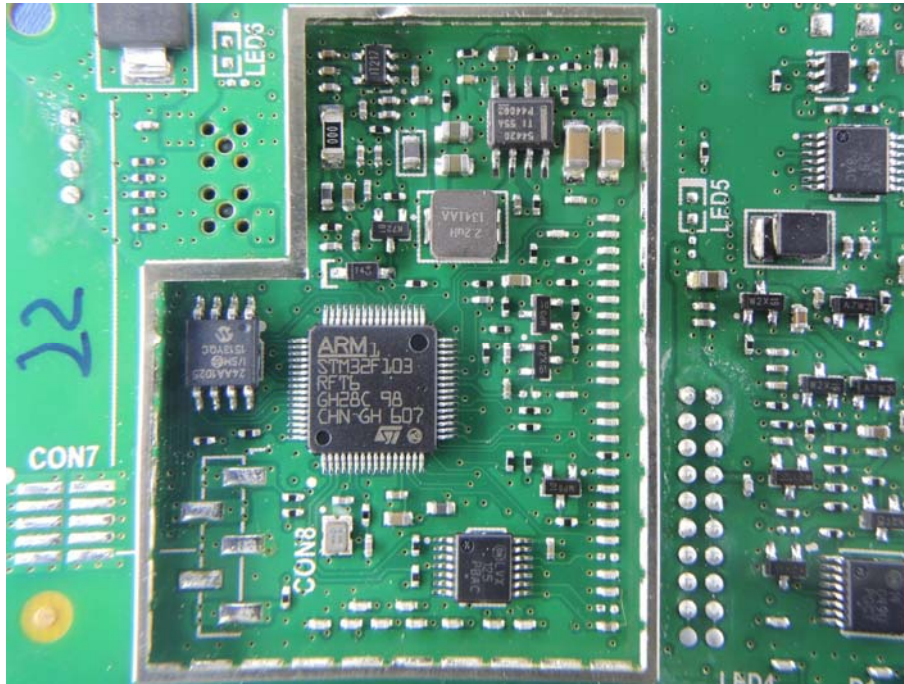
(23) EUT Photo
