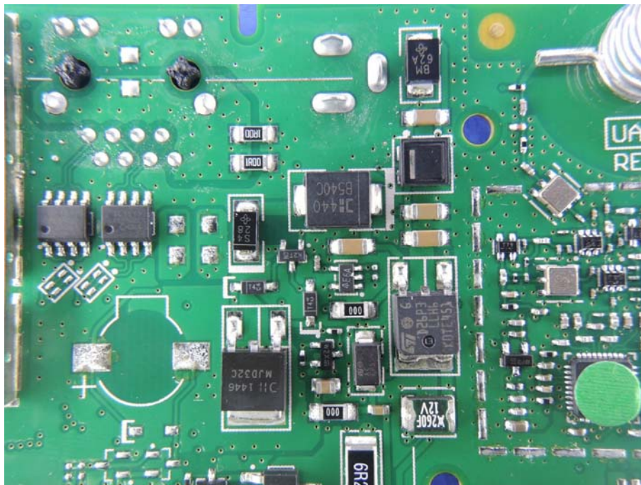
(25) EUT Photo
