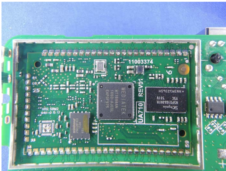
(22) EUT Photo
