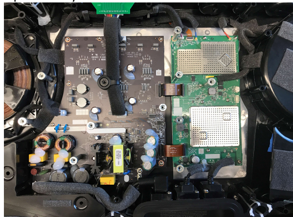
Detail of PCBA in product
