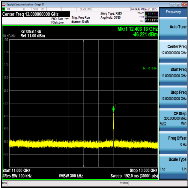
ZIGB-Ant1-2480-11000~13000-PASS
