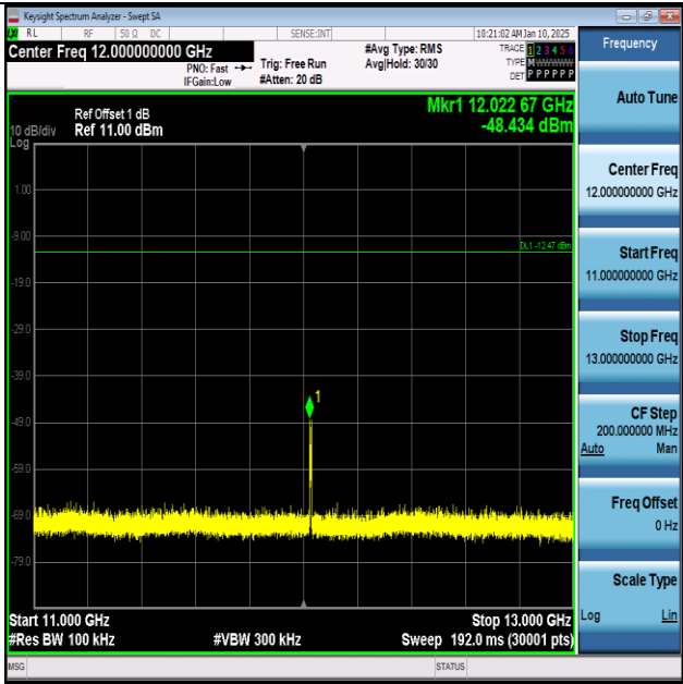
ZIGB-Ant1-2405-11000~13000-PASS
