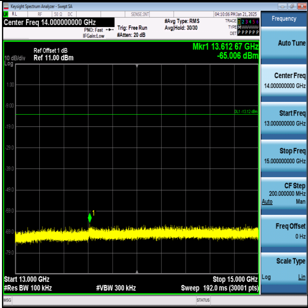
ZIGB-Ant1-2480-13000~15000-PASS
