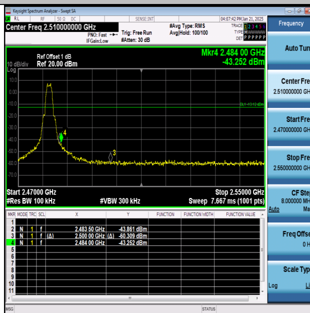
ZIGB-Ant1-2480-PASS
