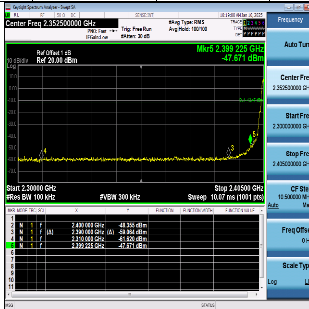
ZIGB-Ant1-2405-PASS
