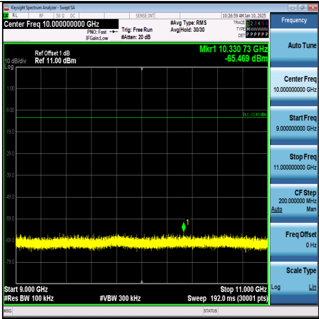
ZIGB-Ant1-2440-9000~11000-PASS
