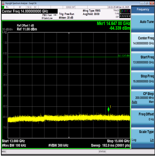
ZIGB-Ant1-2405-13000~15000-PASS
