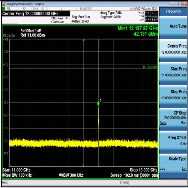
ZIGB-Ant1-2440-11000~13000-PASS
