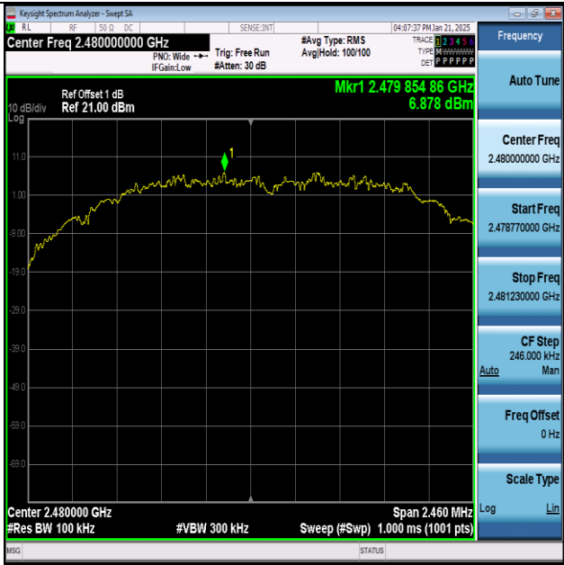
ZIGB-Ant1-2480-PASS
