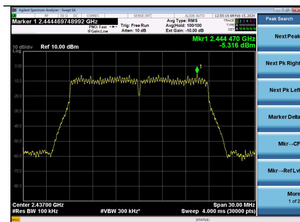
802.11n20 | Channel 6 | MCS7
