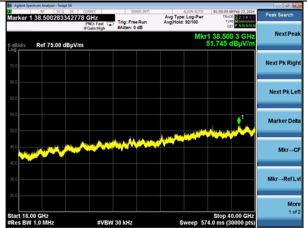
802.11b | Channel 6 | 1 Mbps 18000-40000 MHz | Vertical
