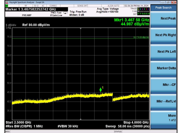
802.11ax20 | Channel 11 | MCS0 | RU38 2500-4000 MHz | Vertical
