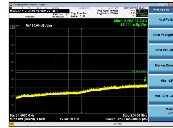
802.11ax40 | Channel 3 | MCS0 | RU38 1000-2310 MHz | Vertical
