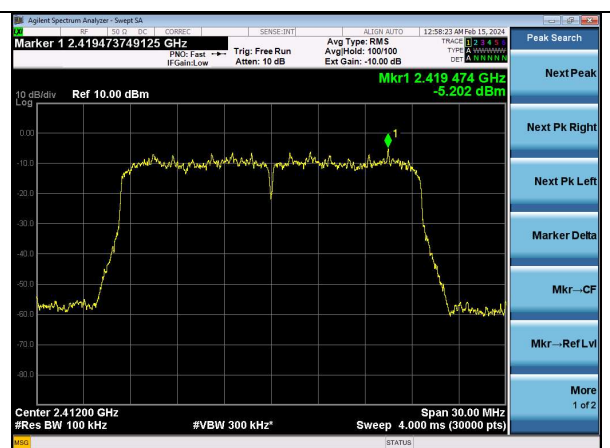
802.11ax20 | Channel 1 | MCS9
