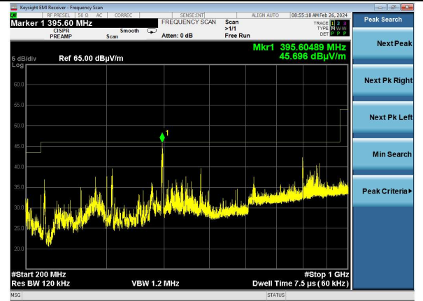
802.11b | Channel 6 | 1 Mbps | 200-1000 MHz | Vertical
