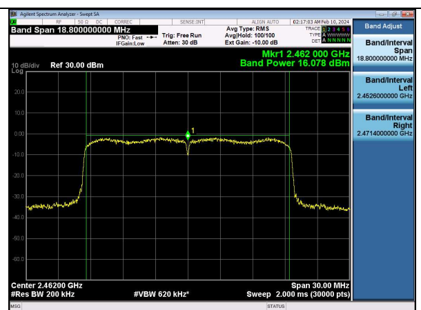
802.11ax20 | Channel 11 | MCS0
