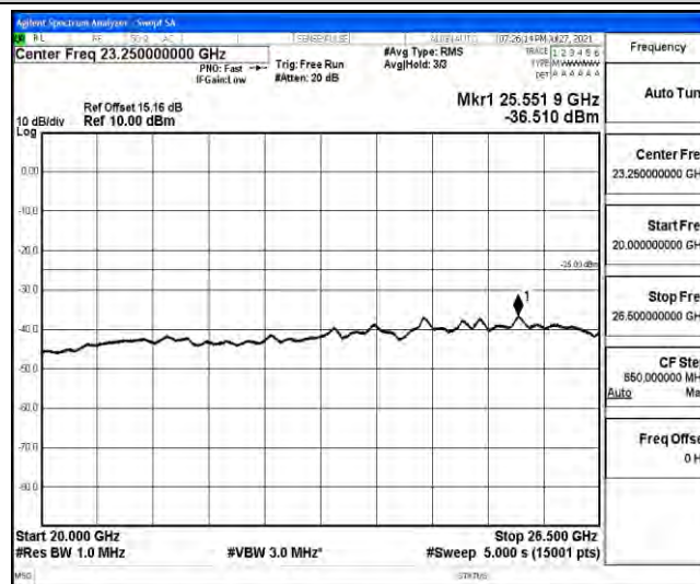
Band41-20MHz-QPSK-41490-1RB#0-Range1:0.009~0.15MHz
