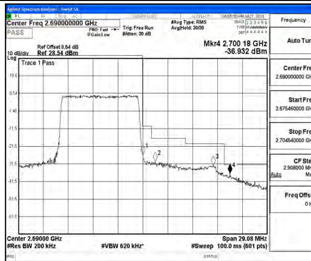
Band41-10MHz-16QAM-39700-50RB#0
