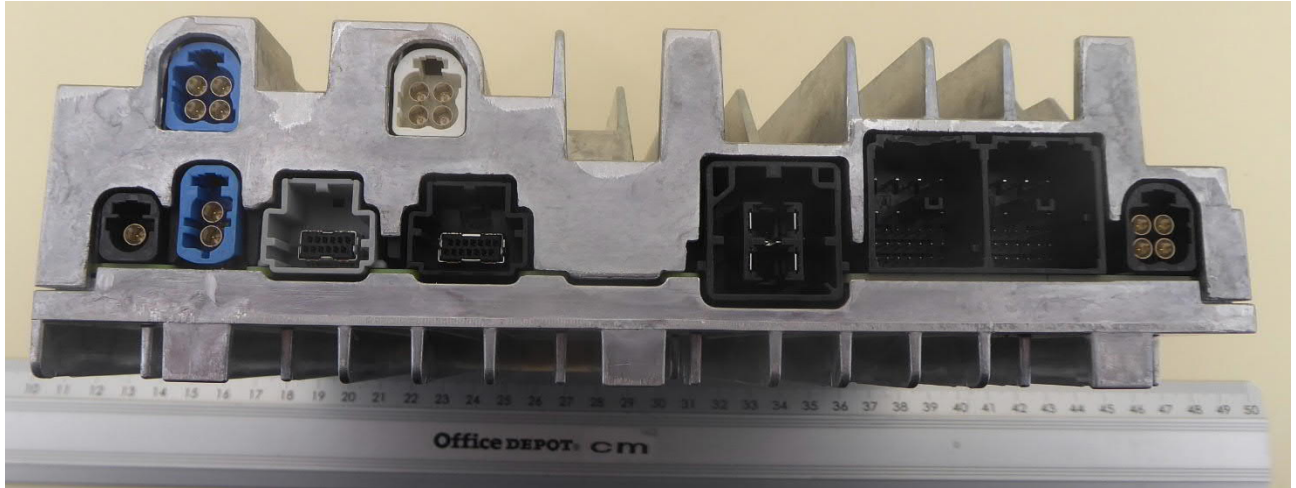
EUT – connectors
