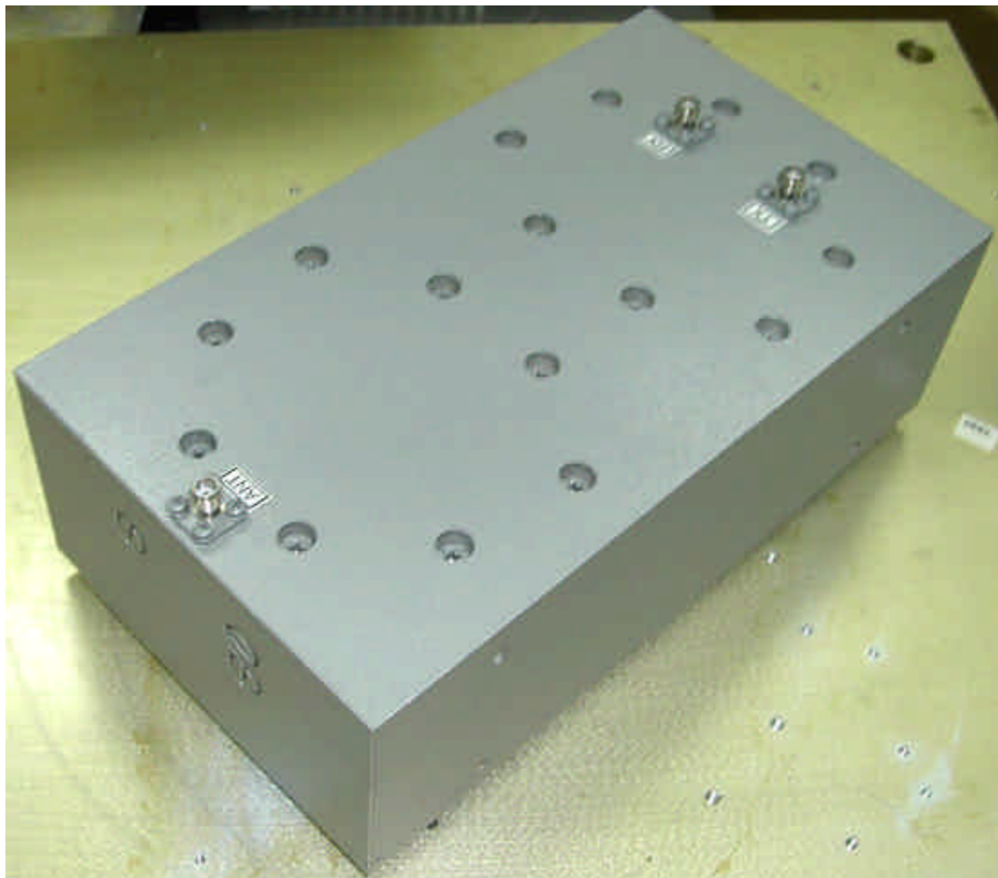
Photograph No.11 MW-BDA-ESMR-50W90 high power repeater Mobile diplexer second side view
