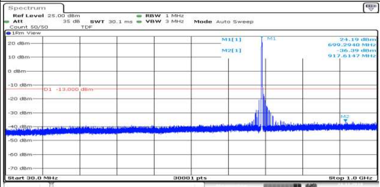
Band12_1.4MHz_QPSK_23017_1_0_Low_30_1000_-36.39_PASS__
