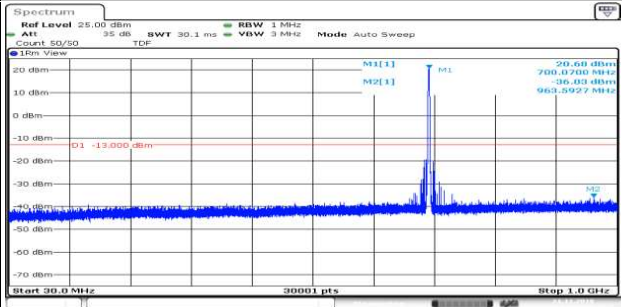
Band12_1.4MHz_QPSK_23017_6_0_Low_30_1000_-36.03_PASS__
