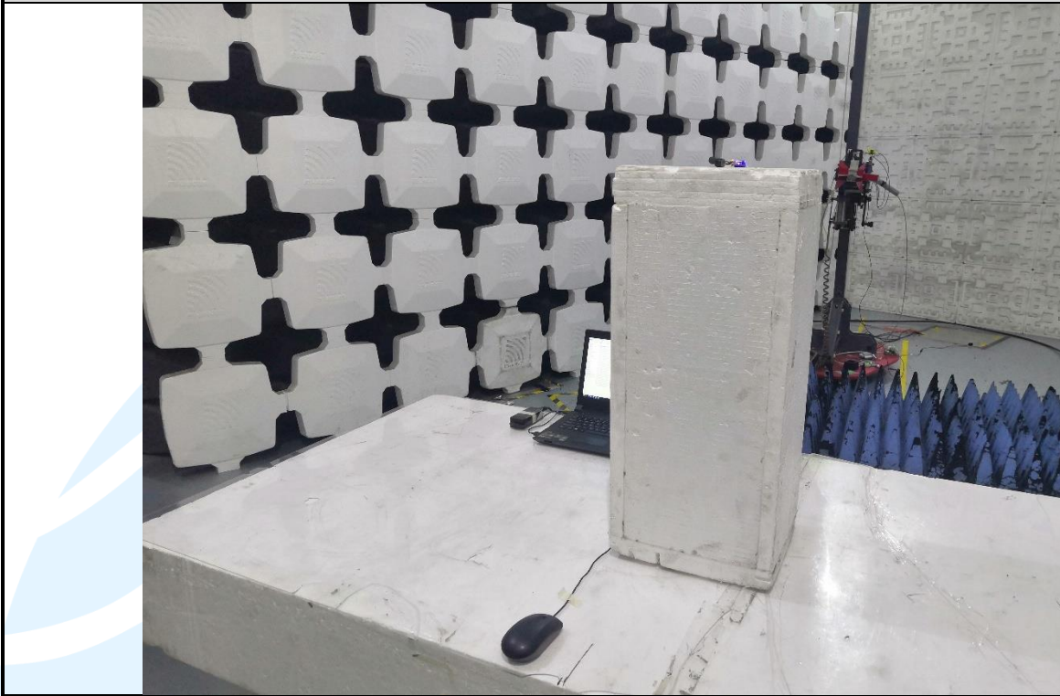
Radiated emission Test Setup (Above 1 GHz) –Left Earbuds
