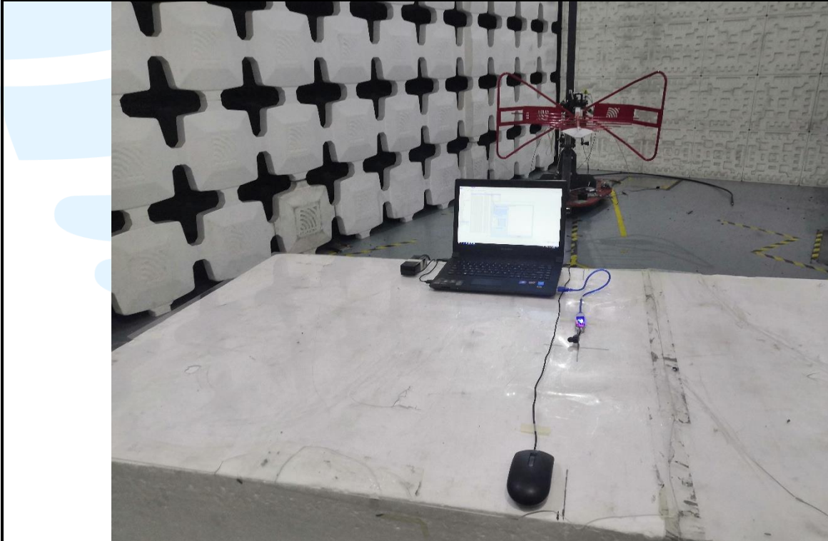
Radiated emission Test Setup (30 MHz~1 GHz) –Right Earbuds
