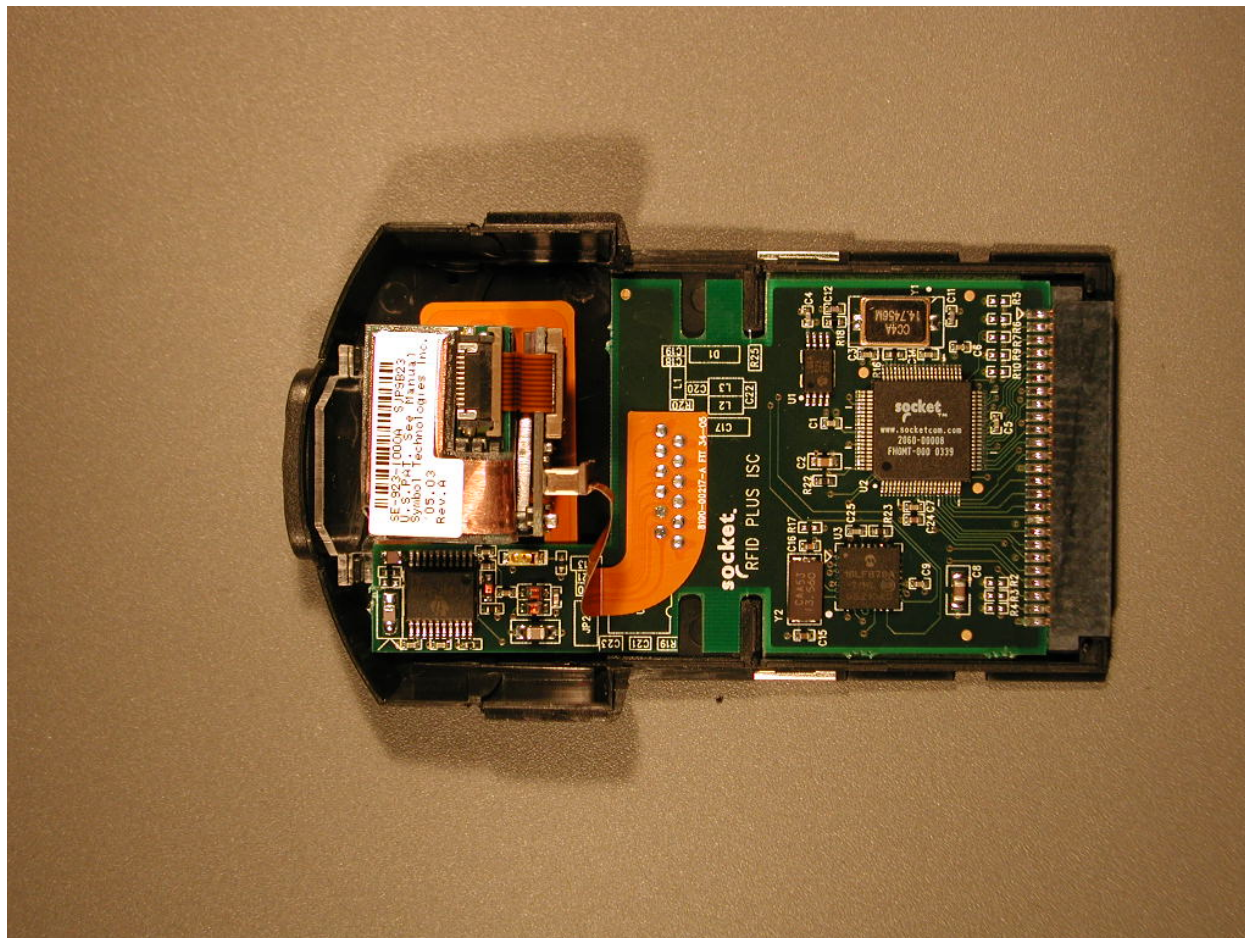
EUT PCB Top View
