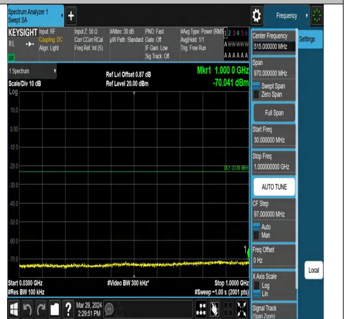
Band66_1.4MHz_QPSK_132322_1RB#0_30~1000_30~1000
