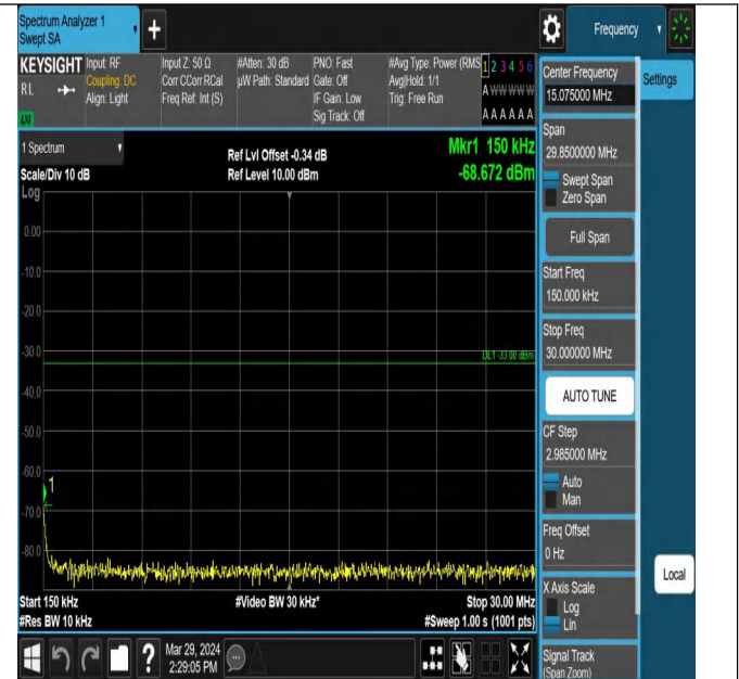
Band66_1.4MHz_QPSK_131979_1RB#0_0.15~30_0.15~30
