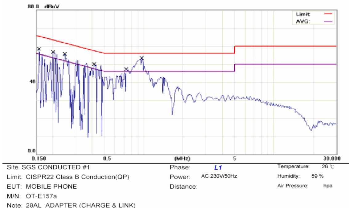
Conducted Emission Measurement
