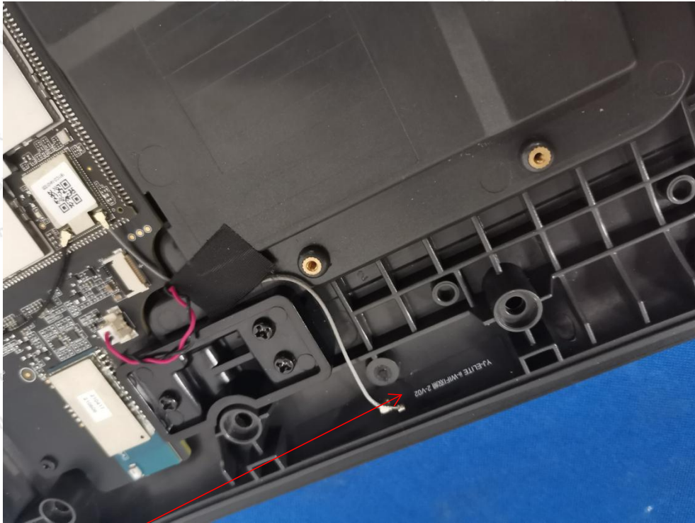
WLAN ANT2
