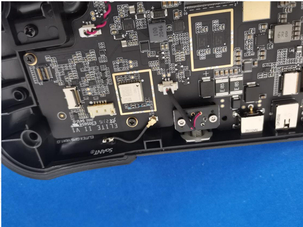
WLAN ANT2
