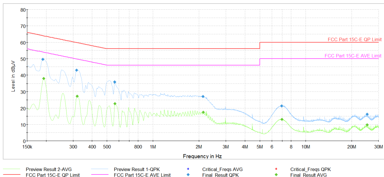
Plot 7-32. AC Line Conducted Plot with Bluetooth LE (L1, 1Mbps – Ch.39 with host PC with USB-C cable)
