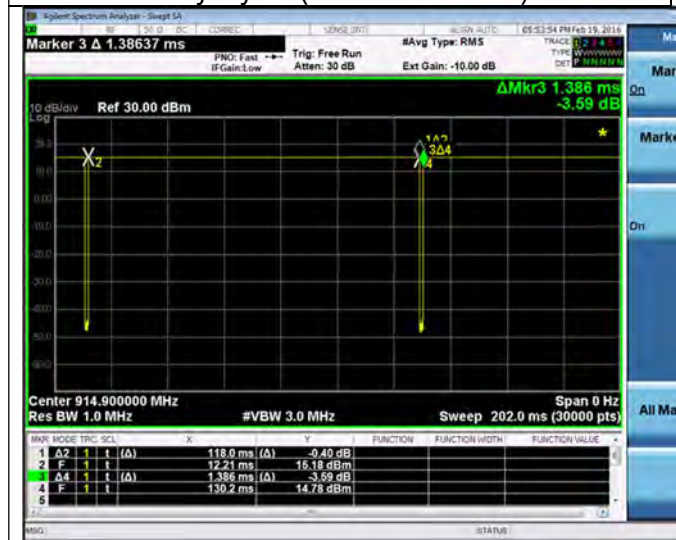
Duty Cycle (125k Hz – SF 7)
