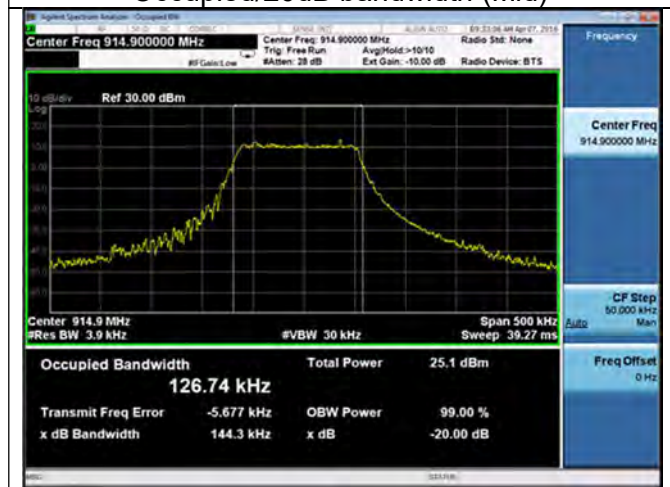
Occupied/20dB bandwidth (High)
