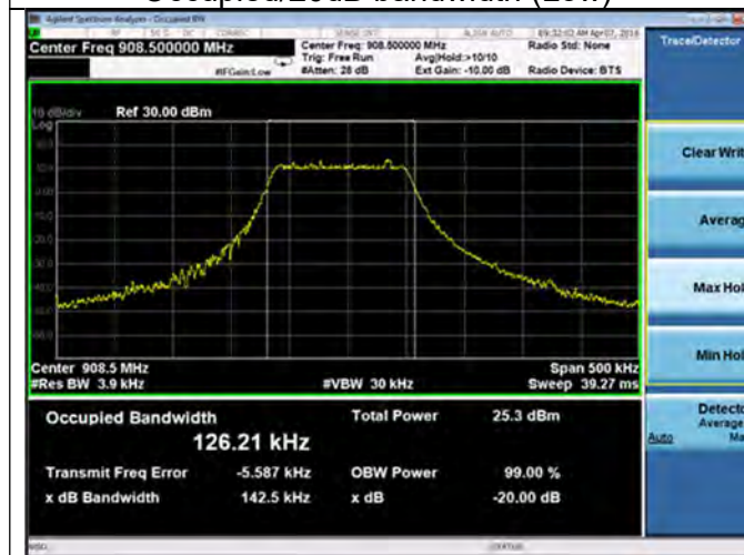
Occupied/20dB bandwidth (Mid)
