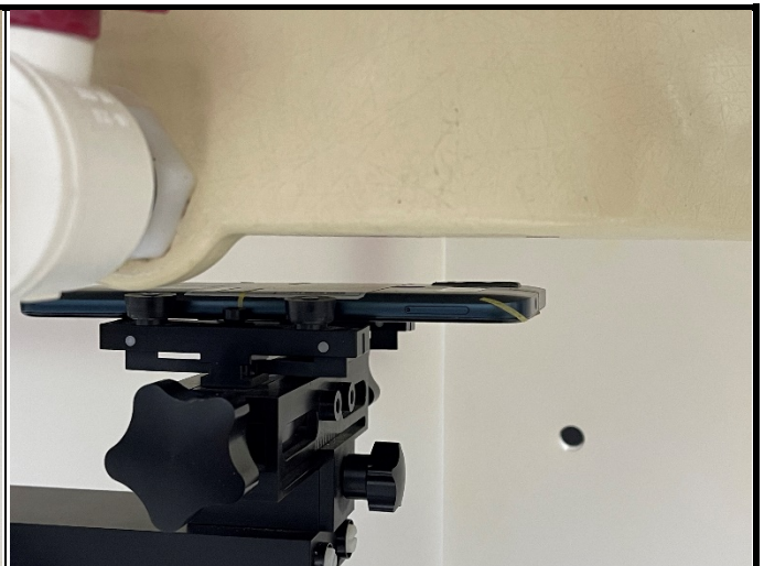
Rear Face of EUT with 1.8 cm Gap
