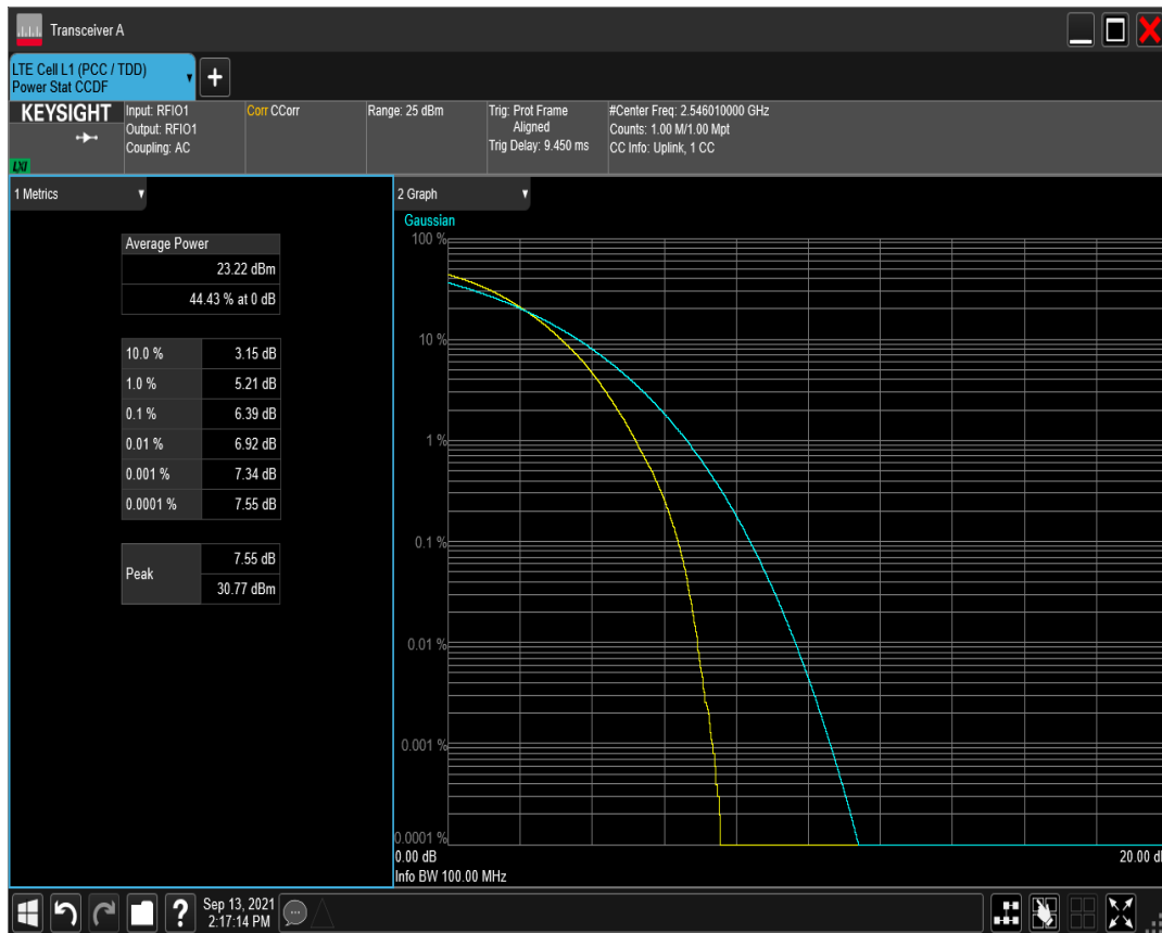
n41 SCS=30kHz DFT_QAM64 BW=100MHz Channel=509202 RB=270@0
