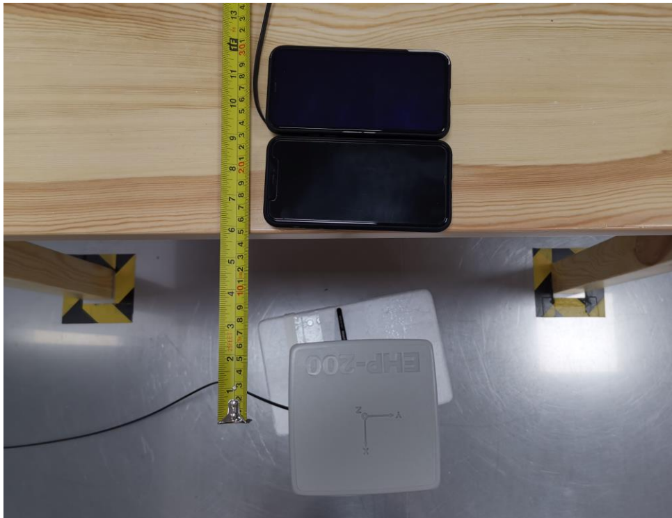
Test setup of C side with Coil 1 + Coil 2
