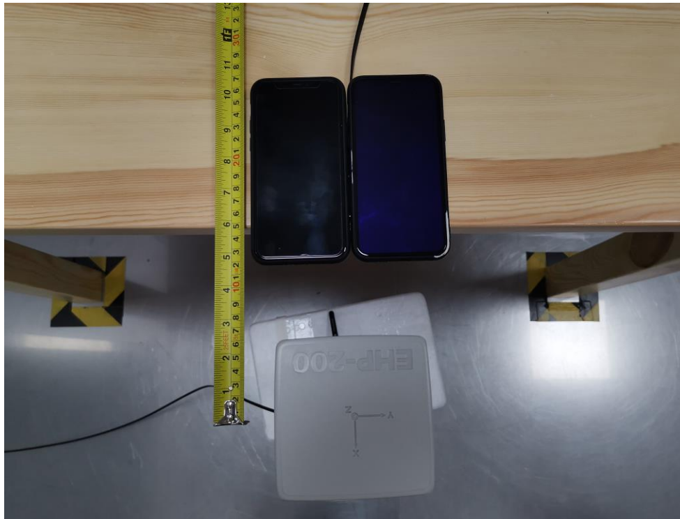
Test setup of A side with Coil 1 + Coil 2
