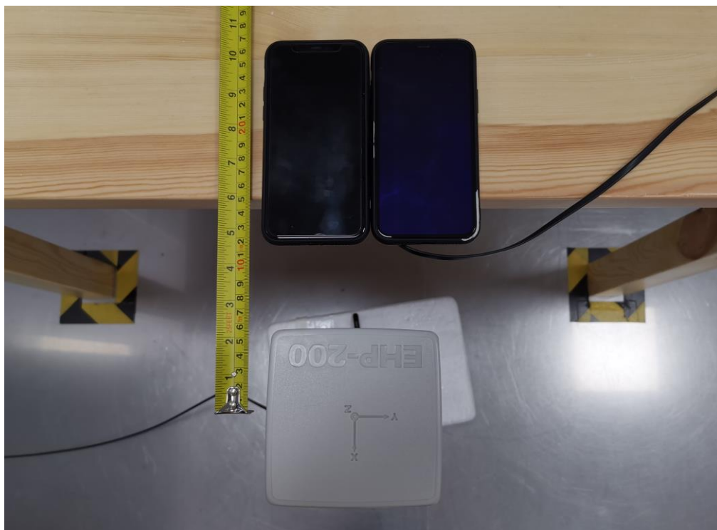
Test setup of B side with Coil 1 + Coil 2
