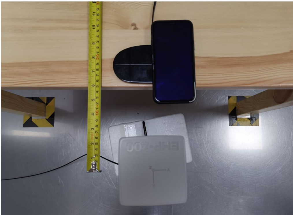
Test setup of A side with Coil 2
