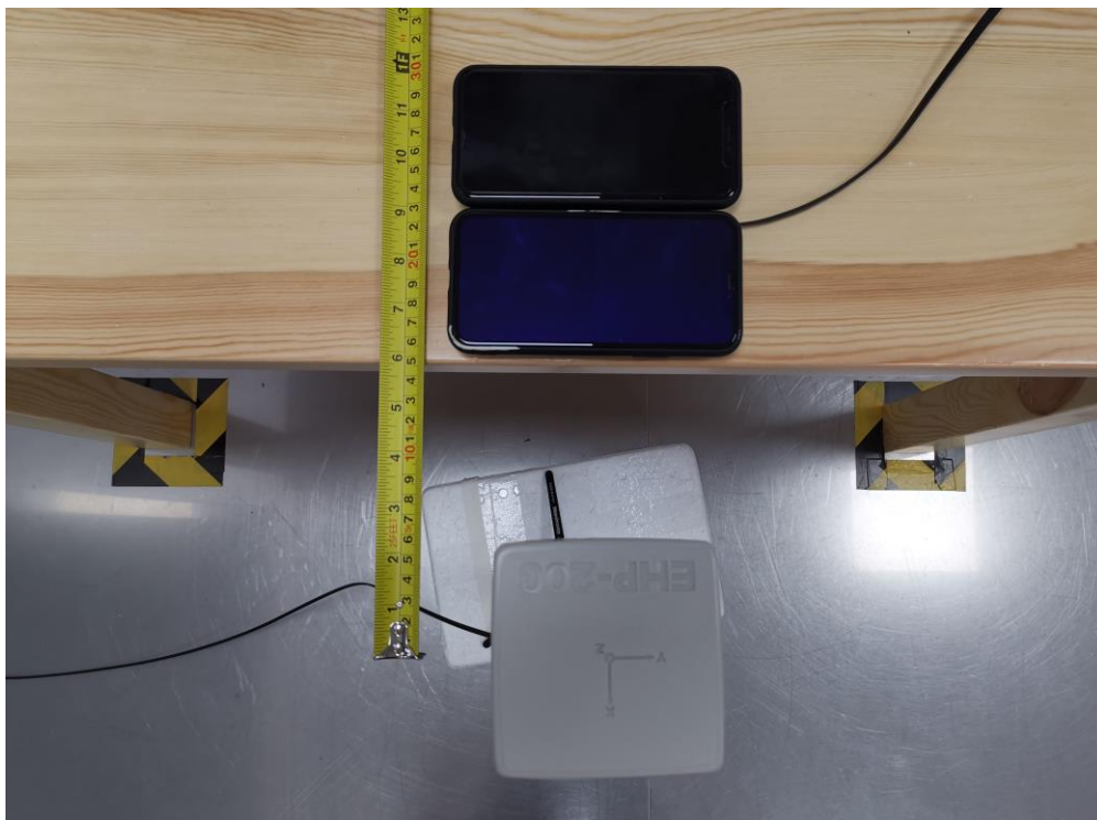
Test setup of D side with Coil 1 + Coil 2
