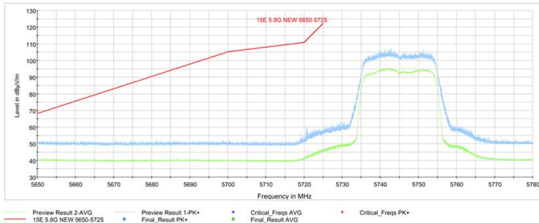
Fig. 28 Band Edges (802.11ax-HT20 Ch149, 5745MHz)
