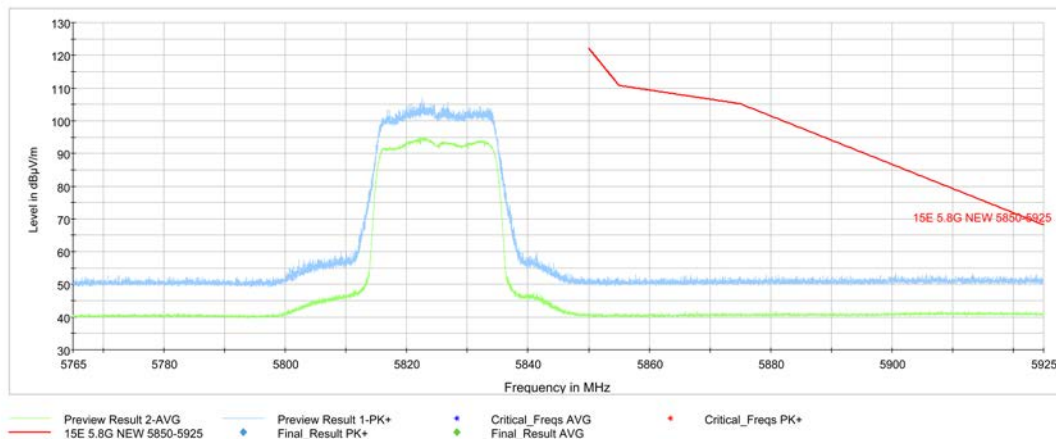
Fig. 29 Band Edges (802.11ax-HT20 Ch165, 5825MHz)
