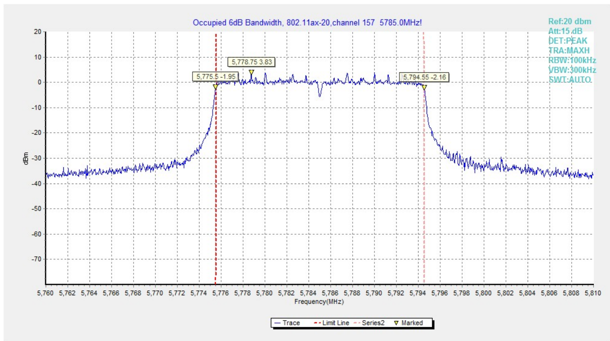
Fig. 5 Occupied 6dB Bandwidth (802.11ax-HE20, Ch 157)
