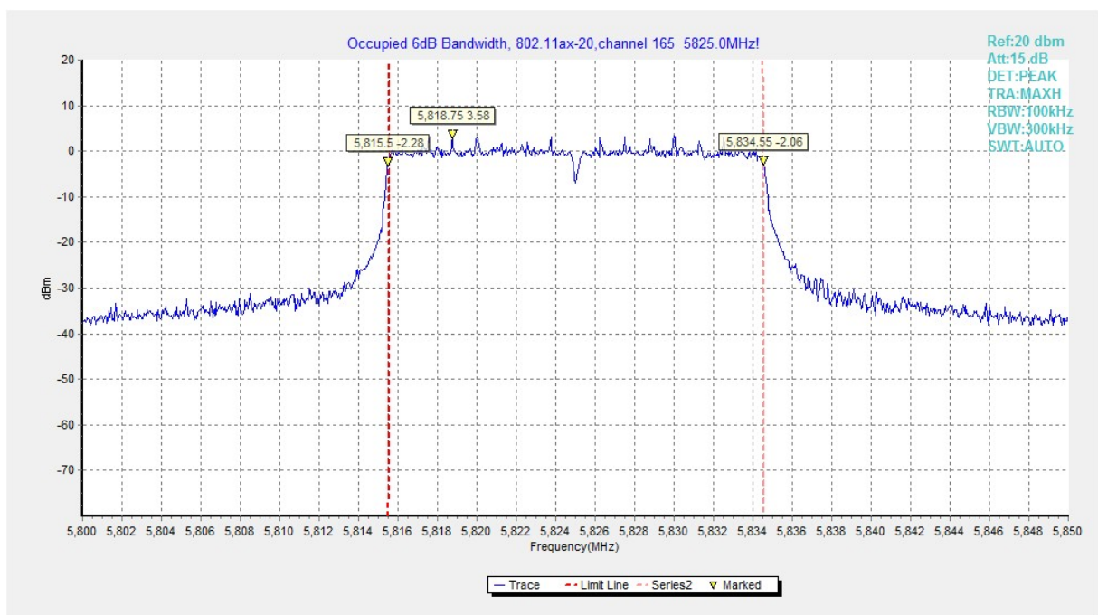
Fig. 6 Occupied 6dB Bandwidth (802.11ax-HE20, Ch 165)
