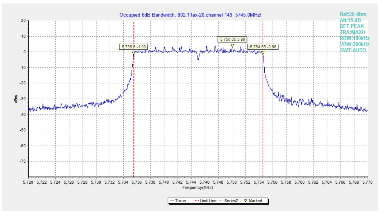
Fig. 4 Occupied 6dB Bandwidth (802.11ax-HE20, Ch 149)
