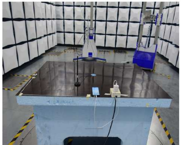
Radiated Disturbance Emissions (below 1GHz)
