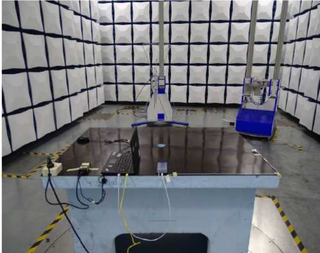
Radiated Disturbance Emissions (below 1GHz)
