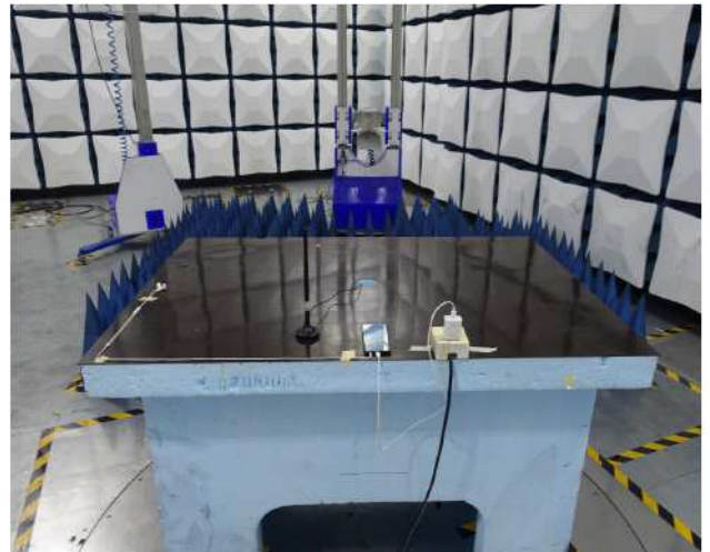
Radiated Disturbance Emissions (1GHz to 18GHz)
