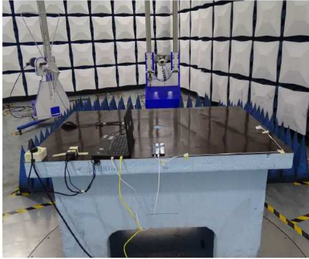
Radiated Disturbance Emissions (18GHz to 40GHz)
