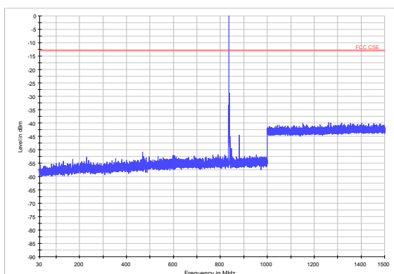
NB-IOT Band 5 CH-High 15KHz 30MHz-1.5GHz
