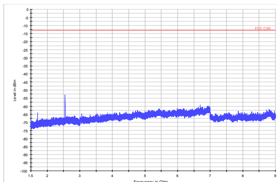
NB-IOT Band 5 CH-High 15KHz 1.5GHz-9GHz
