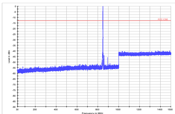
NB-IOT Band 5 CH-High 15KHz 30MHz-1.5GHz
