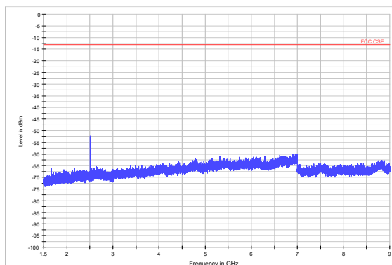
NB-IOT Band 5 CH-Middle 15KHz 1.5GHz-9GHz
