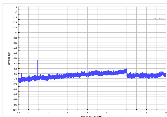
NB-IOT Band 5 CH-Low 15KHz 1.5GHz-9GHz
