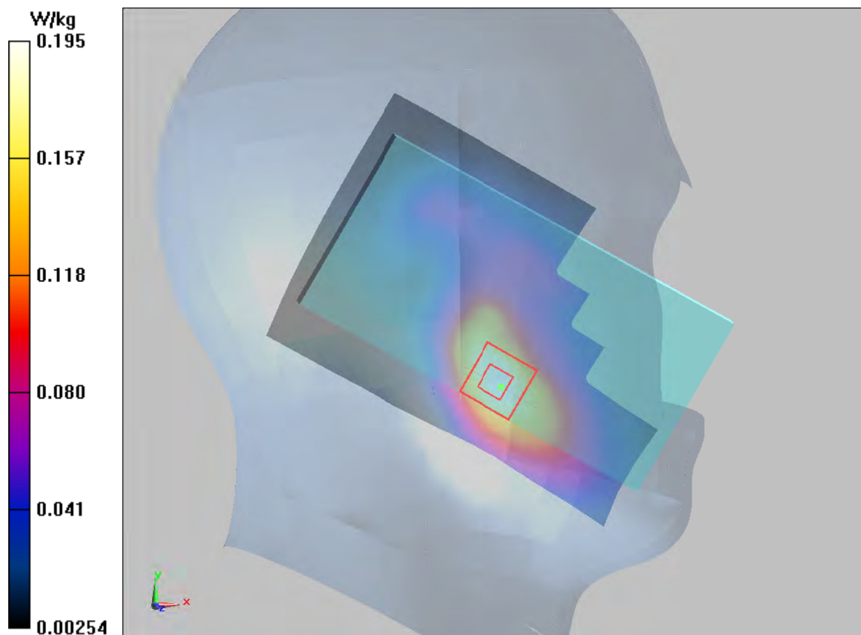
Plot 17 GSM 1900 Back Side Middle (Distance 15mm)
