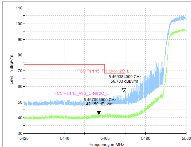
Fig. 61 Band Edges (802.11a, CH100 5500MHz)
