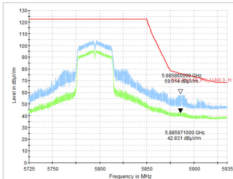
Fig. 70 Band Edges (802.11n-HT40, CH159 5795MHz)
