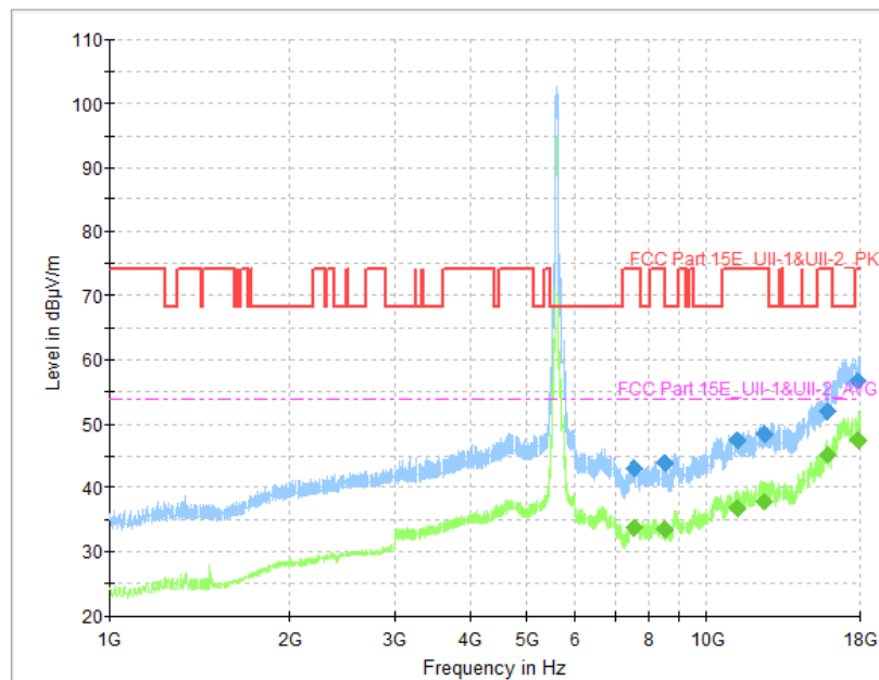
Fig. 101 Transmitter Spurious Emission (802.11ac-VHT80, CH155 5775MHz, 1 GHz-18 GHz)
