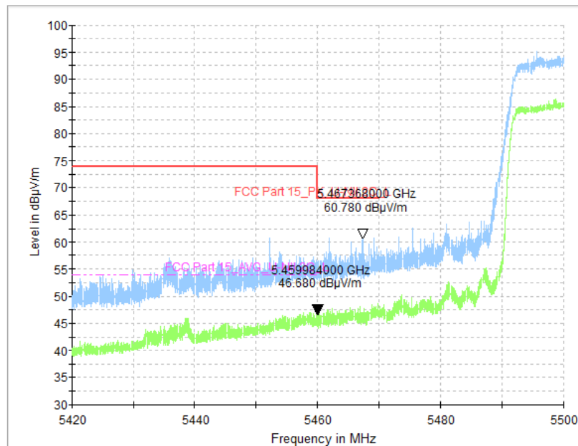
Fig. 73 Band Edges (802.11ac-VHT80, CH106 5530MHz)
