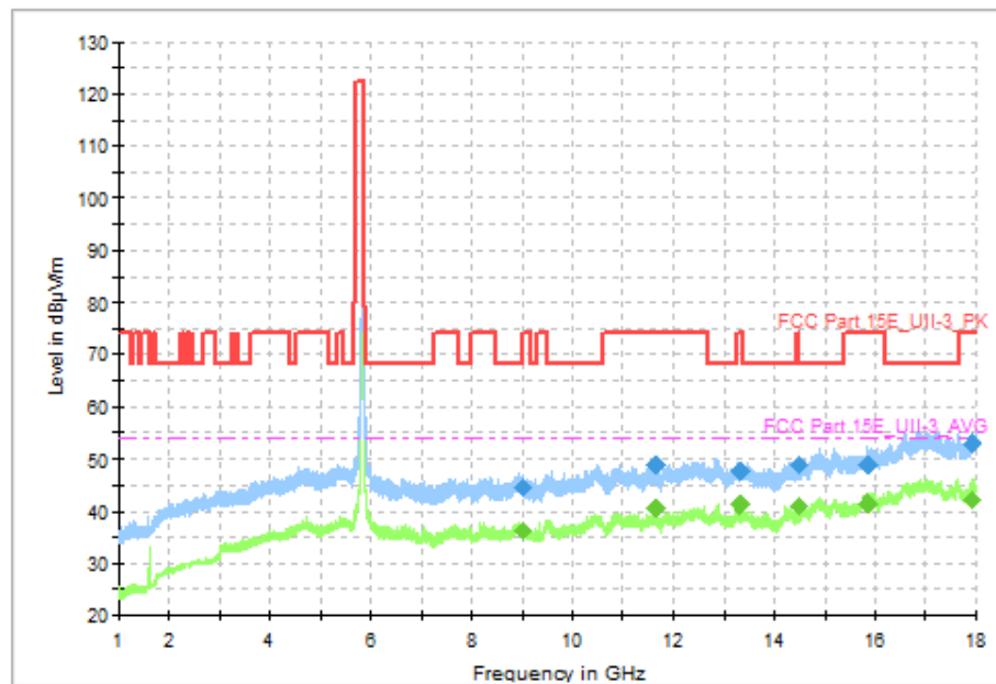
Fig. 87 Transmitter Spurious Emission (802.11a, CH165 5825MHz, 1 GHz-18 GHz)
