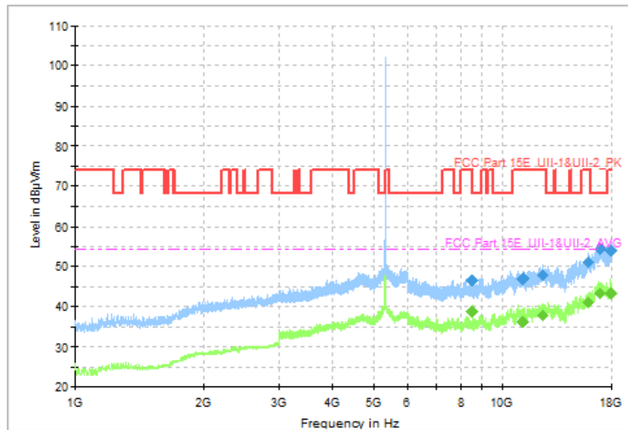
Fig. 81 Transmitter Spurious Emission (802.11a, CH64 5320MHz, 1 GHz-18 GHz)
