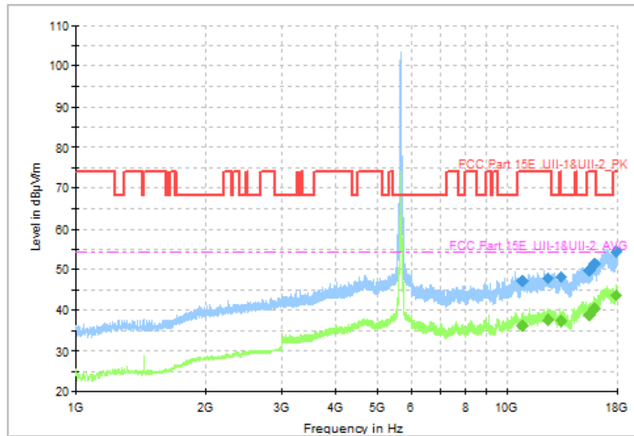
Fig. 94 Transmitter Spurious Emission (802.11n-HT40, CH134 5670MHz, 1 GHz-18 GHz)
