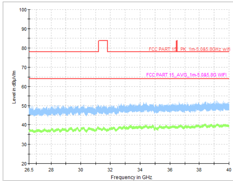
Fig. 104 Transmitter Spurious Emission (All channel, 26.5GHz~40GHz)
