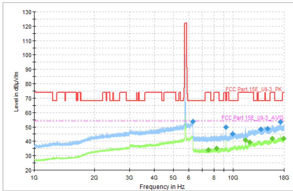
Fig. 95 Transmitter Spurious Emission (802.11n-HT40, CH151 5755MHz, 1 GHz-18 GHz)
