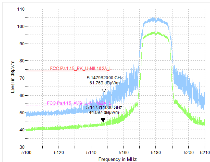
Fig. 59 Band Edges (802.11a, CH36 5180MHz)
