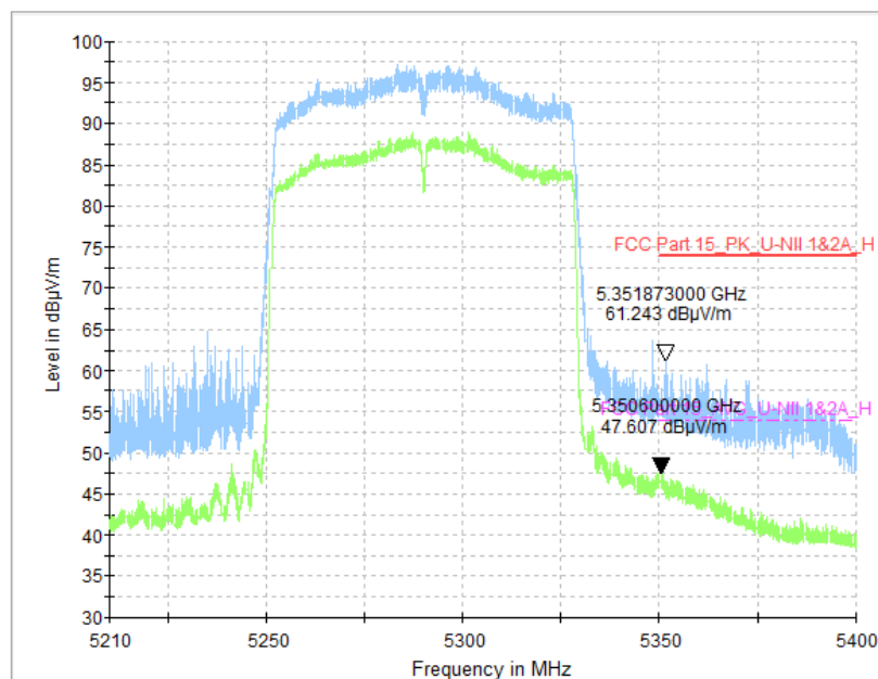
Fig. 72 Band Edges (802.11ac-VHT80, CH58 5290MHz)
