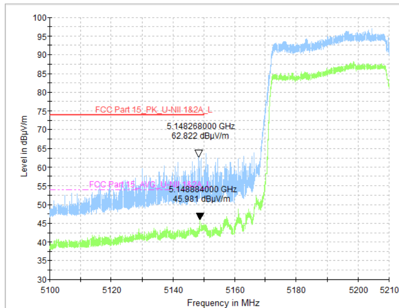
Fig. 71 Band Edges (802.11ac-VHT80, CH42 5210MHz)
