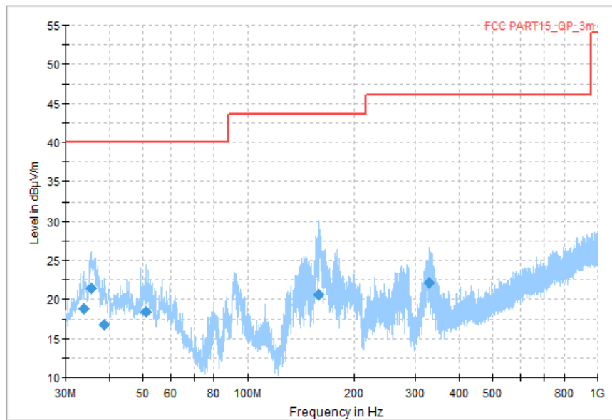
Fig. 102 Transmitter Spurious Emission (All channel, 30MHz~1GHz)
