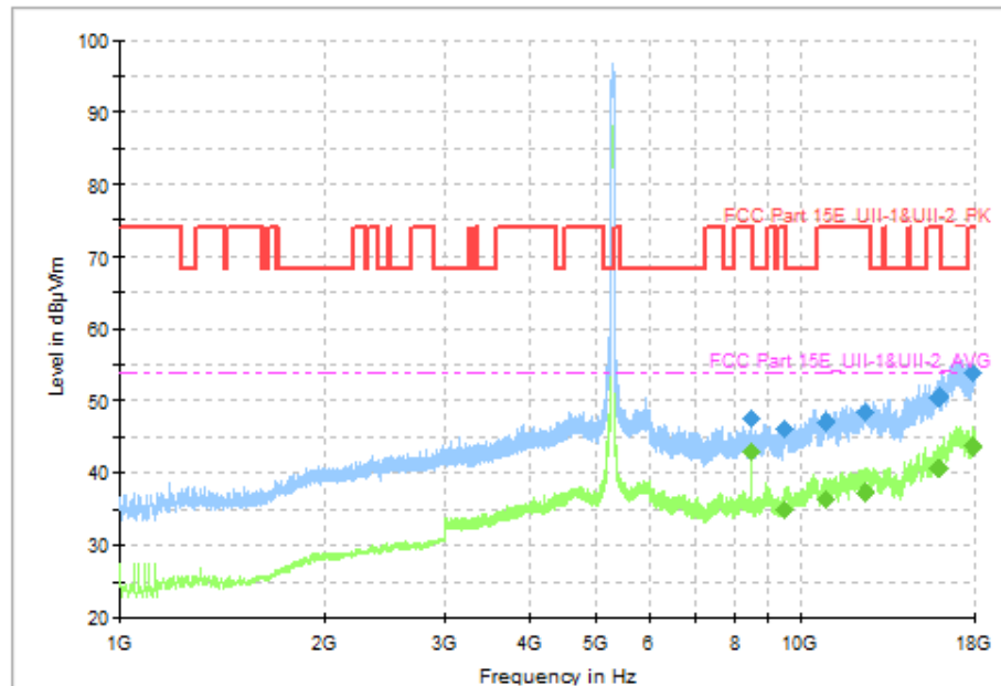
Fig. 98 Transmitter Spurious Emission (802.11ac-VHT80, CH58 5290MHz, 1 GHz-18 GHz)
