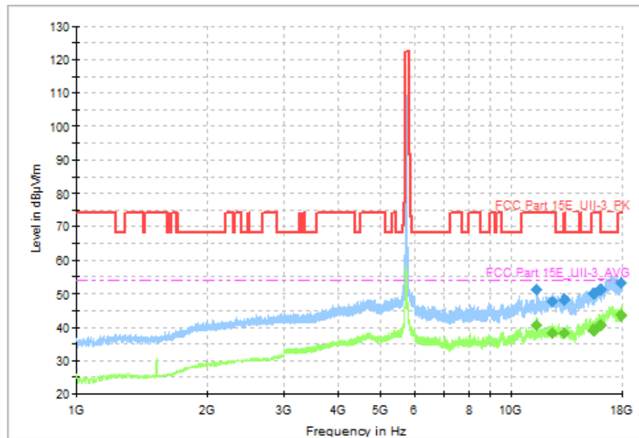
Fig. 85 Transmitter Spurious Emission (802.11a, CH149 5745MHz, 1 GHz-18 GHz)
