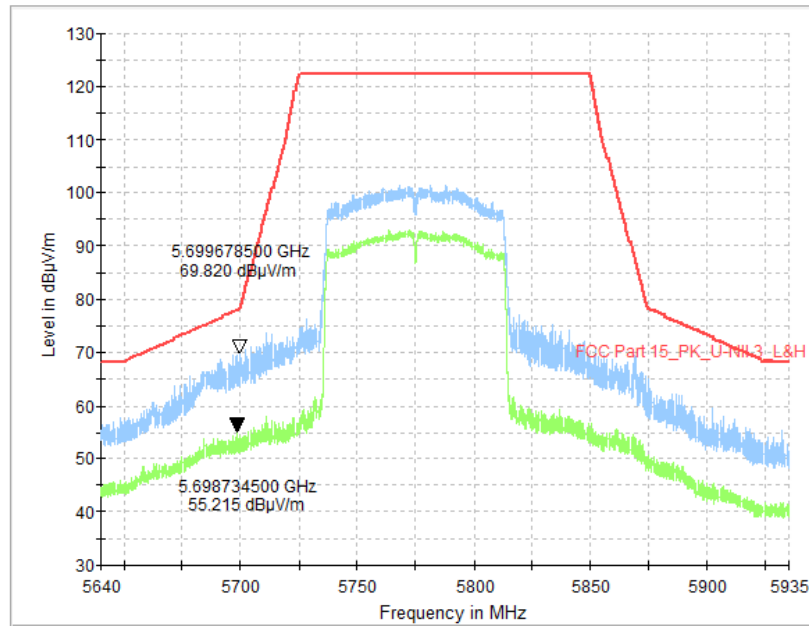
Fig. 75 Band Edges (802.11ac-VHT80, CH155 5775MHz)
