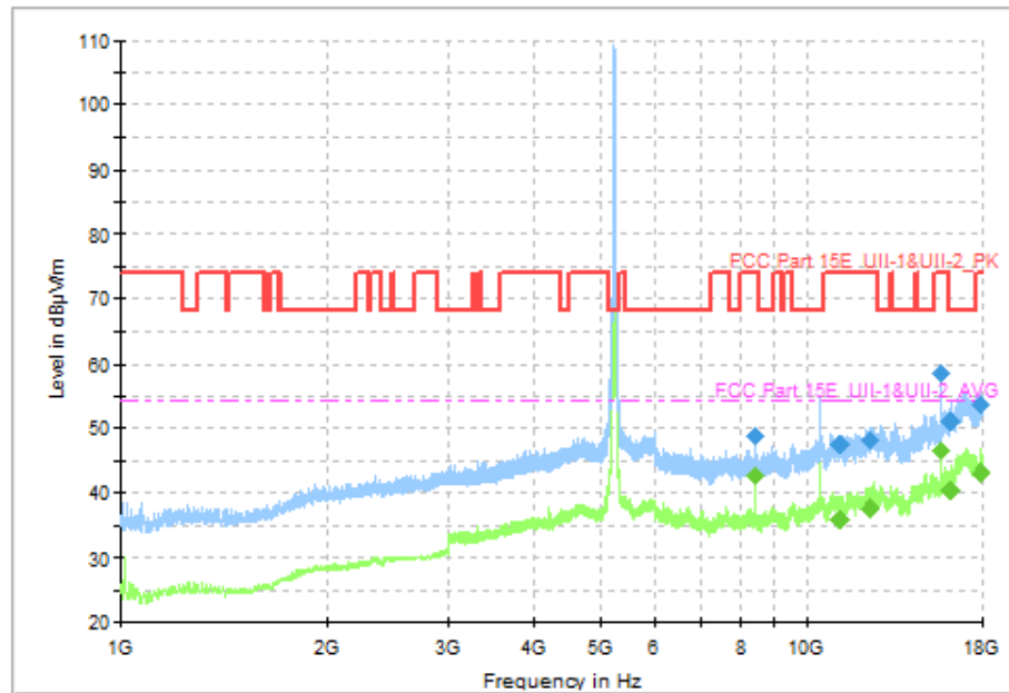
Fig. 78 Transmitter Spurious Emission (802.11a, CH48 5240MHz, 1 GHz-18 GHz)
