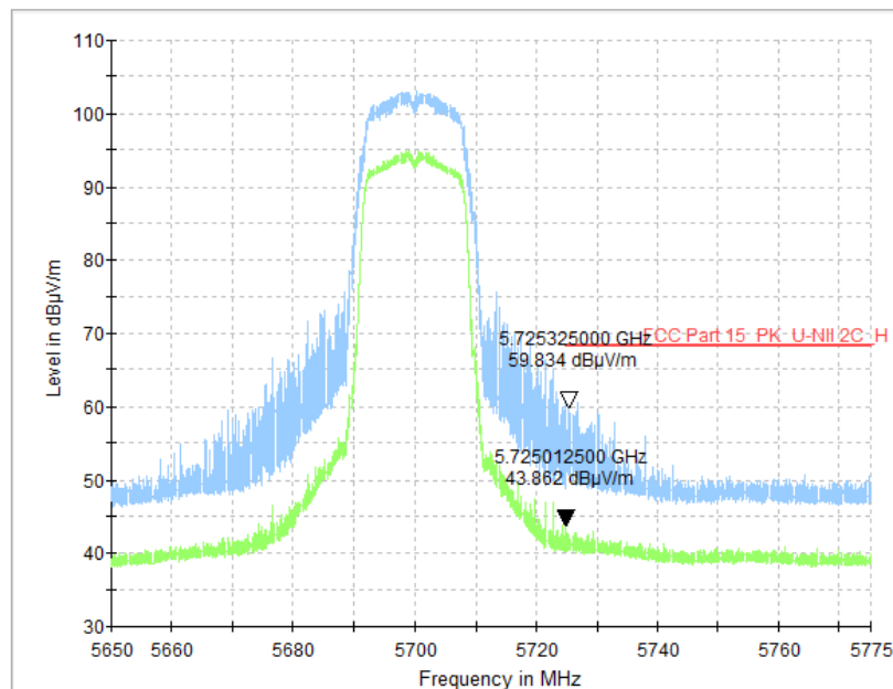
Fig. 62 Band Edges (802.11a, CH140 5700MHz)
