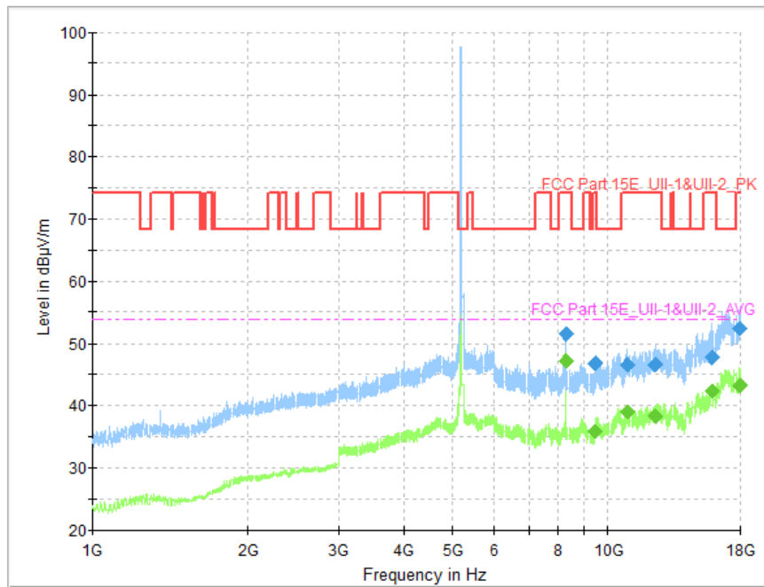
Fig. 88 Transmitter Spurious Emission (802.11n-HT40, CH38 5190MHz, 1 GHz-18 GHz)
