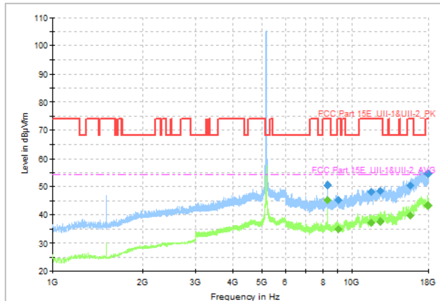
Fig. 76 Transmitter Spurious Emission (802.11a, CH36 5180MHz, 1 GHz-18 GHz)
