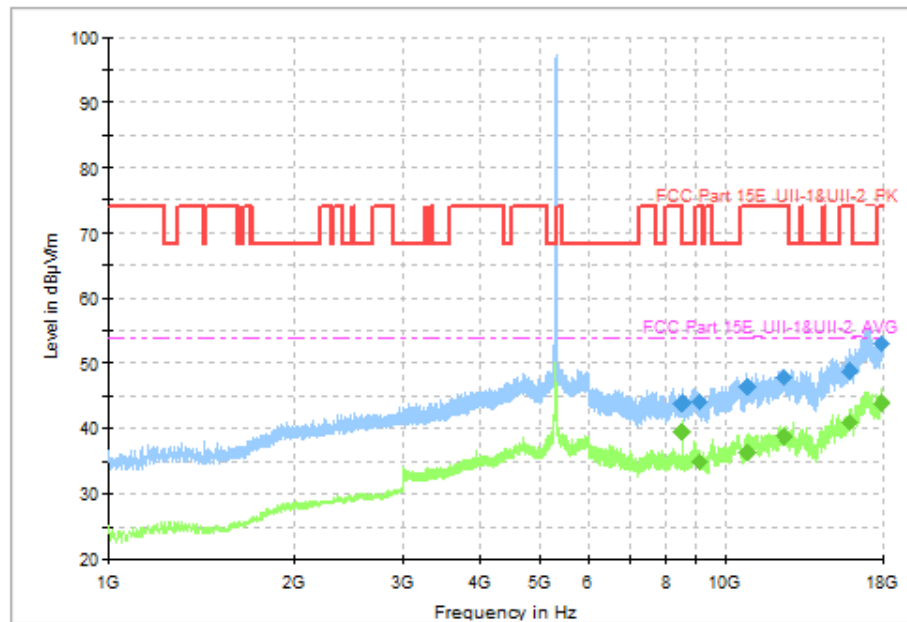
Fig. 91 Transmitter Spurious Emission (802.11n-HT40, CH62 5310MHz, 1 GHz-18 GHz)
