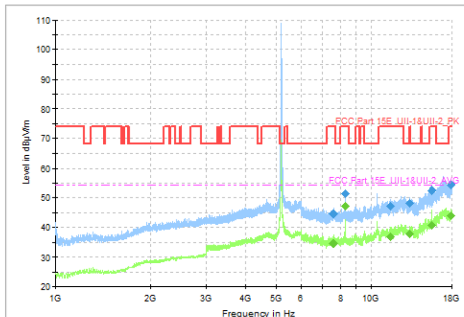
Fig. 77 Transmitter Spurious Emission (802.11a, CH40 5200MHz, 1 GHz-18 GHz)
