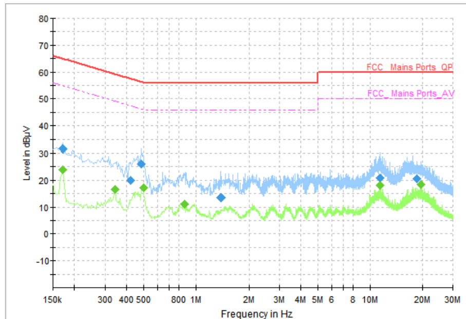
Fig. 107 AC Power line Conducted Emission (Idle)
