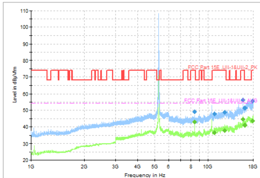
Fig. 79 Transmitter Spurious Emission (802.11a, CH52 5260MHz, 1 GHz-18 GHz)
