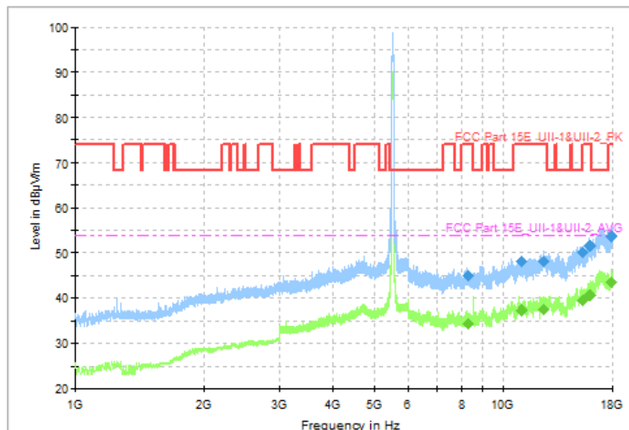
Fig. 99 Transmitter Spurious Emission (802.11ac-VHT80, CH106 5530MHz, 1 GHz-18 GHz)
