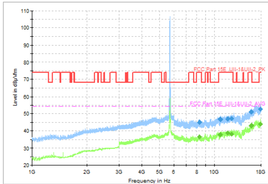
Fig. 84 Transmitter Spurious Emission (802.11a, CH140 5700MHz, 1 GHz-18 GHz)
