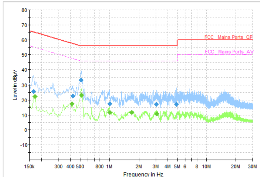
Fig. 106 AC Power line Conducted Emission (Traffic)
