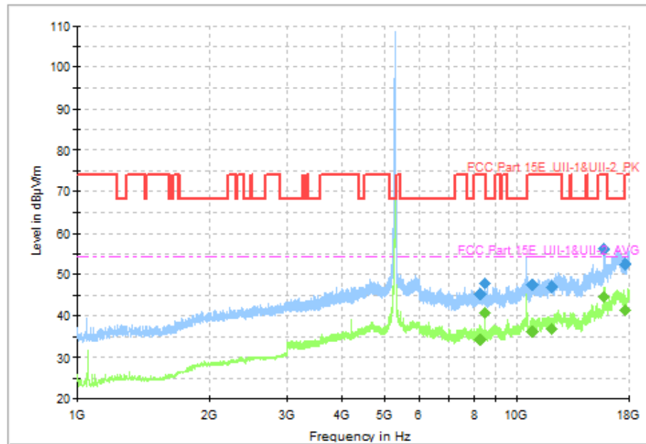
Fig. 80 Transmitter Spurious Emission (802.11a, CH56 5280MHz, 1 GHz-18 GHz)
