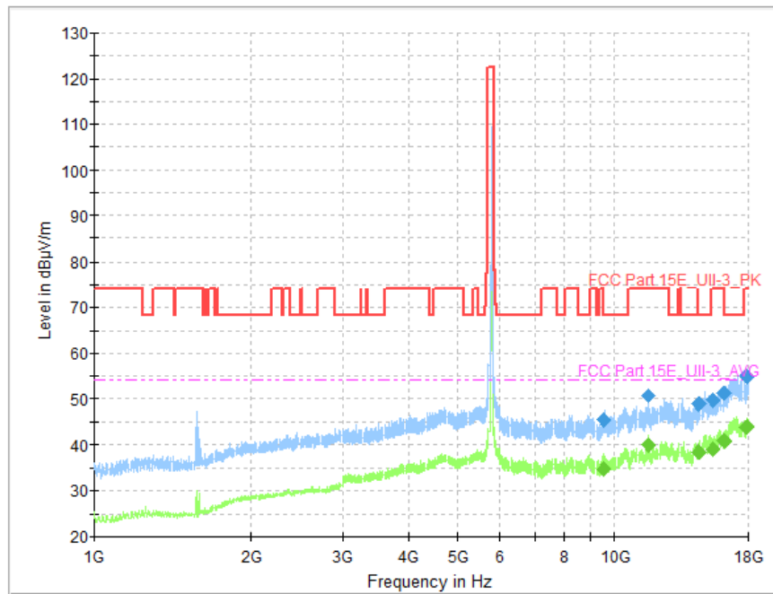
Fig. 86 Transmitter Spurious Emission (802.11a, CH157 5785MHz, 1 GHz-18 GHz)
