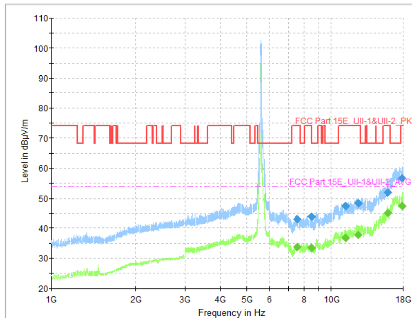
Fig. 100 Transmitter Spurious Emission (802.11ac-VHT80, CH122 5610MHz, 1 GHz-18 GHz)
