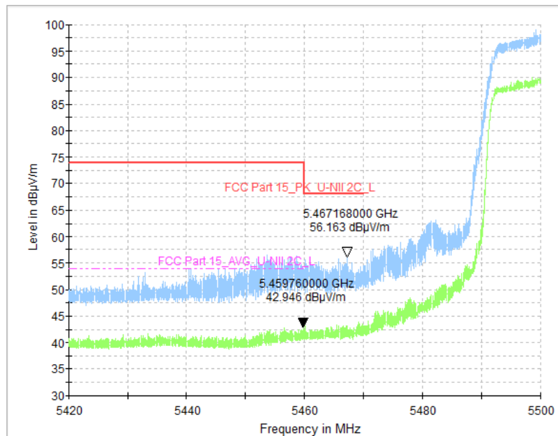
Fig. 67 Band Edges (802.11n-HT40, CH102 5510MHz)
