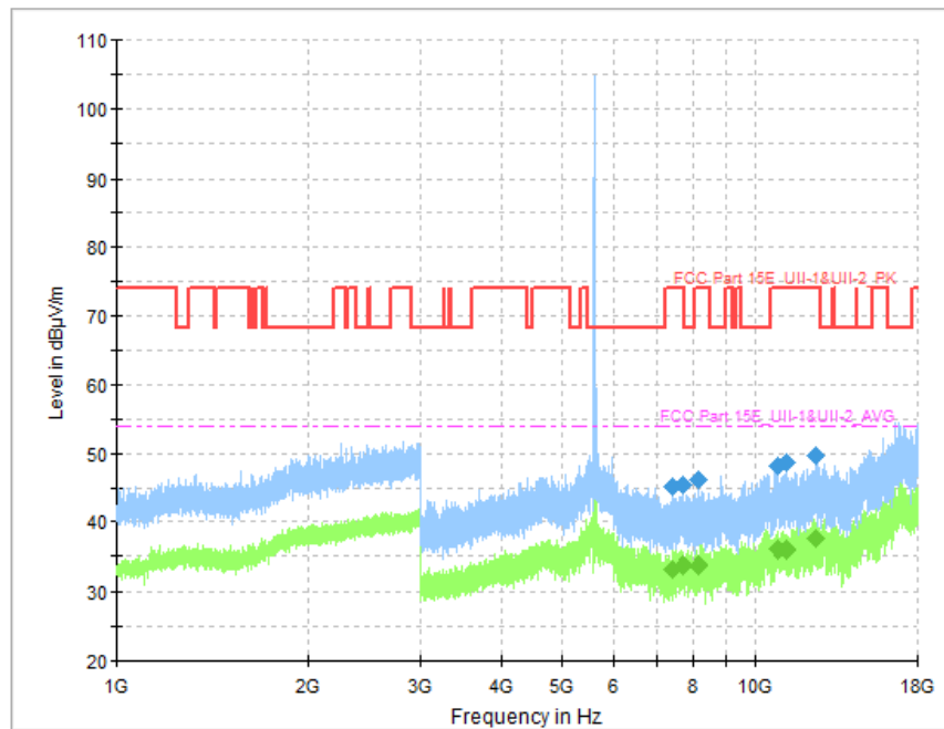
Fig. 83 Transmitter Spurious Emission (802.11a, CH120 5600MHz, 1 GHz-18 GHz)
