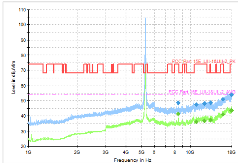
Fig. 90 Transmitter Spurious Emission (802.11n-HT40, CH54 5270MHz, 1 GHz-18 GHz)
