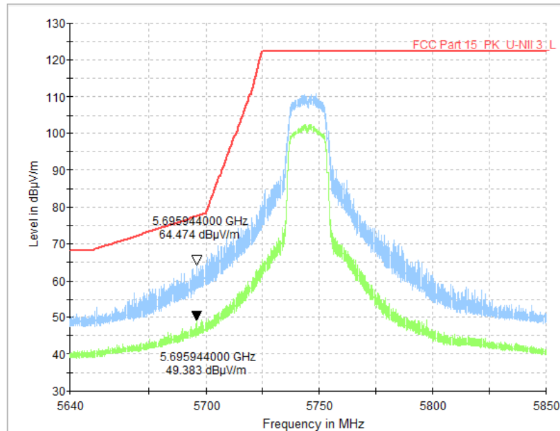
Fig. 63 Band Edges (802.11a, CH149 5745MHz)
