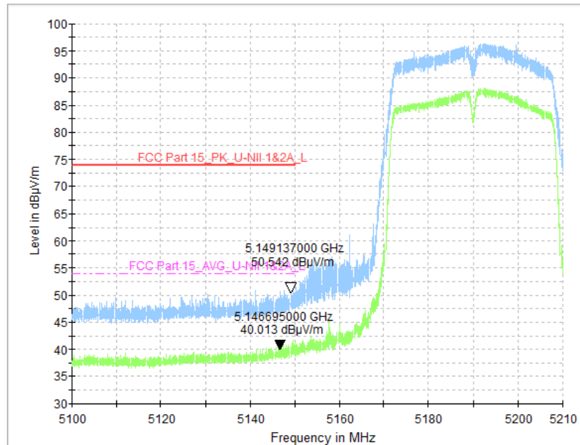
Fig. 65 Band Edges (802.11n-HT40, CH38 5190MHz)
