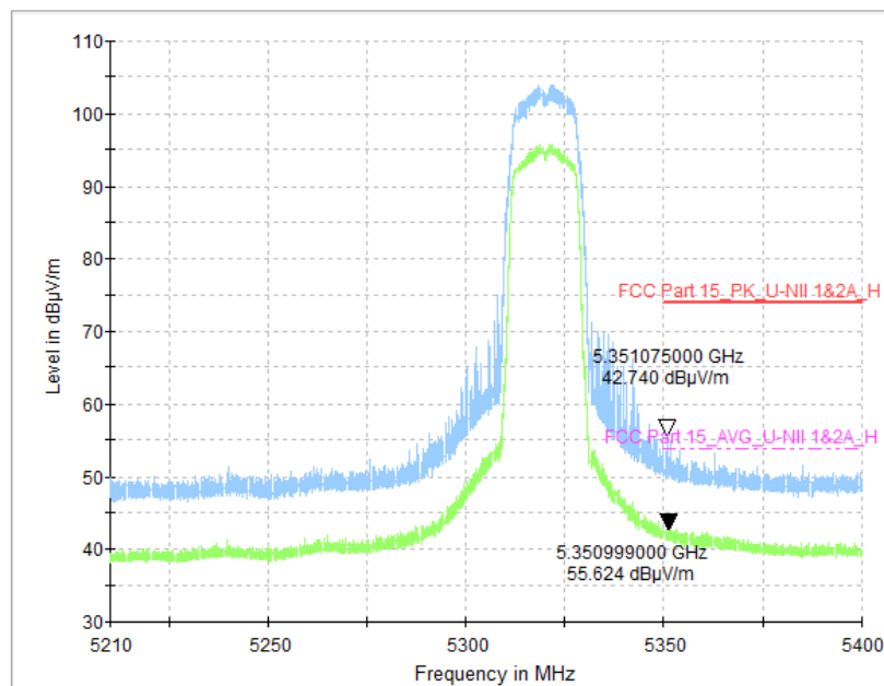
Fig. 60 Band Edges (802.11a, CH64 5320MHz)
