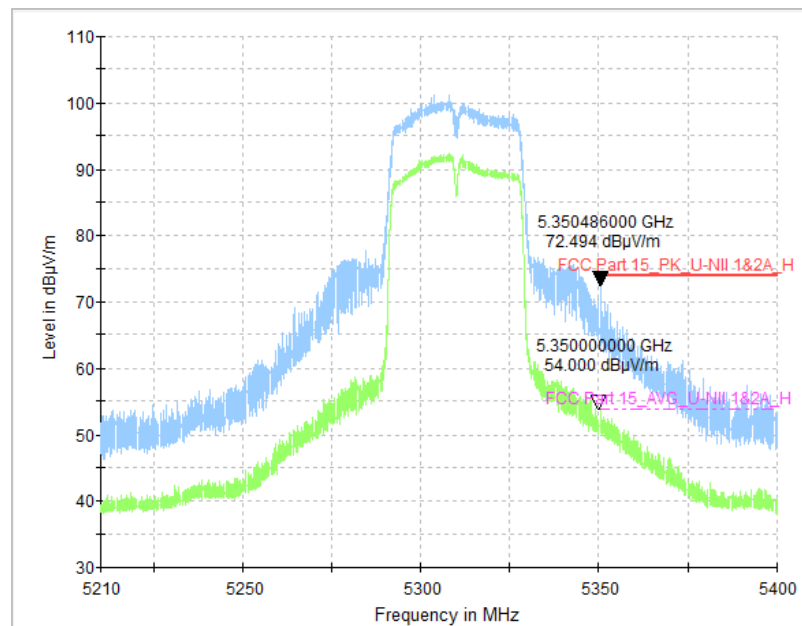
Fig. 66 Band Edges (802.11n-HT40, CH62 5310MHz)
