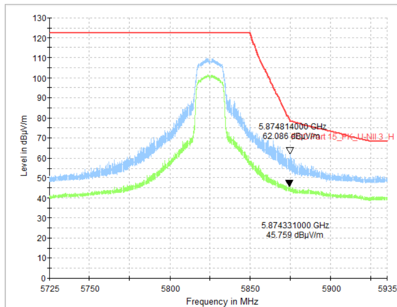
Fig. 64 Band Edges (802.11a, CH165 5825MHz)
