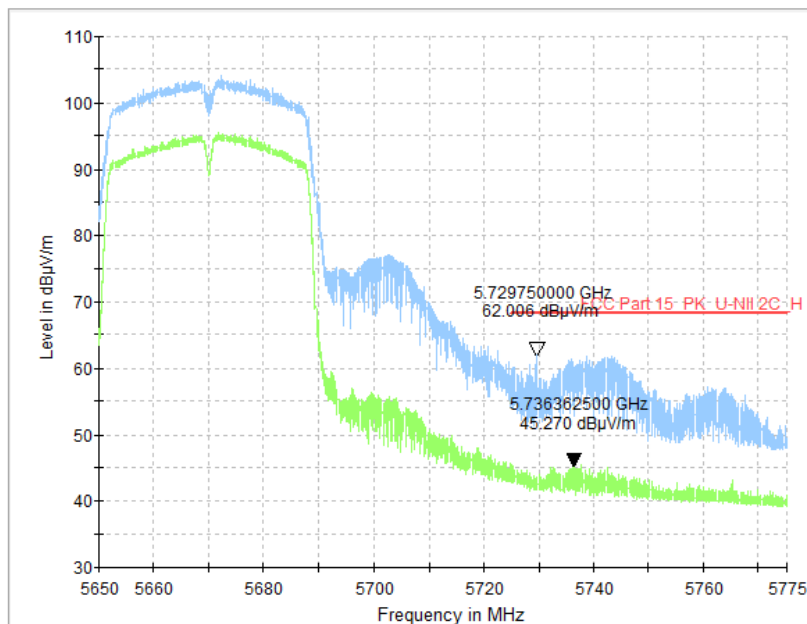
Fig. 68 Band Edges (802.11n-HT40, CH134 5670MHz)
