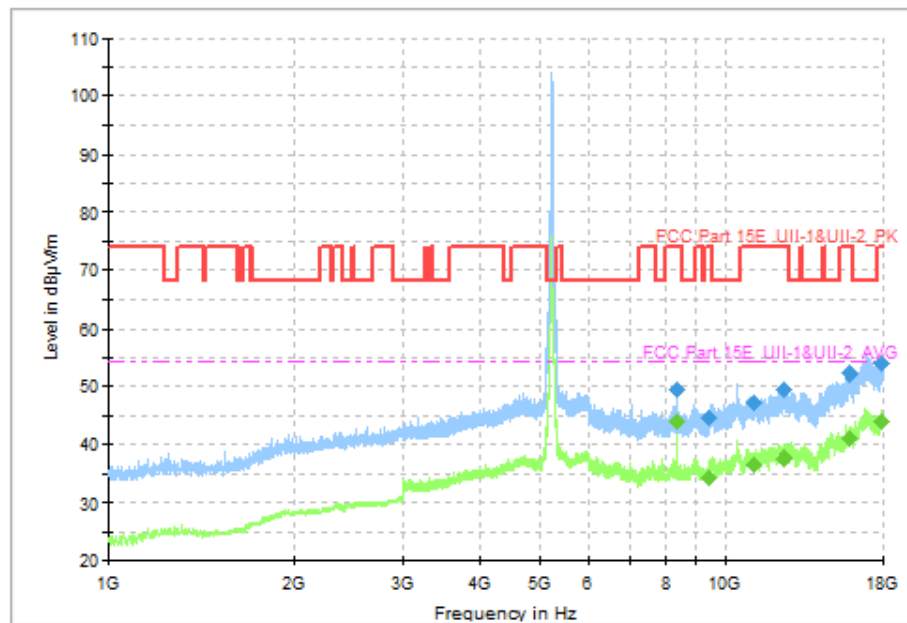
Fig. 89 Transmitter Spurious Emission (802.11n-HT40, CH46 5230MHz, 1 GHz-18 GHz)
