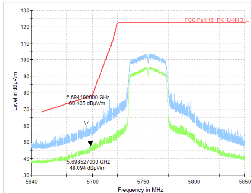
Fig. 69 Band Edges (802.11n-HT40, CH151 5755MHz)
