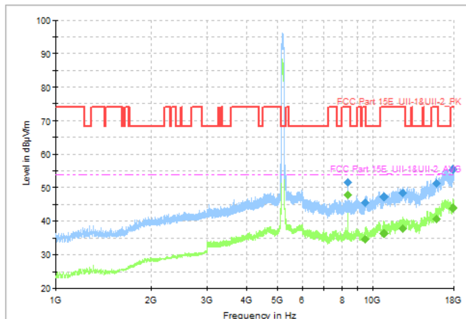
Fig. 97 Transmitter Spurious Emission (802.11ac-VHT80, CH42 5210MHz, 1 GHz-18 GHz)
