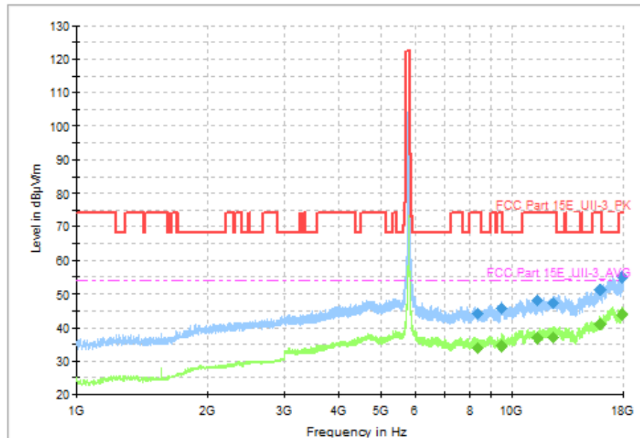
Fig. 96 Transmitter Spurious Emission (802.11n-HT40, CH159 5795MHz, 1 GHz-18 GHz)
