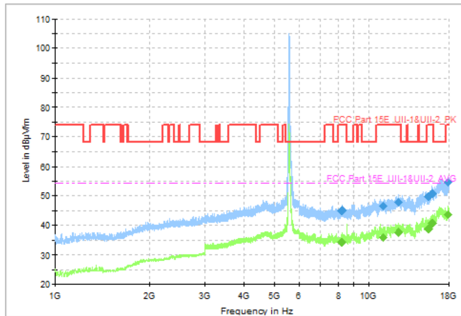
Fig. 93 Transmitter Spurious Emission (802.11n-HT40, CH118 5580MHz, 1 GHz-18 GHz)
