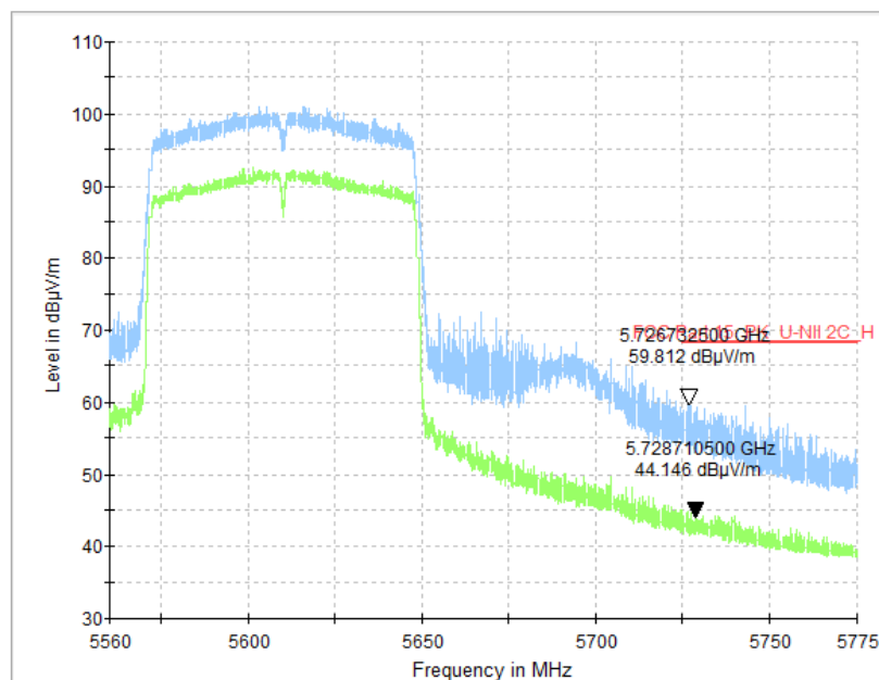
Fig. 74 Band Edges (802.11ac-VHT80, CH122 5610MHz)
