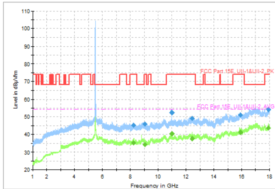
Fig. 82 Transmitter Spurious Emission (802.11a, CH100 5500MHz, 1 GHz-18 GHz)
