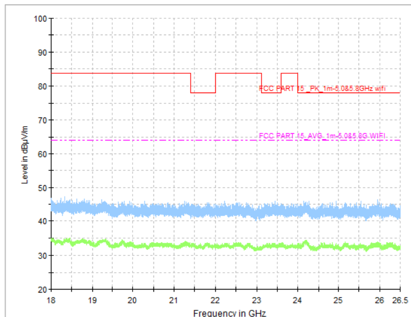
Fig. 103 Transmitter Spurious Emission (All channel, 18GHz~26.5GHz)
