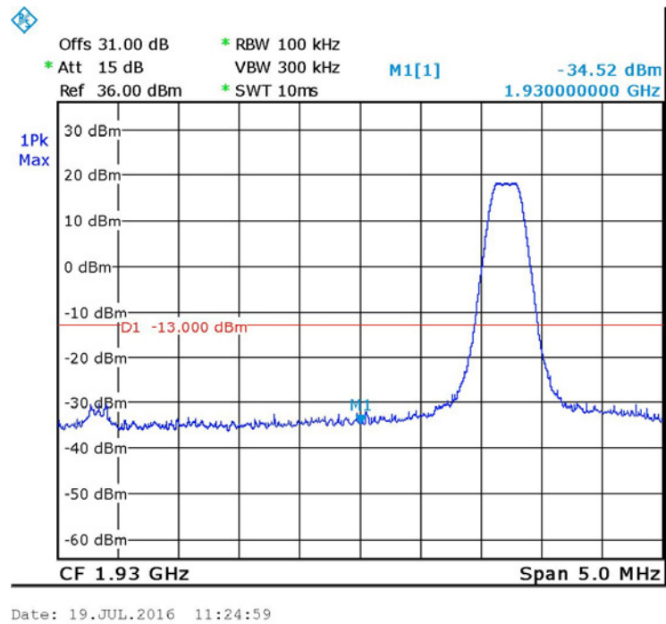
Figure 54. — GSM - 1931.2 MHz
