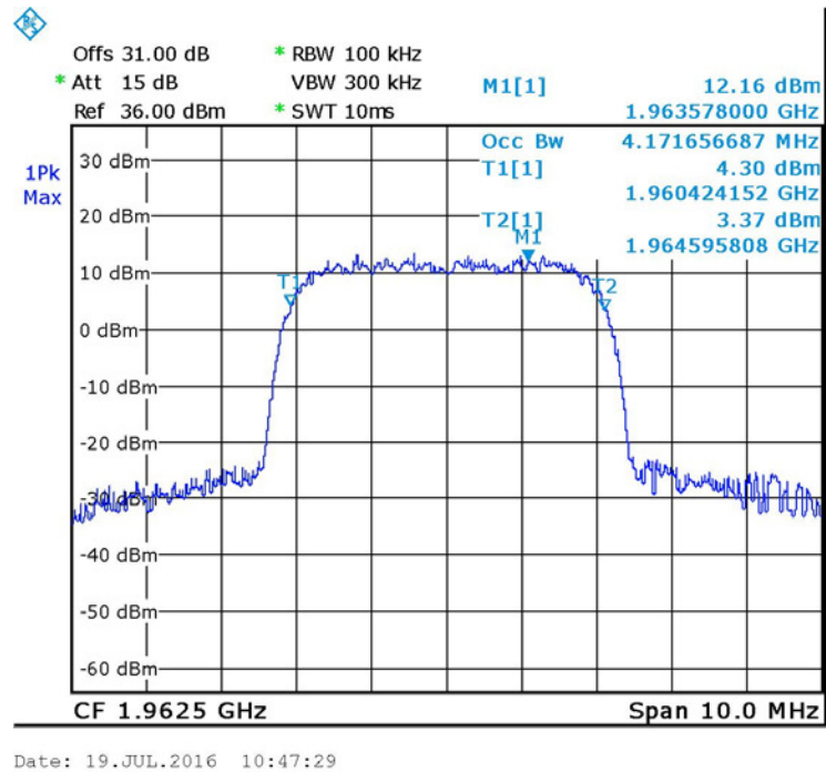
Figure 37. — W-CDMA - Output 1962.5 MHz
