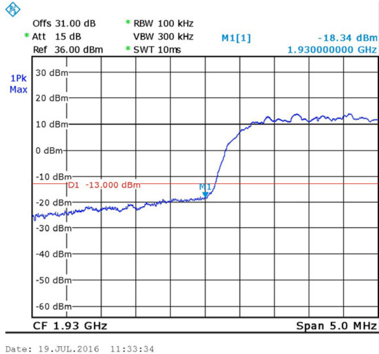
Figure 56. — W-CDMA - 1932.5 MHz
