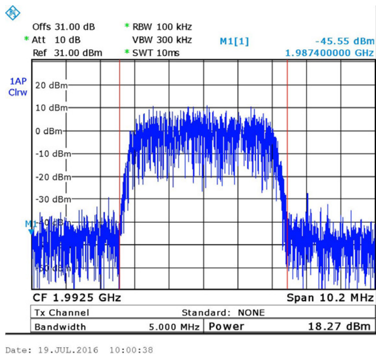
Figure 19. — W-CDMA - 1992.5 MHz
