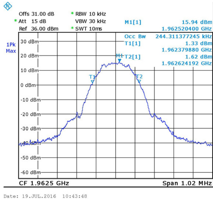
Figure 31. — GSM - Output 1962.5 MHz
