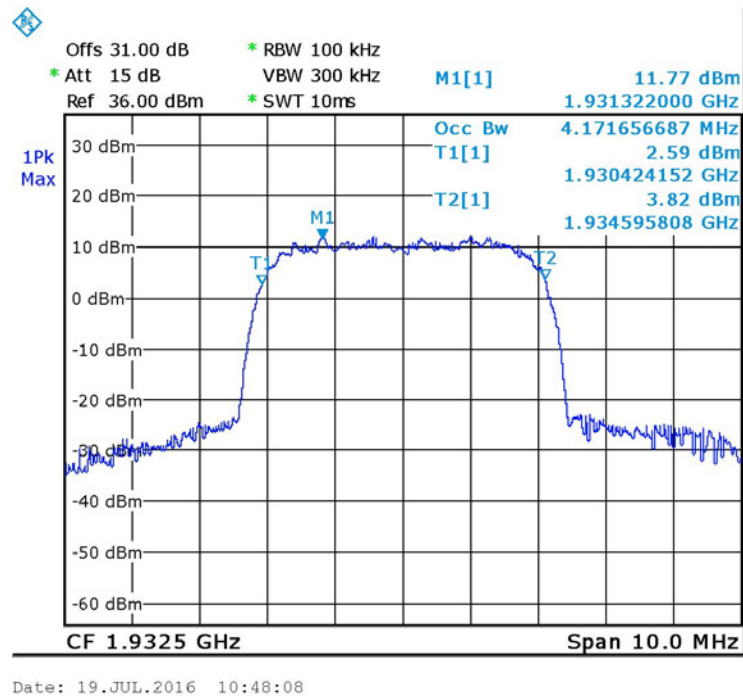
Figure 35. — W-CDMA - Output 1932.5 MHz
