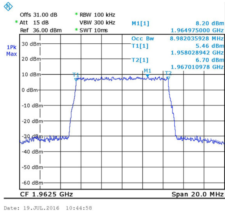
Figure 25. — LTE 64QAM Output 1962.5 MHz
