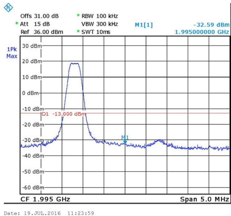
Figure 55. — GSM - 1993.8 MHz
