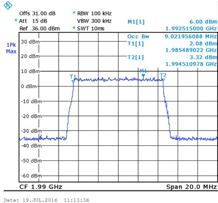
Figure 26. — LTE 64QAM Input 1990.0 MHz
