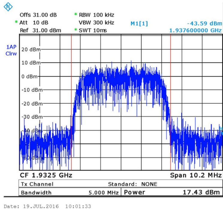
Figure 17. — W-CDMA - 1932.5 MHz
