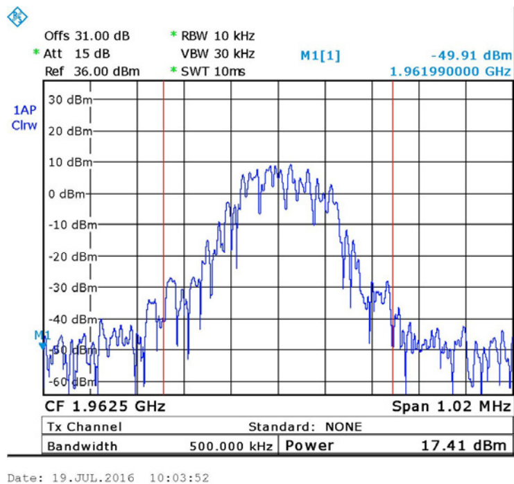
Figure 15. — GSM -1962.5 MHz
