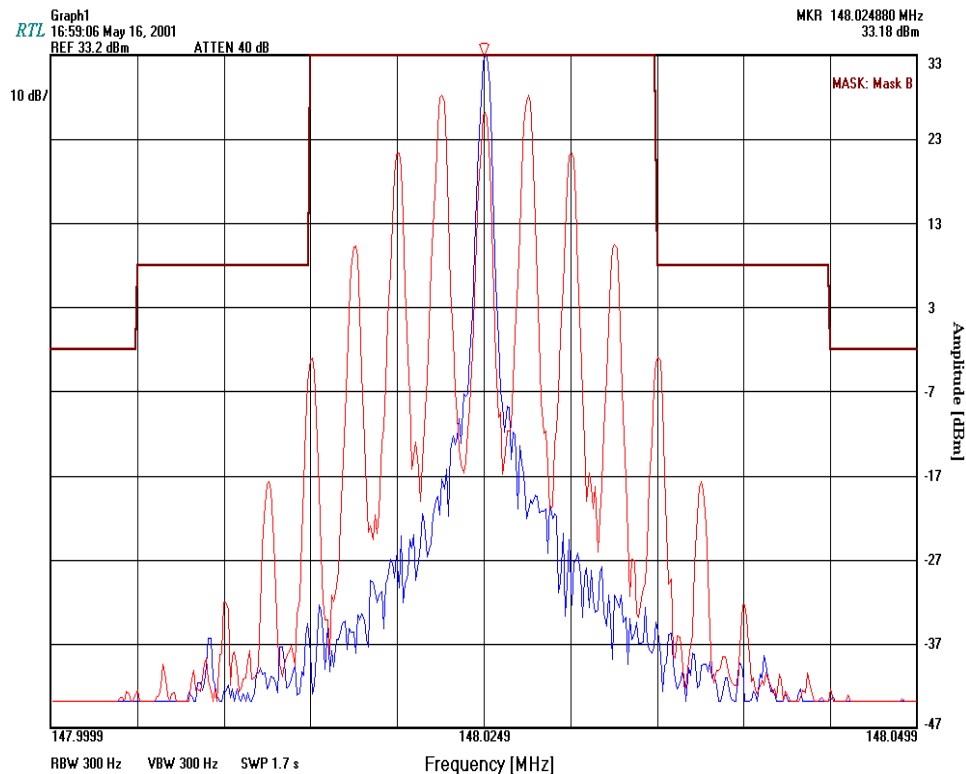
PLOT 9-1: OCCUPIED BANDWIDTH {25 KHz CHANNEL BANDWIDTH: MASK B (AUDIO MODULATION: 2,500 Hz)}
