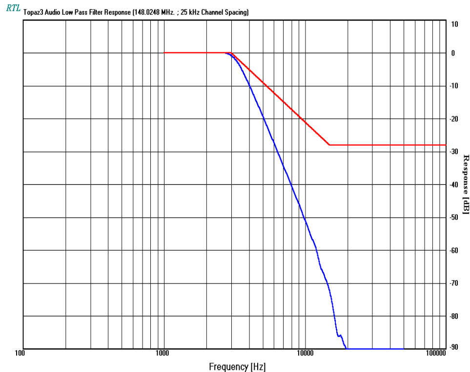
PLOT 12-1: MODULATION CHARACTERISTICS – Audio Low Pass Filter
