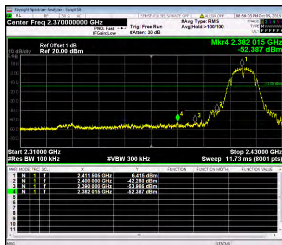
Left bandedge
