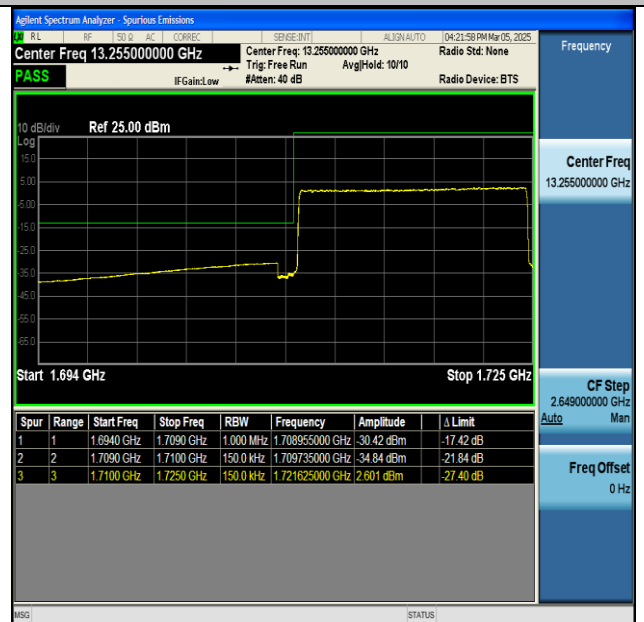
NTNV-n66-PC3-15-15-L-CP-QPSK-Outer_Full-PASS
