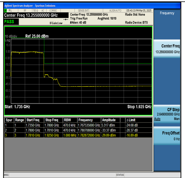
NTNV-n66-PC3-15-45-H-DFT-BPSK-Outer_Full-PASS
