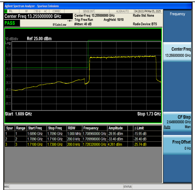
NTNV-n66-PC3-15-20-L-DFT-BPSK-Outer_Full-PASS
