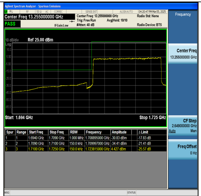
NTNV-n66-PC3-15-15-L-DFT-BPSK-Outer_Full-PASS
