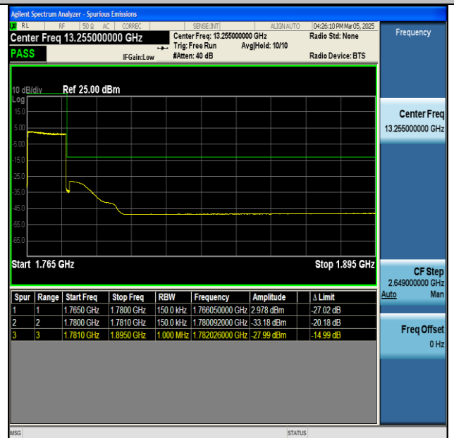
NTNV-n66-PC3-15-15-H-CP-QPSK-Outer_Full-PASS
