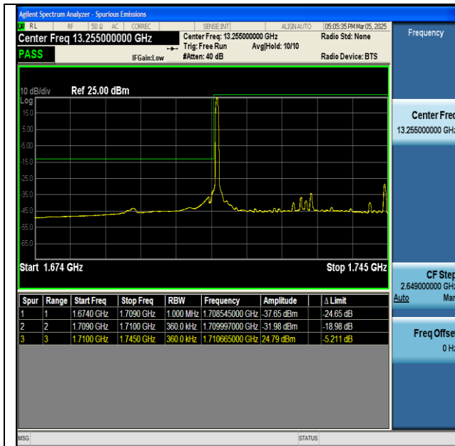
NTNV-n66-PC3-15-35-L-DFT-BPSK-Edge_1RB_Left-PASS
