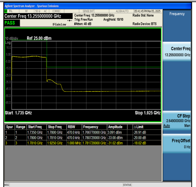
NTNV-n66-PC3-15-45-H-CP-QPSK-Outer_Full-PASS
