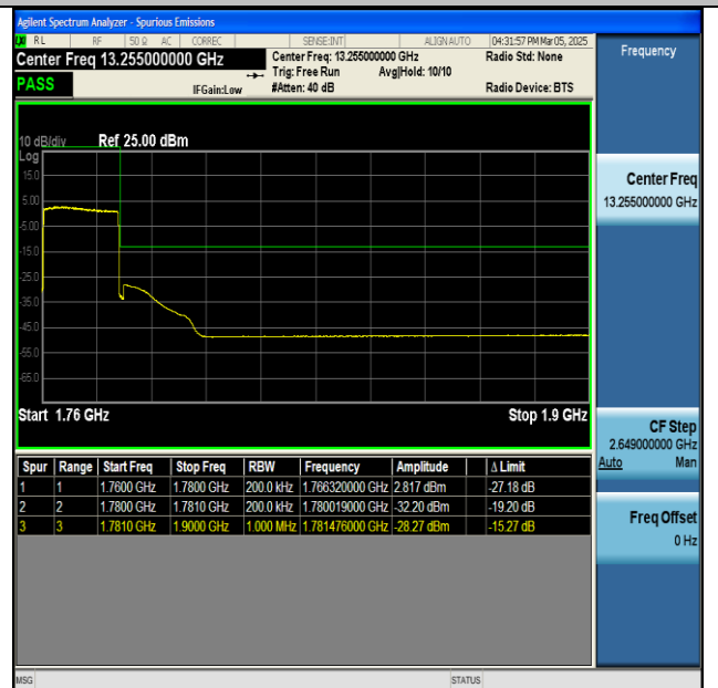
NTNV-n66-PC3-15-20-H-CP-QPSK-Outer_Full-PASS
