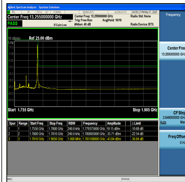
NTNV-n66-PC3-15-25-H-CP-QPSK-Edge_1RB_Right-PASS
