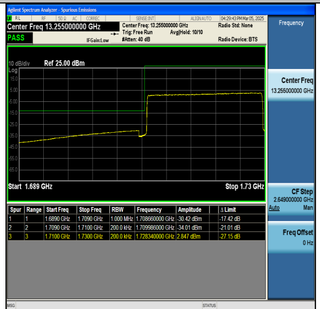
NTNV-n66-PC3-15-20-L-CP-QPSK-Outer_Full-PASS
