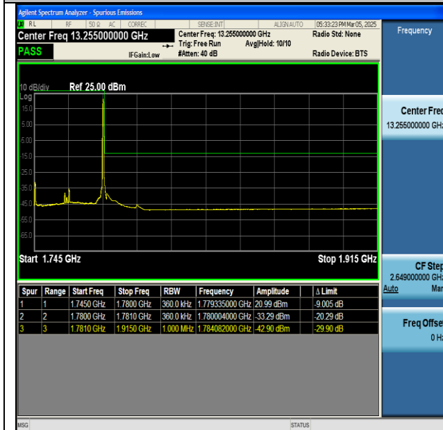
NTNV-n66-PC3-15-35-H-CP-QPSK-Edge_1RB_Right-PASS
