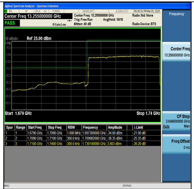
NTNV-n66-PC3-15-30-L-DFT-BPSK-Outer_Full-PASS
