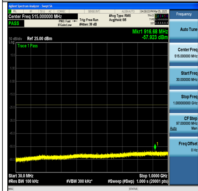
NTNV-n66-PC3-15-45-H-DFT-BPSK-Edge_1RB_Left-30-1000-PASS
