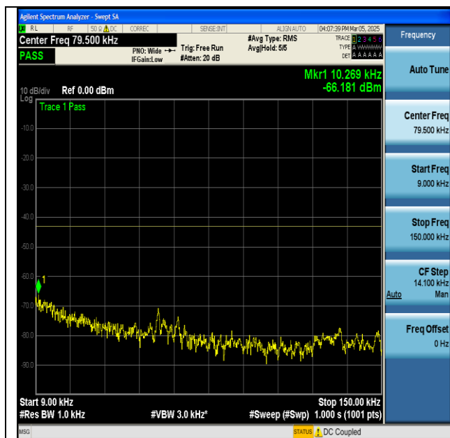
NTNV-n66-PC3-15-45-H-DFT-BPSK-Edge_1RB_Left-0.009-0.15-PASS
