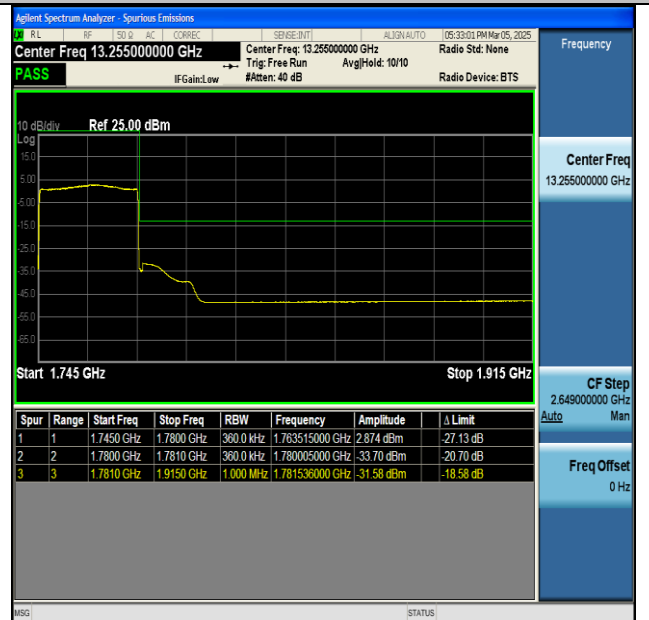
NTNV-n66-PC3-15-35-H-CP-QPSK-Outer_Full-PASS
