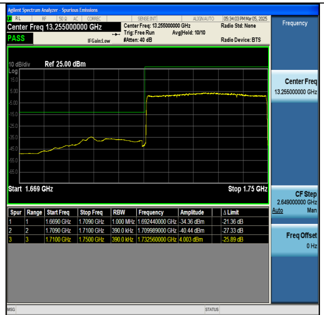
NTNV-n66-PC3-15-40-L-DFT-BPSK-Outer_Full-PASS
