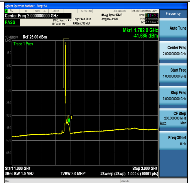
NTNV-n66-PC3-15-45-H-DFT-BPSK-Edge_1RB_Left-1000-3000-PASS
