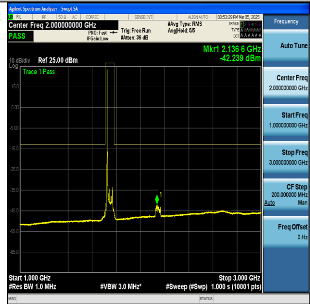
NTNV-n66-PC3-15-45-M-DFT-BPSK-Edge_1RB_Left- 1000-3000-PASS
