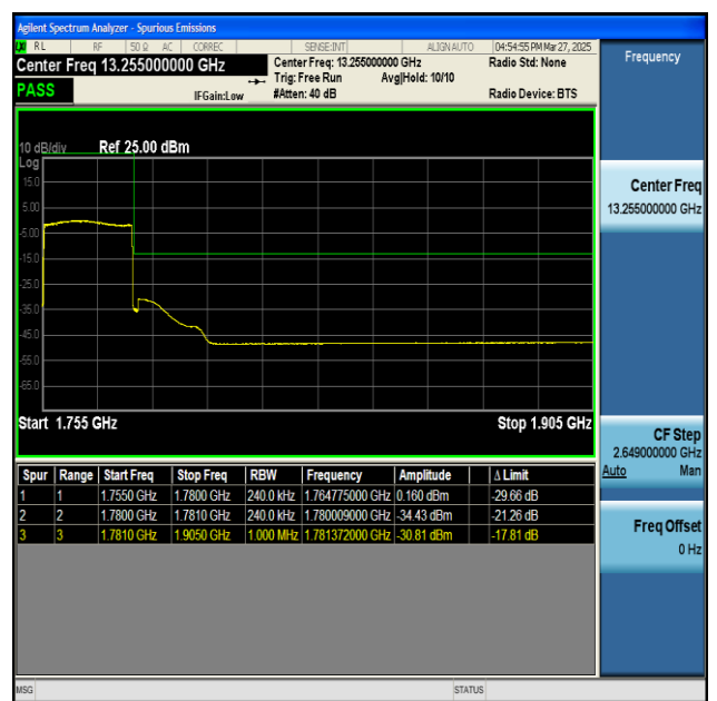
NTNV-n66-PC3-15-25-H-CP-QPSK-Outer_Full-PASS
