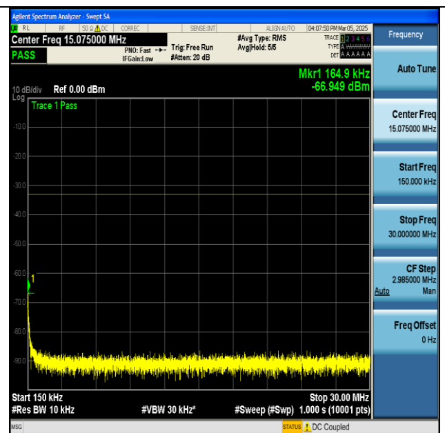
NTNV-n66-PC3-15-45-H-DFT-BPSK-Edge_1RB_Left-0.15-30-PASS
