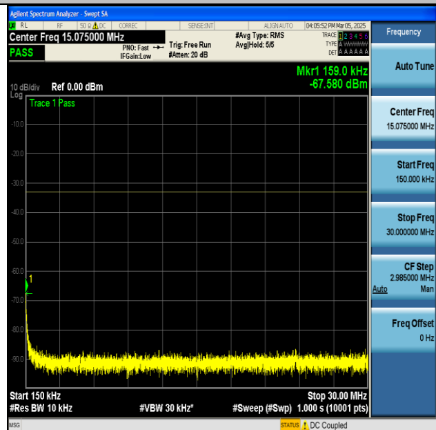
NTNV-n66-PC3-15-45-M-CP-QPSK-Edge_1RB_Left-0.15- 30-PASS
