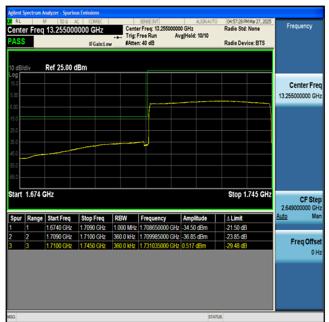
NTNV-n66-PC3-15-35-L-CP-QPSK-Outer_Full-PASS
