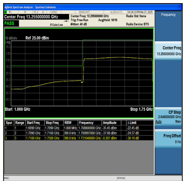
NTNV-n66-PC3-15-40-L-CP-QPSK-Outer_Full-PASS
