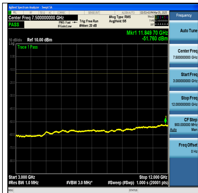
NTNV-n66-PC3-15-45-M-DFT-BPSK-Edge_1RB_Left- 3000-12000-PASS
