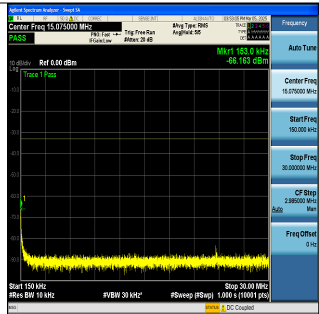
NTNV-n66-PC3-15-45-M-DFT-BPSK-Edge_1RB_Left- 0.15-30-PASS
