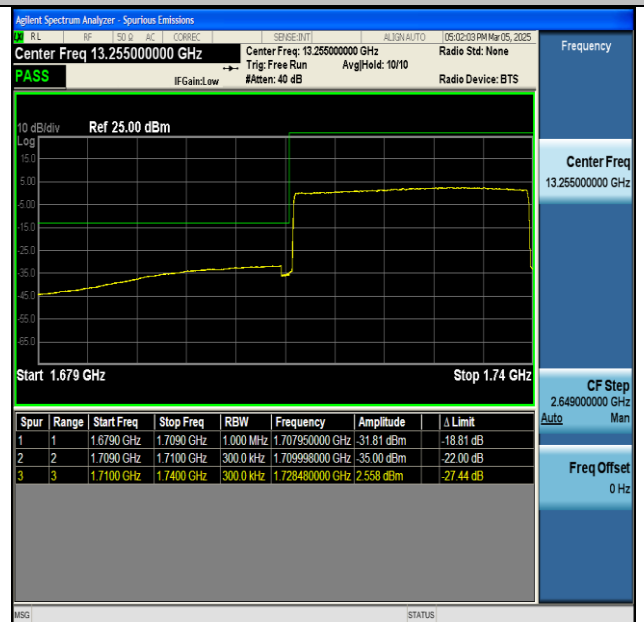
NTNV-n66-PC3-15-30-L-CP-QPSK-Outer_Full-PASS
