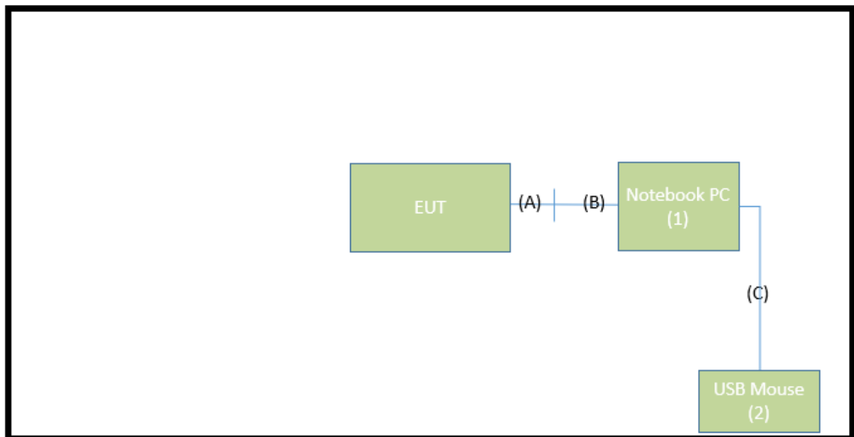
Connection Diagram
