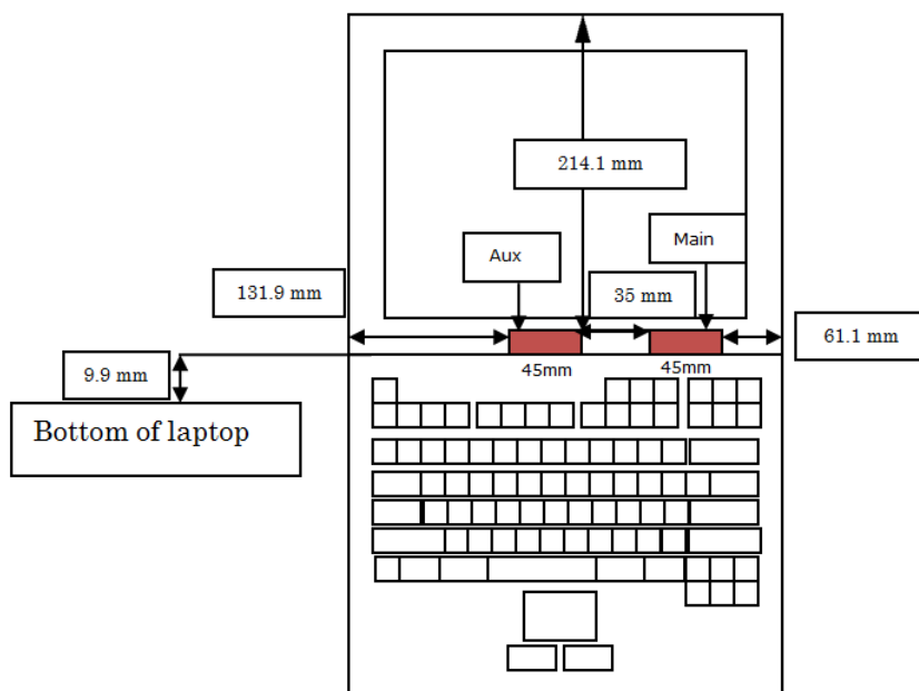
Fig.6 Antenna position of EUT (Front view)
