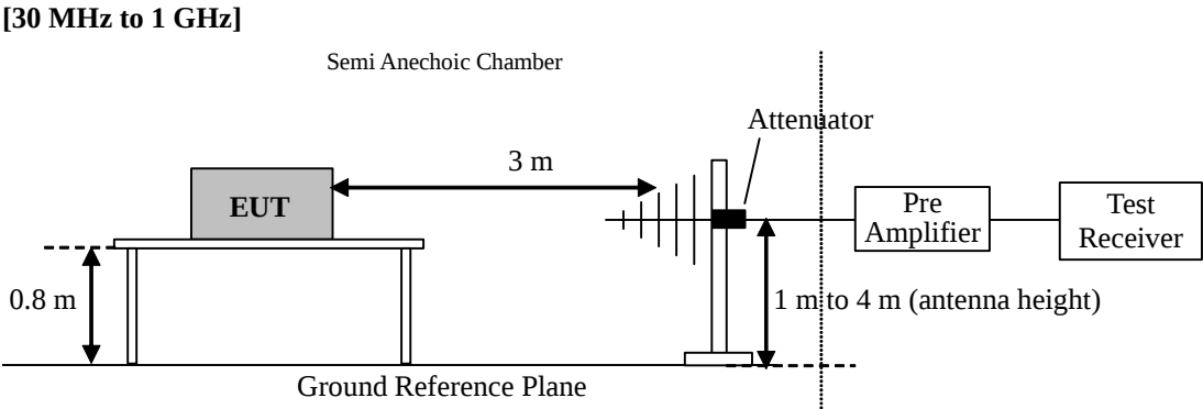
Figure 2: Test Setup
