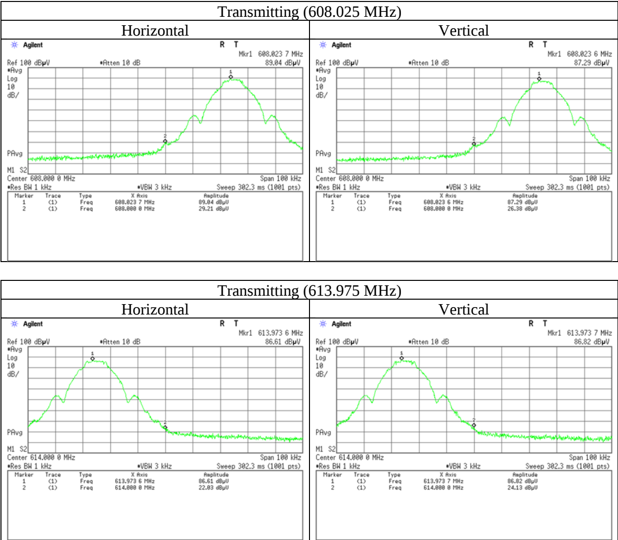
Reference Plot for Band Edge compliance (Marker Delta Method)
