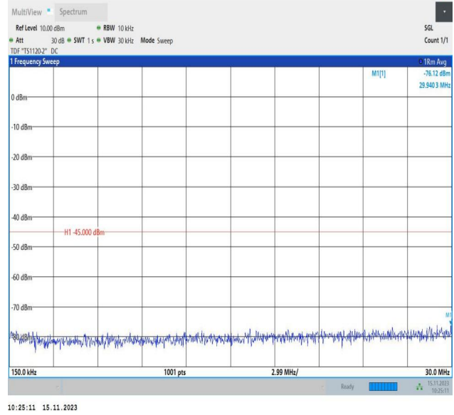
Band7_20MHz_QPSK_21100_1RB#0_0.15~30_0.15~30
