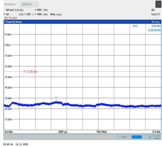
Band7_10MHz_16QAM_21100_1RB#0_20000~27000_20000~27000
