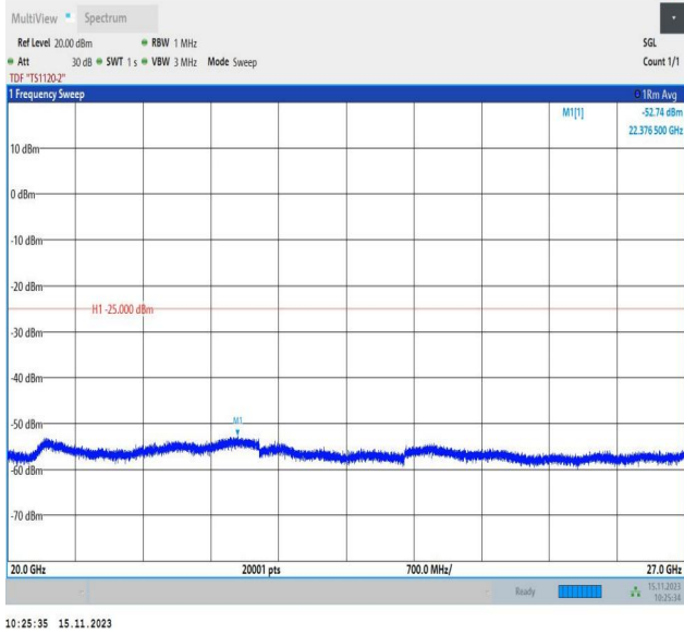
Band7_20MHz_QPSK_21100_1RB#0_20000~27000_20000~27000
