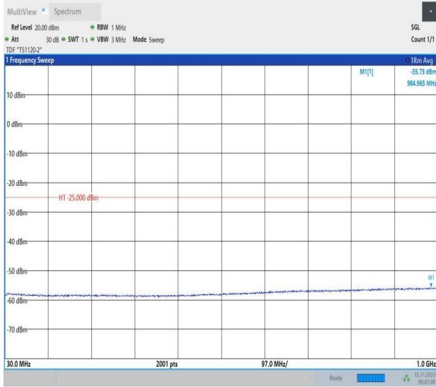
Band7_10MHz_QPSK_21400_1RB#0_30~1000_30~1000
