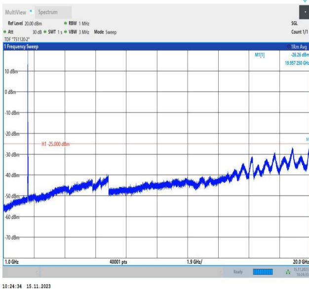
Band7_20MHz_16QAM_20850_1RB#0_1000~20000_1000~20000
