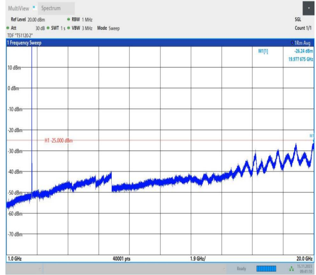
Band7_10MHz_QPSK_21400_1RB#0_1000~20000_1000~200 00
