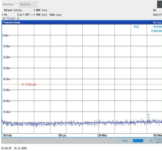
Band7_15MHz_16QAM_21100_1RB#0_0.15~30_0.15~30
