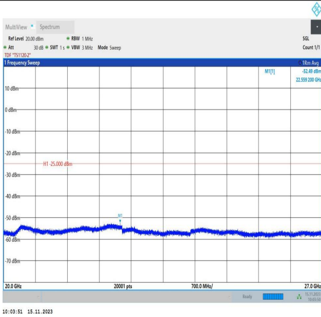
Band7_15MHz_QPSK_21375_1RB#0_20000~27000_20000~27000
