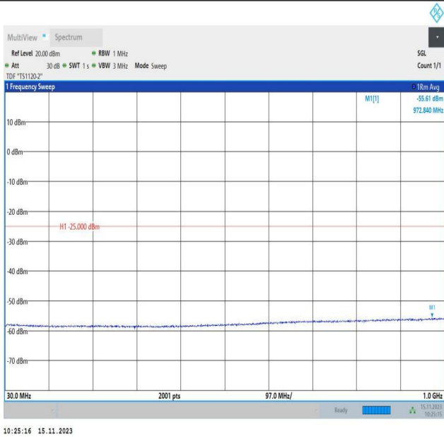
Band7_20MHz_QPSK_21100_1RB#0_30~1000_30~1000
