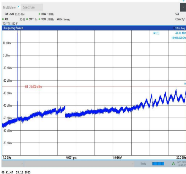
Band7_10MHz_16QAM_21400_1RB#0_1000~20000_1000~20000
