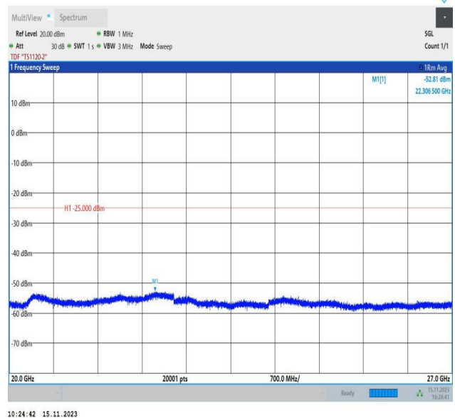
Band7_20MHz_16QAM_20850_1RB#0_20000~27000_20000~27000
