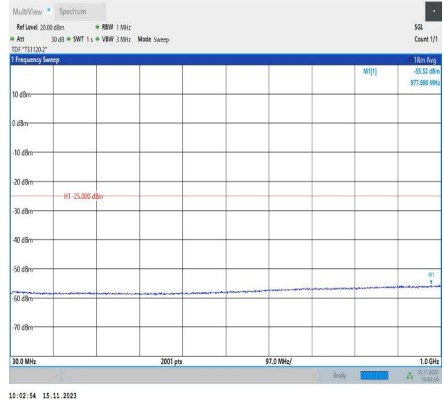
Band7_15MHz_16QAM_21100_1RB#0_30~1000_30~1000
