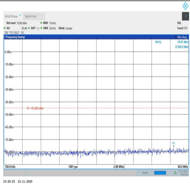
Band7_20MHz_QPSK_21350_1RB#0_0.15~30_0.15~30
