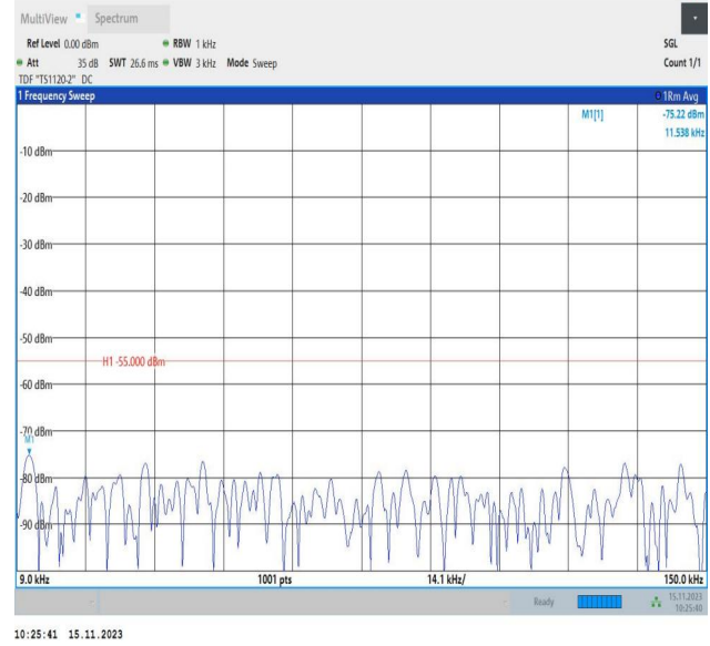
Band7_20MHz_16QAM_21100_1RB#0_0.009~0.15_0.009~0.15
