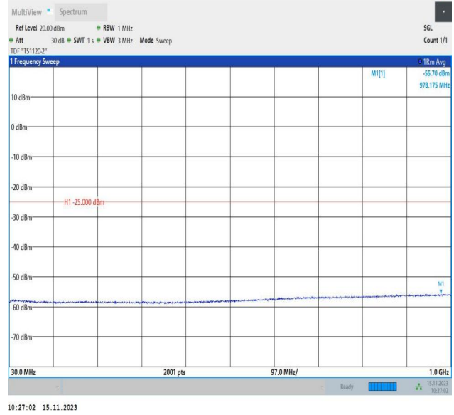
Band7_20MHz_16QAM_21350_1RB#0_30~1000_30~1000
