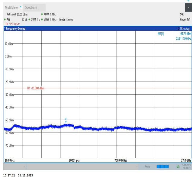
Band7_20MHz_16QAM_21350_1RB#0_20000~27000_20000~27000
