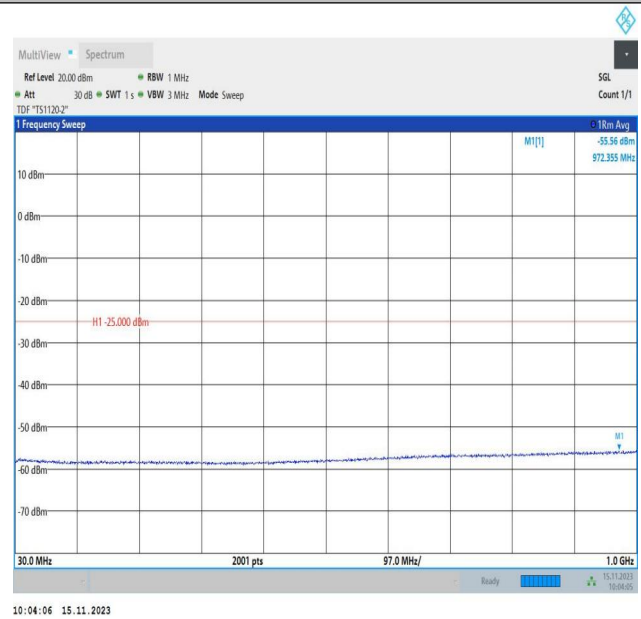
Band7_15MHz_16QAM_21375_1RB#0_30~1000_30~1000
