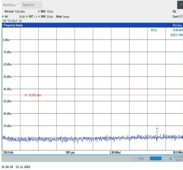
Band7_20MHz_16QAM_20850_1RB#0_0.15~30_0.15~30
