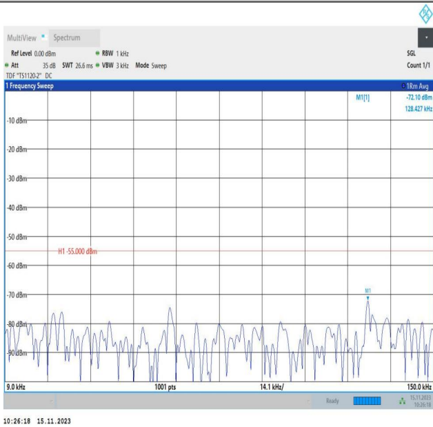
Band7_20MHz_QPSK_21350_1RB#0_0.009~0.15_0.009~0.15
