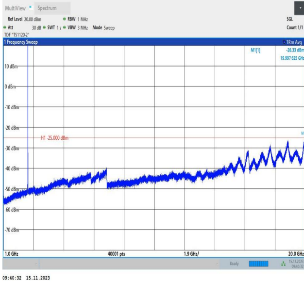
Band7_10MHz_16QAM_21100_1RB#0_1000~20000_1000~20000
