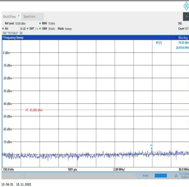
Band7_15MHz_16QAM_21375_1RB#0_0.15~30_0.15~30
