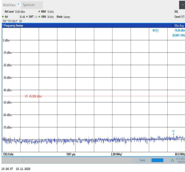
Band7_20MHz_16QAM_21350_1RB#0_0.15~30_0.15~30
