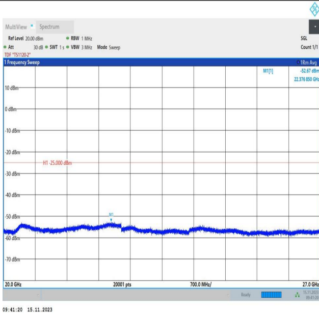
Band7_10MHz_QPSK_21400_1RB#0_20000~27000_20000~ 27000
