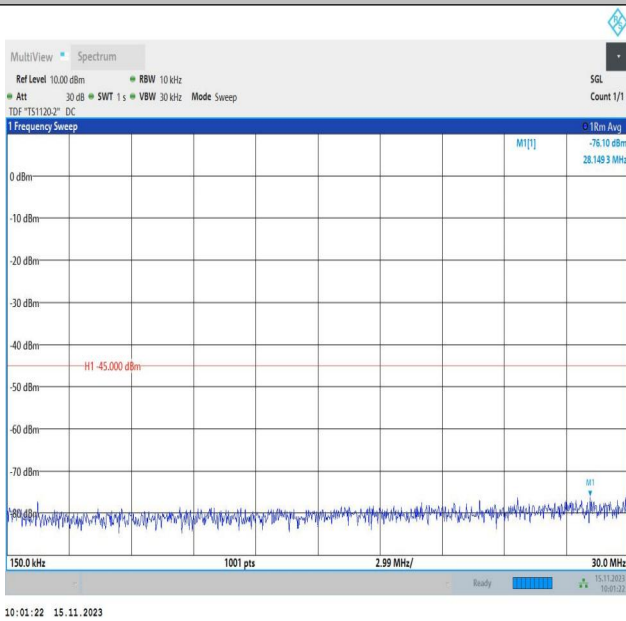
Band7_15MHz_16QAM_20825_1RB#0_0.15~30_0.15~30
