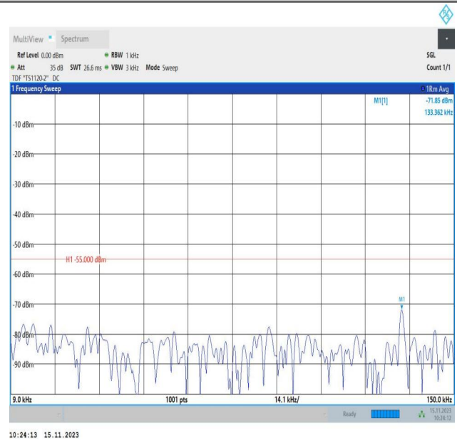
Band7_20MHz_16QAM_20850_1RB#0_0.009~0.15_0.009~0.1 5
