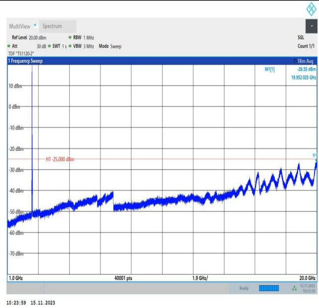
Band7_20MHz_QPSK_20850_1RB#0_1000~20000_1000~200 00
