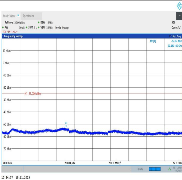
Band7_20MHz_QPSK_20850_1RB#0_20000~27000_20000~ 27000
