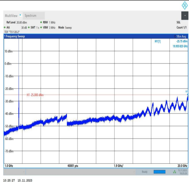
Band7_20MHz_QPSK_21100_1RB#0_1000~20000_1000~200
