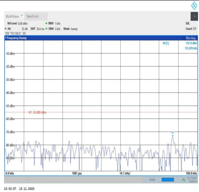
Band7_15MHz_16QAM_21375_1RB#0_0.009~0.15_0.009~0.15
