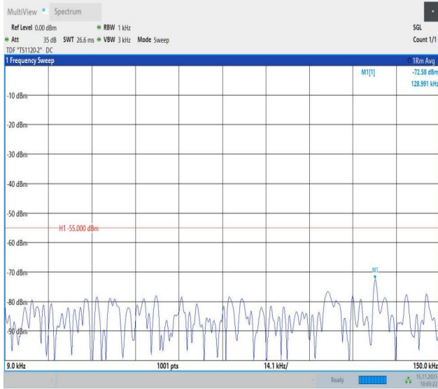
Band7_15MHz_QPSK_21375_1RB#0_0.009~0.15_0.009~0.1
