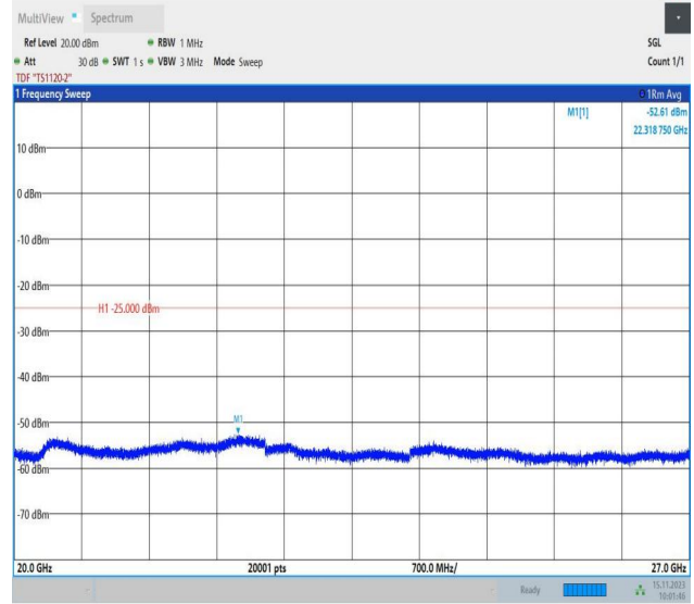
Band7_15MHz_16QAM_20825_1RB#0_20000~27000_20000~27000
