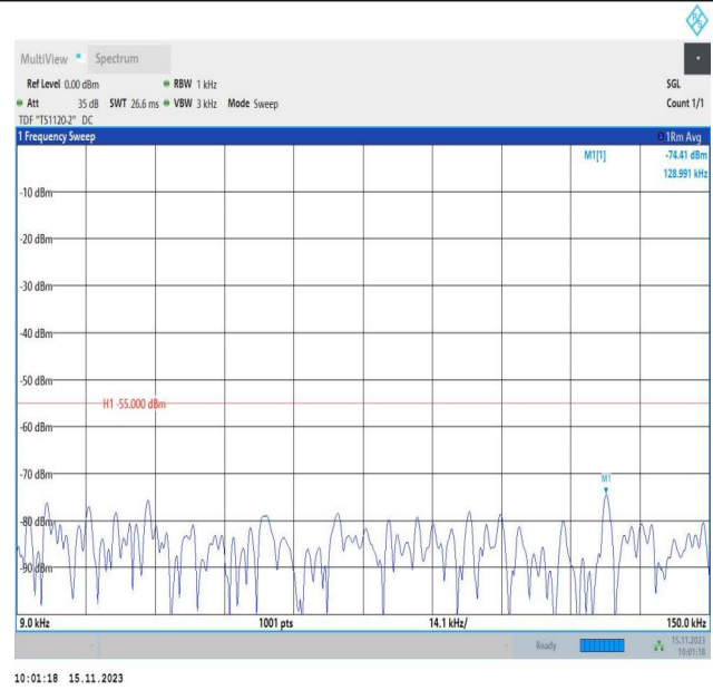
Band7_15MHz_16QAM_20825_1RB#0_0.009~0.15_0.009~0.15
