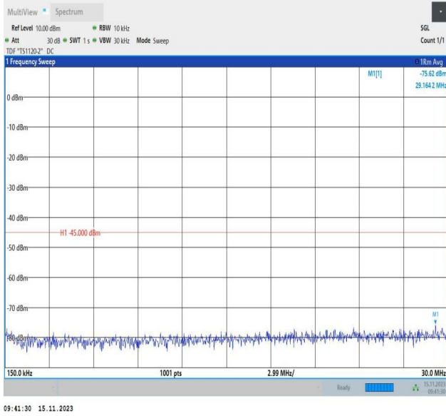
Band7_10MHz_16QAM_21400_1RB#0_0.15~30_0.15~30
