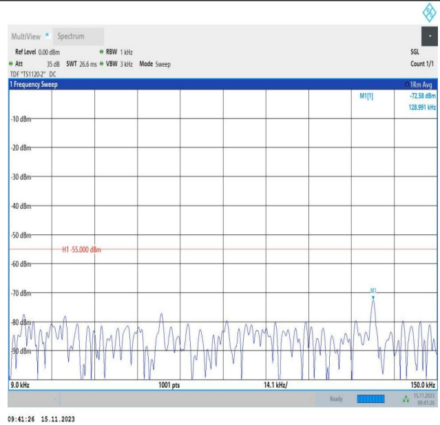
Band7_10MHz_16QAM_21400_1RB#0_0.009~0.15_0.009~0.1 5
