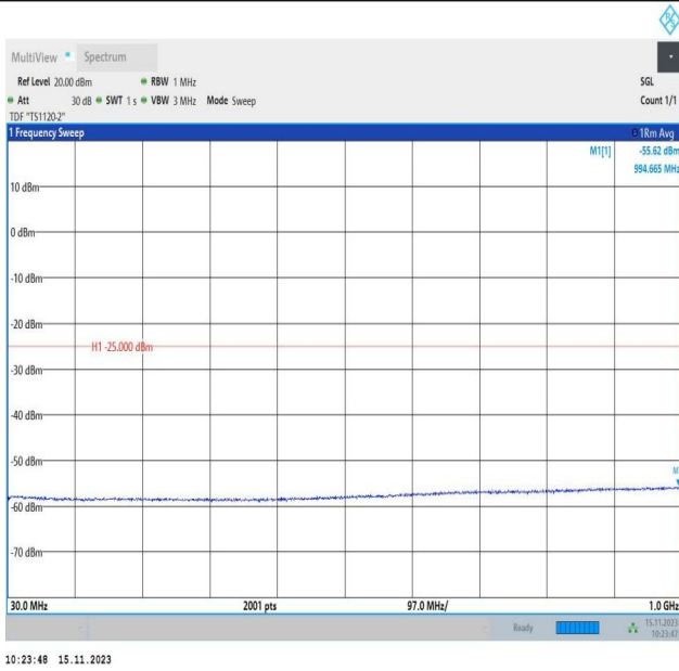
Band7_20MHz_QPSK_20850_1RB#0_30~1000_30~1000
