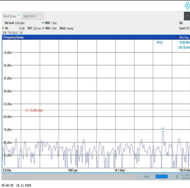
Band7_10MHz_QPSK_21400_1RB#0_0.009~0.15_0.009~0.15
