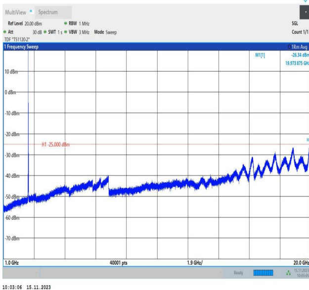
Band7_15MHz_16QAM_21100_1RB#0_1000~20000_1000~20000
