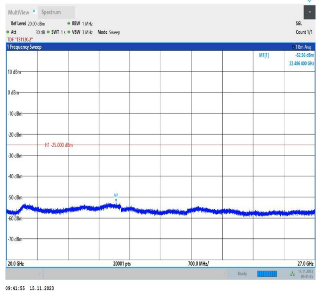
Band7_10MHz_16QAM_21400_1RB#0_20000~27000_20000~27000
