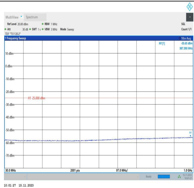
Band7_15MHz_16QAM_20825_1RB#0_30~1000_30~1000
