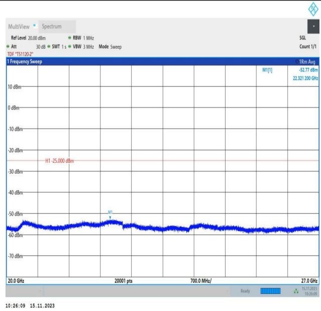
Band7_20MHz_16QAM_21100_1RB#0_20000~27000_20000~27000
