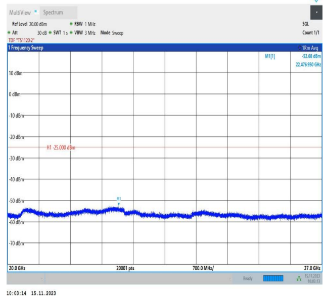
Band7_15MHz_16QAM_21100_1RB#0_20000~27000_20000~27000
