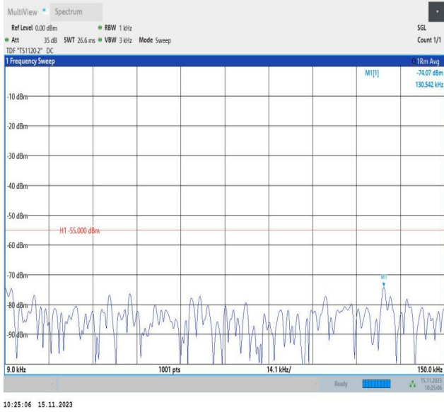
Band7_20MHz_QPSK_21100_1RB#0_0.009~0.15_0.009~0.1
