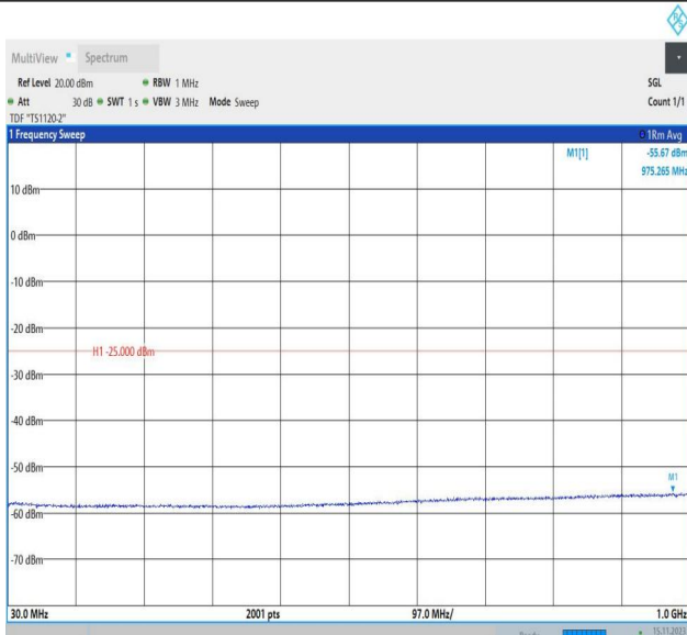
Band7_15MHz_QPSK_21375_1RB#0_30~1000_30~1000
