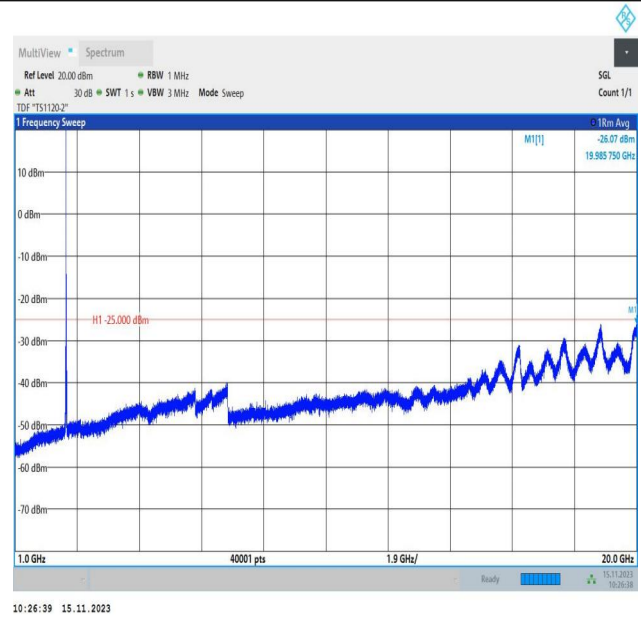
Band7_20MHz_QPSK_21350_1RB#0_1000~20000_1000~200 00
