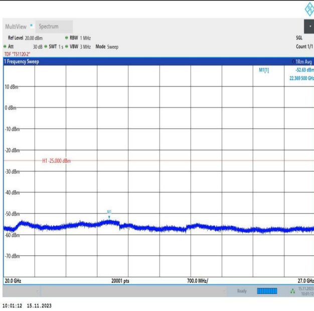
Band7_15MHz_QPSK_20825_1RB#0_20000~27000_20000~27000
