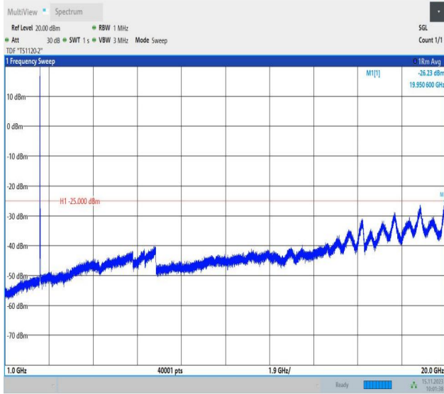
Band7_15MHz_16QAM_20825_1RB#0_1000~20000_1000~20000
