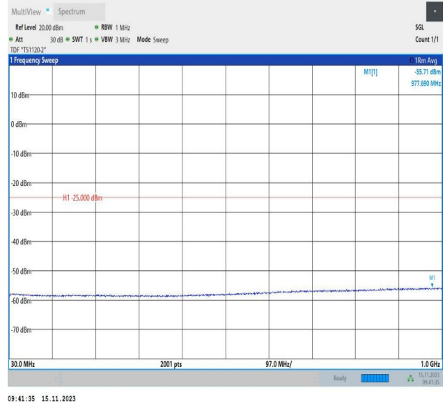
Band7_10MHz_16QAM_21400_1RB#0_30~1000_30~1000
