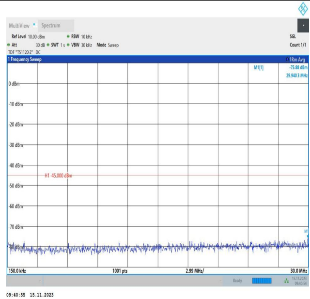
Band7_10MHz_QPSK_21400_1RB#0_0.15~30_0.15~30
