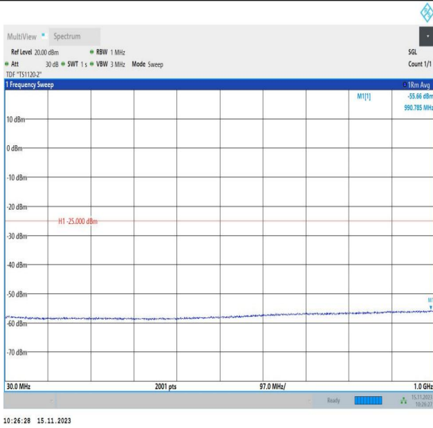
Band7_20MHz_QPSK_21350_1RB#0_30~1000_30~1000
