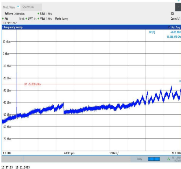
Band7_20MHz_16QAM_21350_1RB#0_1000~20000_1000~20000
