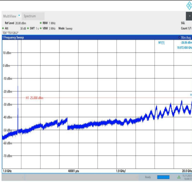
Band7_15MHz_16QAM_21375_1RB#0_1000~20000_1000~20000
