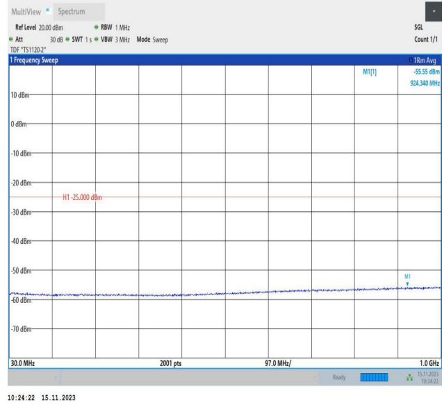
Band7_20MHz_16QAM_20850_1RB#0_30~1000_30~1000
