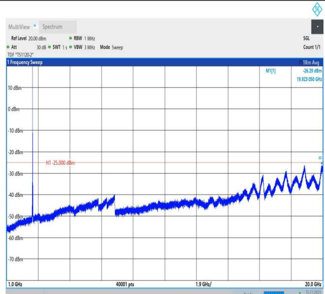
Band7_15MHz_QPSK_21375_1RB#0_1000~20000_1000~2000
