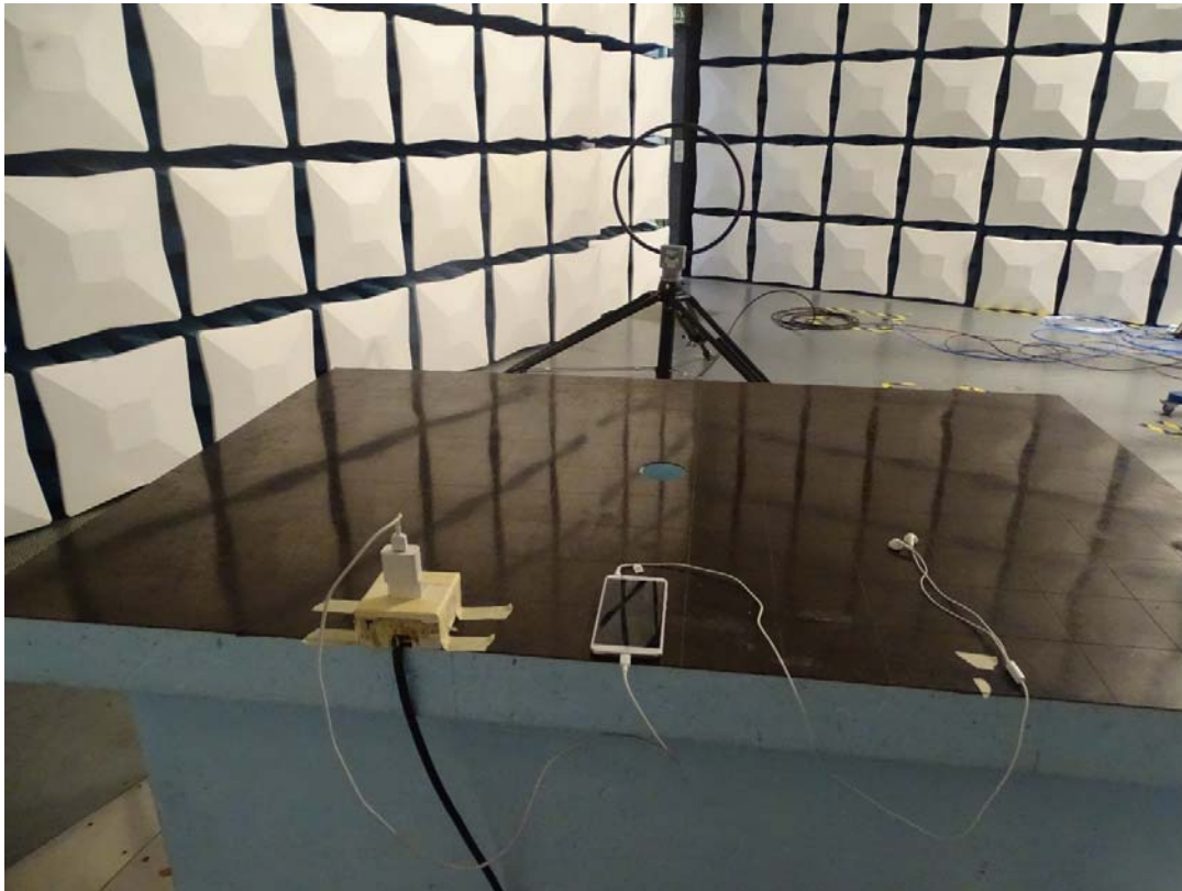
Radiated Spurious Emission (9K-30MHz)
