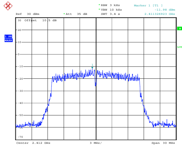
802.11g_2412MHz
