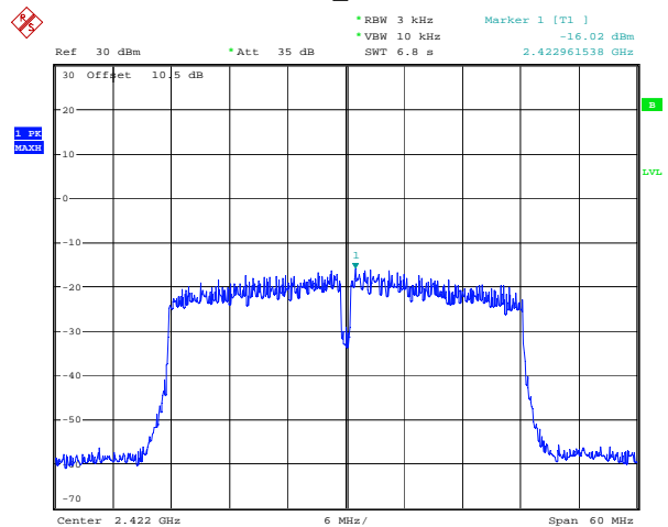
802.11n40_2422MHz
