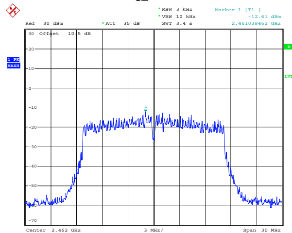
802.11g_2462MHz
