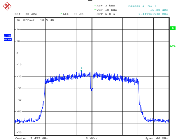
802.11n40_2452MHz
