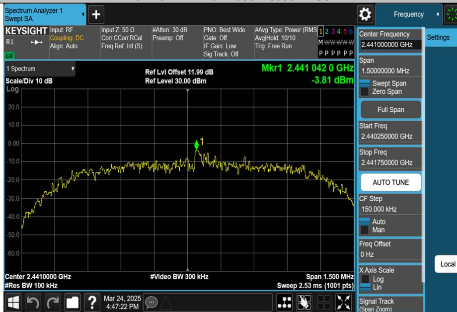
3DH5-Ant1-2441-0~Reference-PASS
