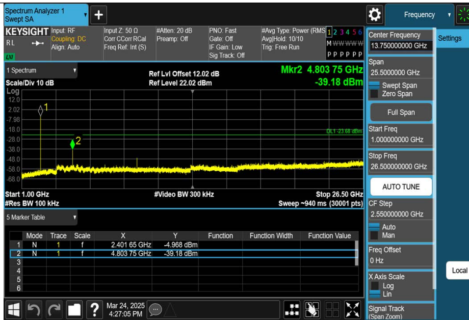
DH5-Ant1-2402-1000~26500-PASS
