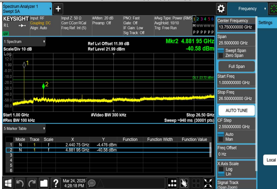
DH5-Ant1-2441-1000~26500-PASS
