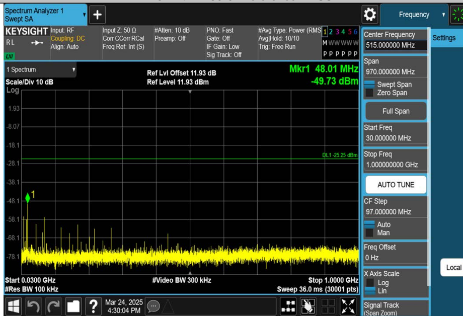
DH5-Ant1-2480-30~1000-PASS
