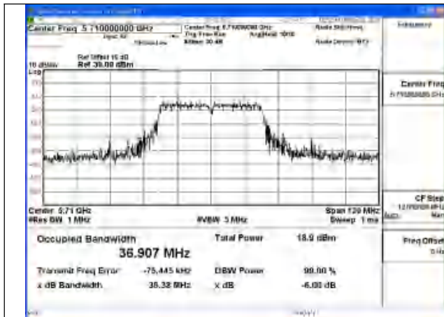
Test Mode: 802.11n HT40
