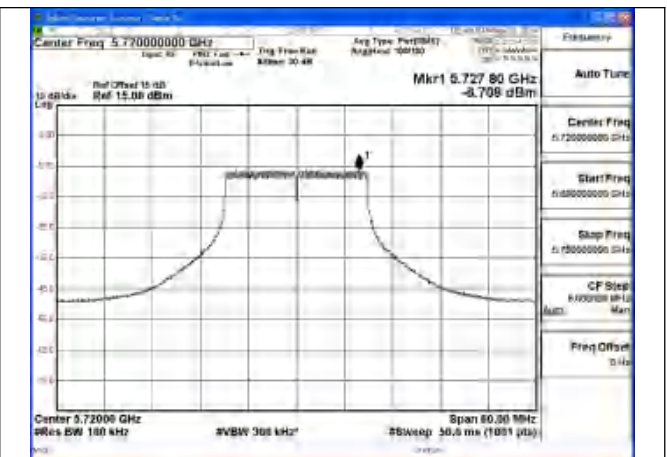
Mode:802.11n HT20 Frequency:5720MHz Ant:Chain0 scope:NII3
