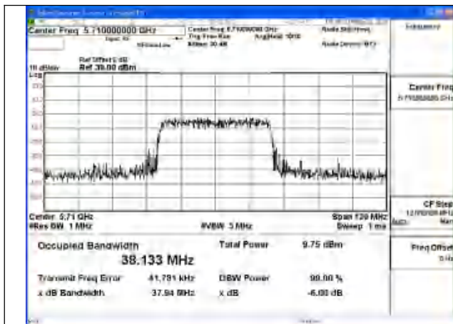
Test Mode: 802.11ax HE40
