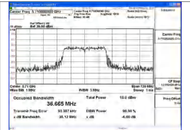
Test Mode: 802.11ac VHT40
