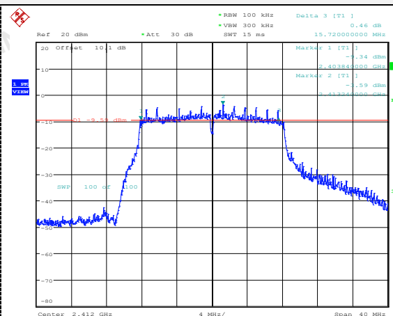
802.11g
