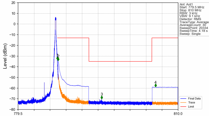
Band13_5MHz_16QAM_HCH_784.5MHz_RB_1_24_NTNV
