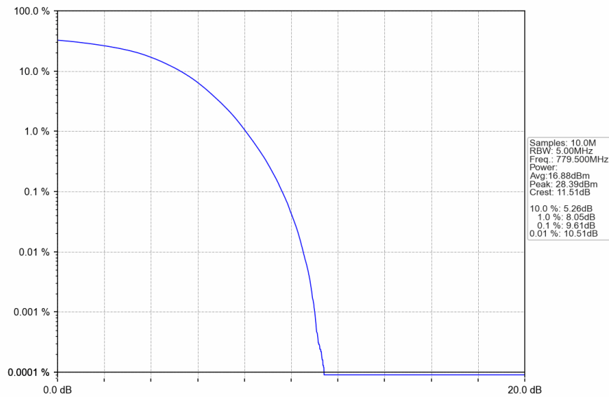
Band13_5MHz_64QAM_LCH_779.5MHz_RB_25_0_NTNV
