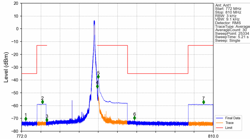
Band13_10MHz_16QAM_HCH_782MHz_RB_1_49_NTNV
