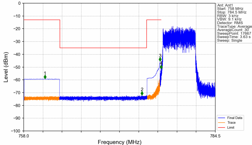
Band13_5MHz_64QAM_LCH_779.5MHz_RB_25_0_NTNV
