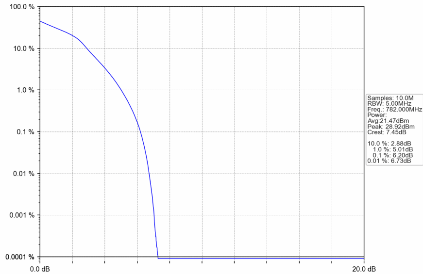
Band13_5MHz_16QAM_MCH_782MHz_RB_25_0_NTNV
