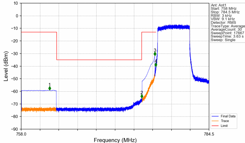
Band13_5MHz_QPSK_LCH_779.5MHz_RB_25_0_NTNV
