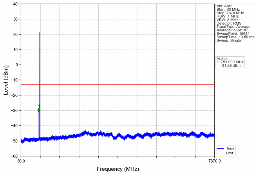
Band13_5MHz_16QAM_HCH_784.5MHz_RB_1_0_NTNV
