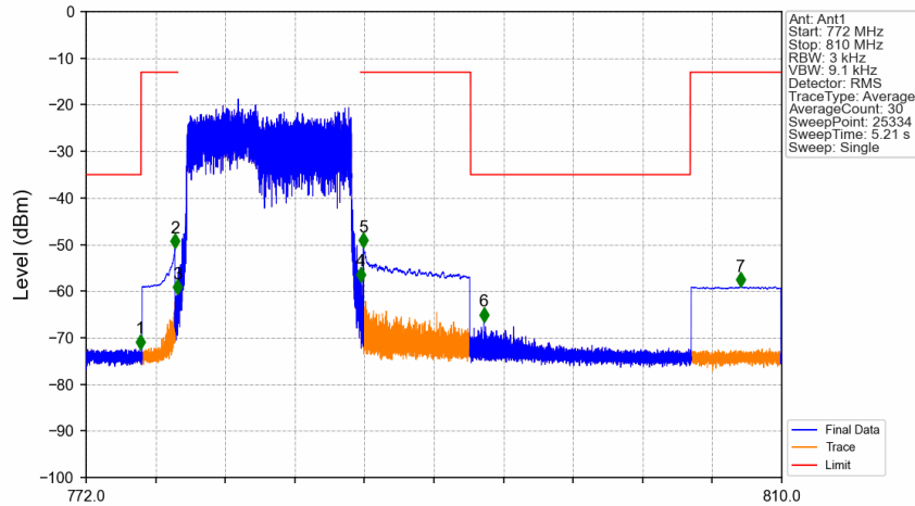
Band13_10MHz_64QAM_HCH_782MHz_RB_50_0_NTNV
