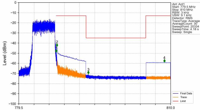
Band13_5MHz_64QAM_HCH_784.5MHz_RB_25_0_NTNV
