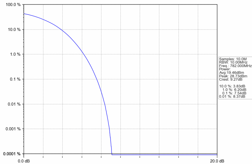
Band13_10MHz_64QAM_MCH_782MHz_RB_50_0_NTNV
