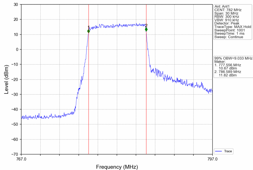
Band13_10MHz_64QAM_MCH_782MHz_RB_50_0_NTNV
