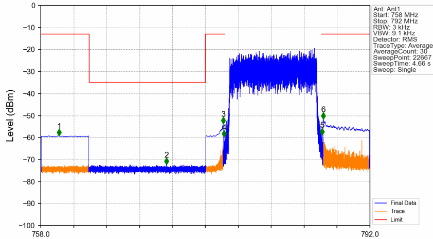
Band13_10MHz_64QAM_LCH_782MHz_RB_50_0_NTNV
