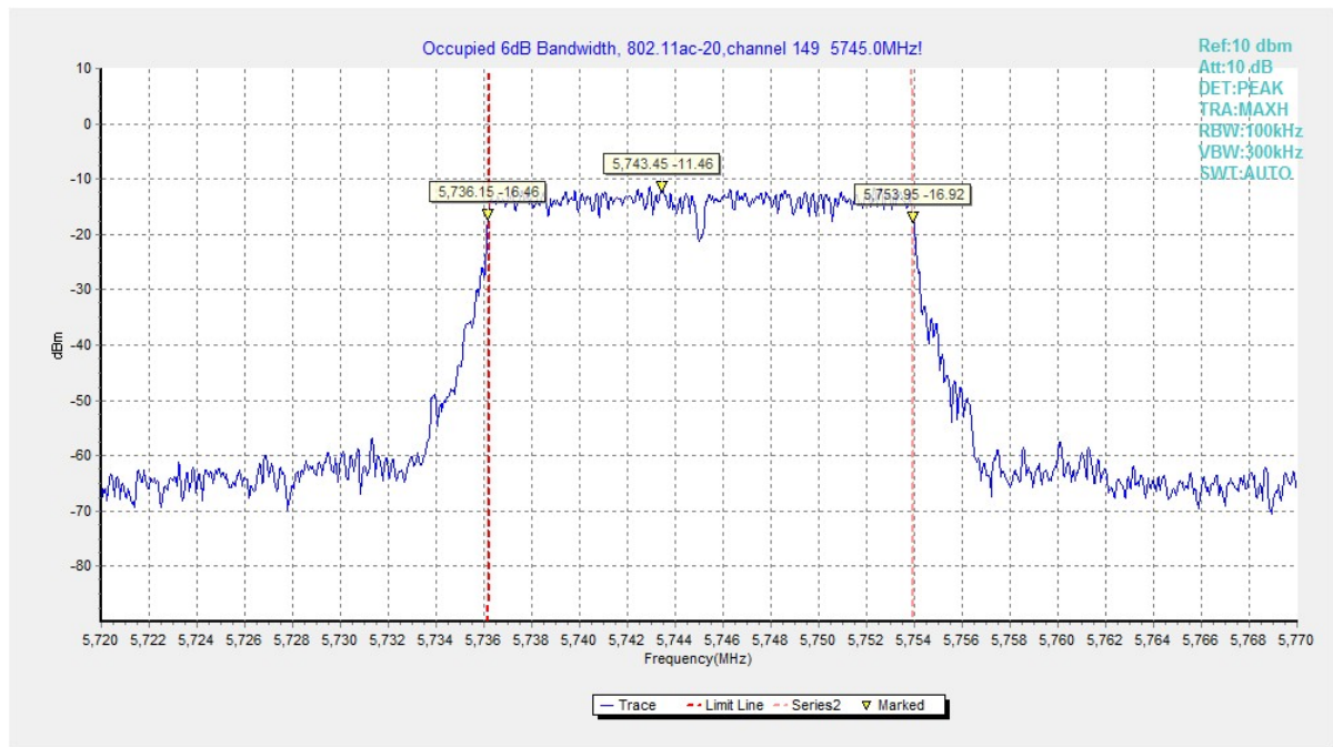
Fig. 7 Occupied 6dB Bandwidth (802.11ac20, Ch 149)
