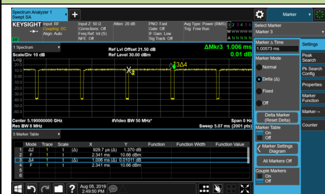
802.11ac-VHT40 (T = 929.7μs)
