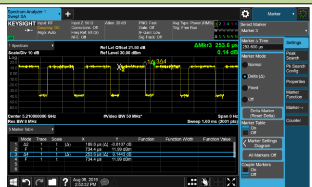
802.11ac-VHT80 (T = 189.6μs)
