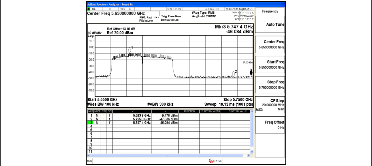
11AC80MIMO_Ant2_High_5610
