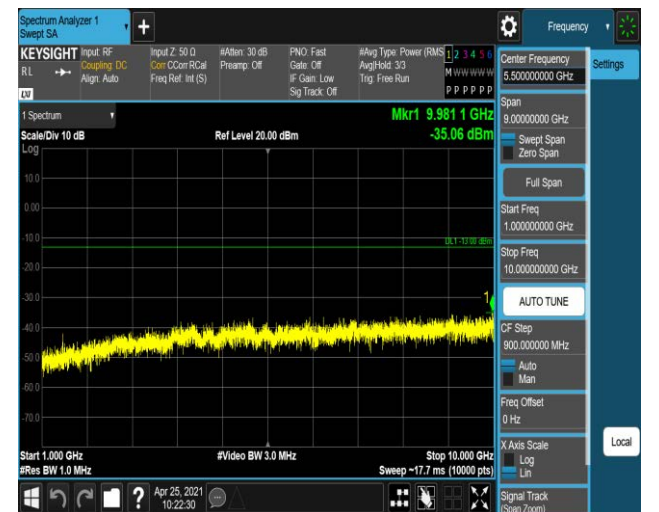
Band17-10MHz-16QAM-23780-1RB#0-Range2:1000~10000MHz
