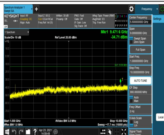
Band12-10MHz-QPSK-23130-1RB#0-Range2:1000~10
