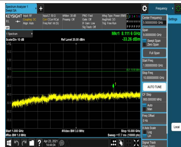
Band12-10MHz-QPSK-23060-1RB#0-Range2:1000~10
