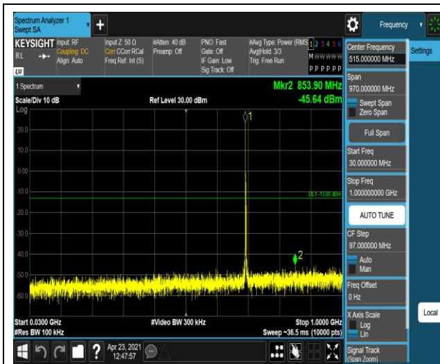
Band12-3MHz-QPSK-23095-1RB#0-Range1:30~10
