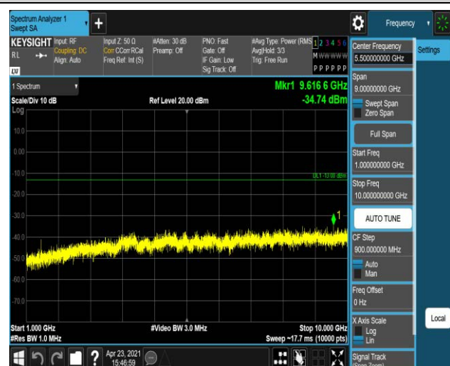
Band17-5MHz-QPSK-23825-1RB#0-Range2:1000~100
