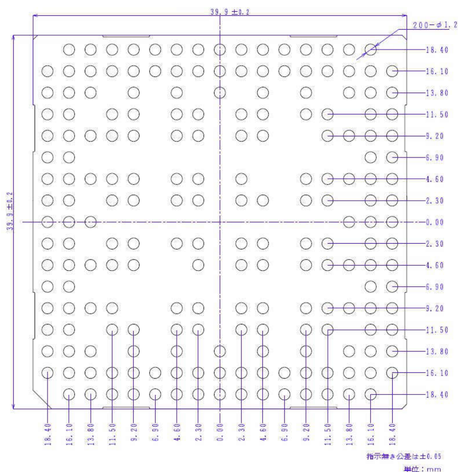
Figure. 7-1 Bottom view with dimensions
