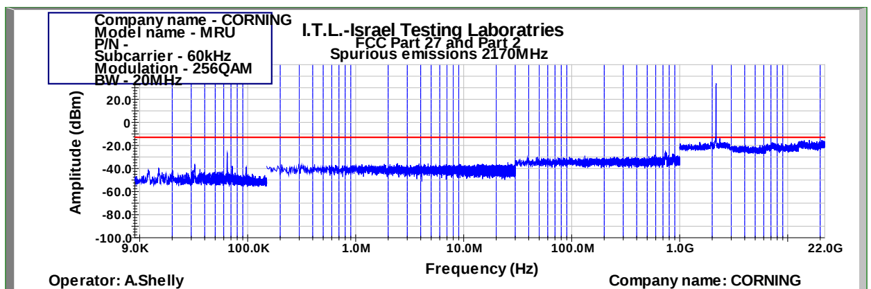
Figure 965: Spurious Emissions at Antenna Terminal 256QAM 20MHz B.W.; 2170.0MHz, 60kHz
