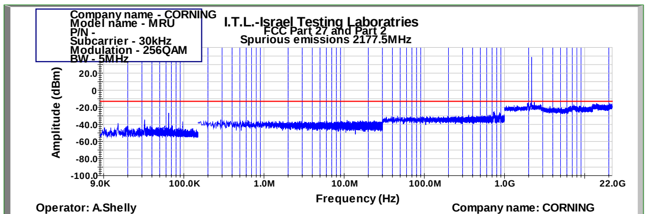
Figure 938: Spurious Emissions at Antenna Terminal 256QAM 5MHz B.W.; 2177.5MHz, 30kHz
