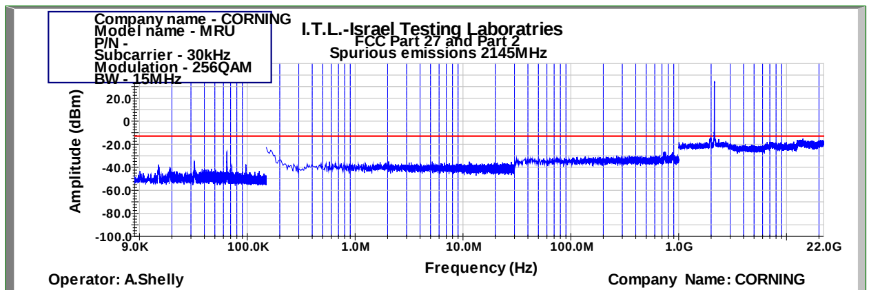
Figure 952: Spurious Emissions at Antenna Terminal 256QAM 15MHz B.W.; 2145.0MHz, 30kHz
