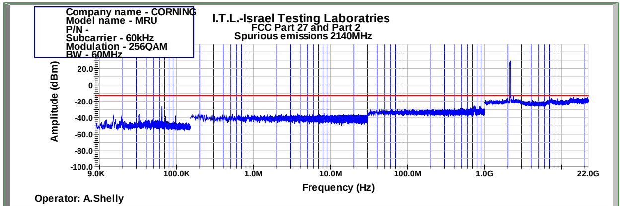
Figure 996: Spurious Emissions at Antenna Terminal 256QAM 60MHz B.W.; 2140.0MHz, 60kHz
