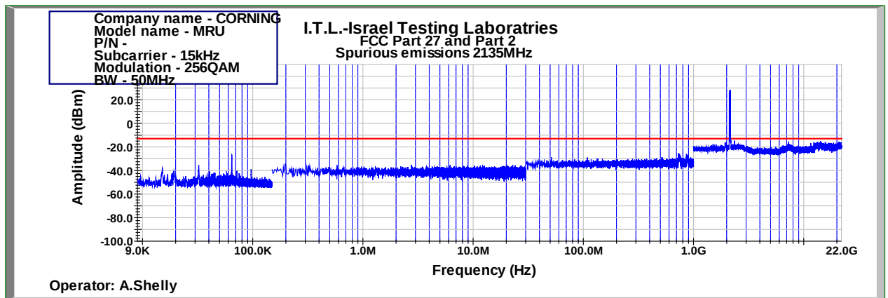
Figure 984: Spurious Emissions at Antenna Terminal 256QAM 50MHz B.W.; 2135.0MHz, 15kHz
