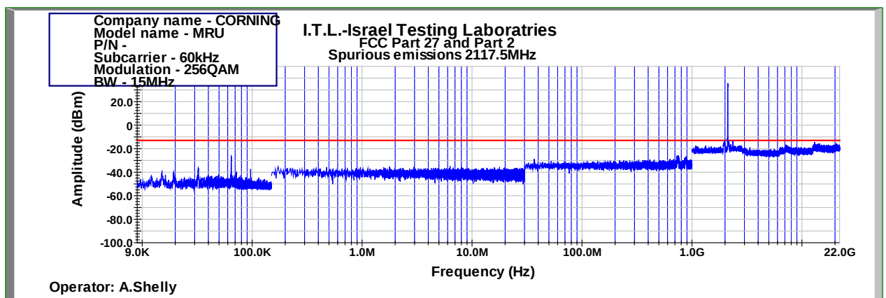
Figure 954: Spurious Emissions at Antenna Terminal 256QAM 15MHz B.W.; 2117.5MHz, 60kHz
