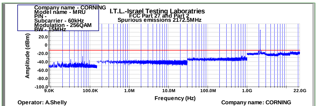
Figure 956: Spurious Emissions at Antenna Terminal 256QAM 15MHz B.W.; 2172.5MHz, 60kHz
