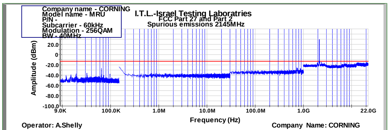
Figure 982: Spurious Emissions at Antenna Terminal 256QAM 40MHz B.W.; 2145.0MHz, 60kHz
