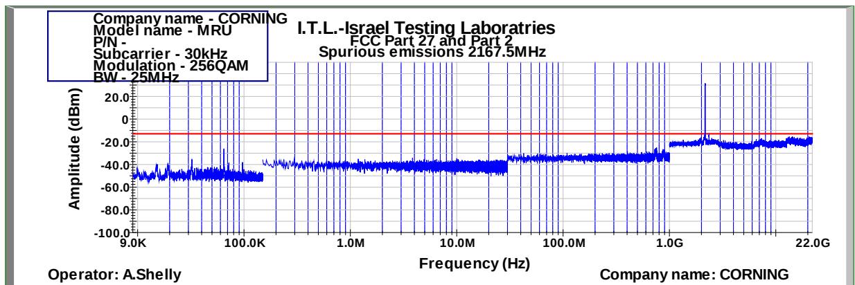
Figure 971: Spurious Emissions at Antenna Terminal 256QAM 25MHz B.W.; 2167.5MHz, 30kHz
