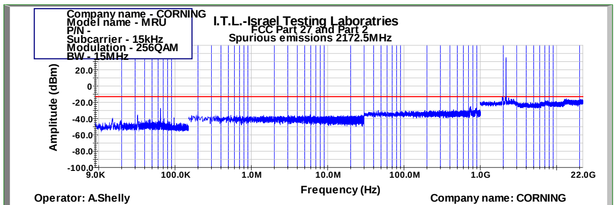
Figure 950: Spurious Emissions at Antenna Terminal 256QAM 15MHz B.W.; 2172.5MHz, 15kHz
