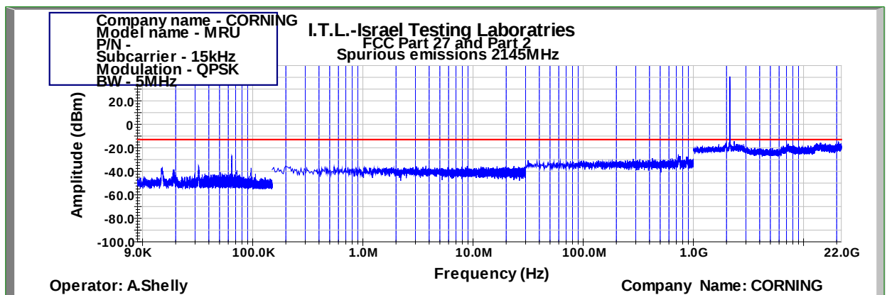
Figure 1000: Spurious Emissions at Antenna Terminal QPSK 5MHz B.W.; 2145.0MHz, 15kHz
