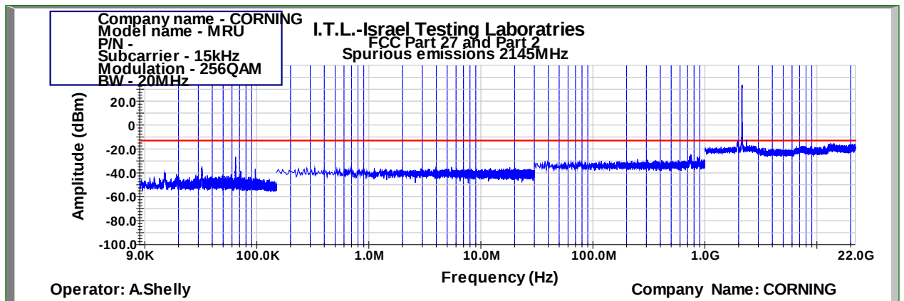
Figure 958: Spurious Emissions at Antenna Terminal 256QAM 20MHz B.W.; 2145.0MHz, 15kHz
