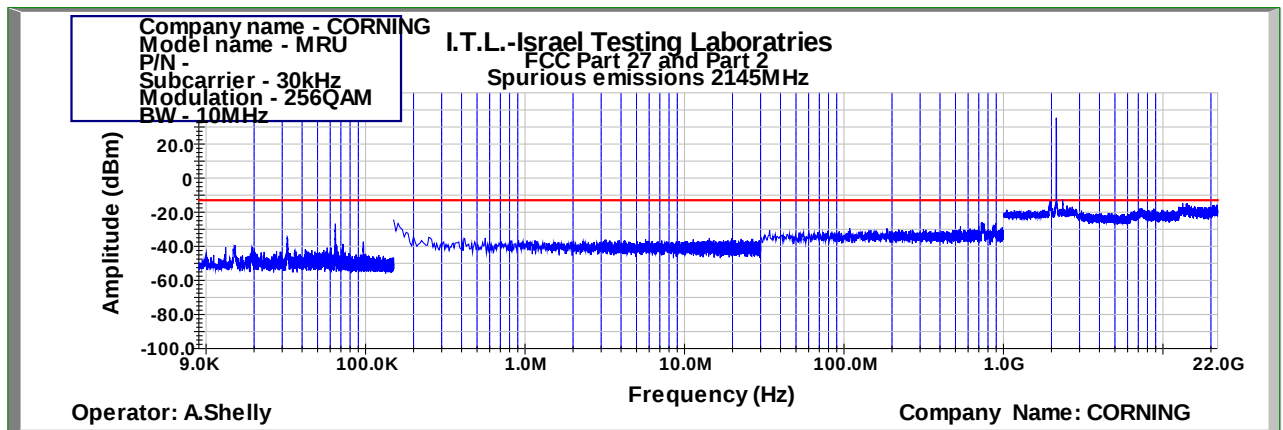
Figure 943: Spurious Emissions at Antenna Terminal 256QAM 10MHz B.W.; 2145.0MHz, 30kHz
