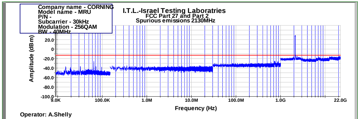
Figure 978: Spurious Emissions at Antenna Terminal 256QAM 40MHz B.W.; 2130.0MHz, 30kHz
