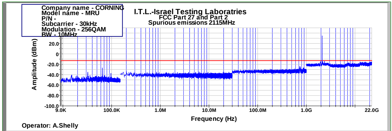
Figure 942: Spurious Emissions at Antenna Terminal 256QAM 10MHz B.W.; 2115.0MHz, 30kHz
