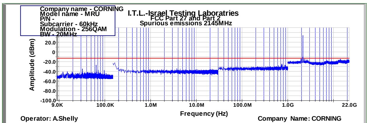
Figure 964: Spurious Emissions at Antenna Terminal 256QAM 20MHz B.W.; 2145.0MHz, 60kHz
