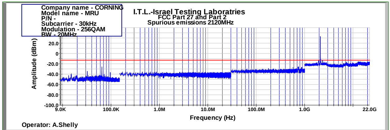
Figure 960: Spurious Emissions at Antenna Terminal 256QAM 20MHz B.W.; 2120.0MHz, 30kHz
