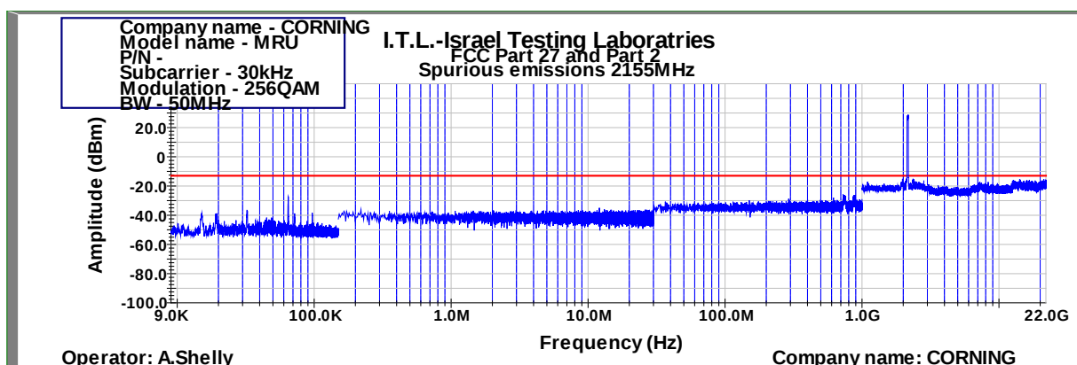
Figure 989: Spurious Emissions at Antenna Terminal 256QAM 50MHz B.W.; 2155.0MHz, 30kHz
