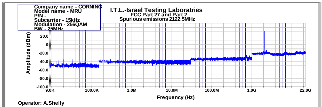
Figure 966: Spurious Emissions at Antenna Terminal 256QAM 25MHz B.W.; 2122.5MHz, 15kHz
