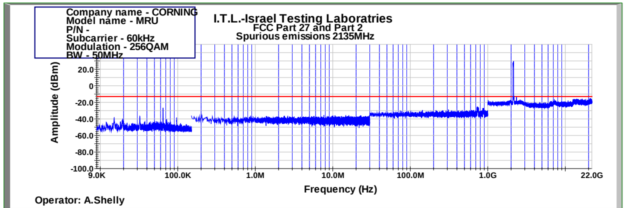
Figure 990: Spurious Emissions at Antenna Terminal 256QAM 50MHz B.W.; 2135.0MHz, 60kHz
