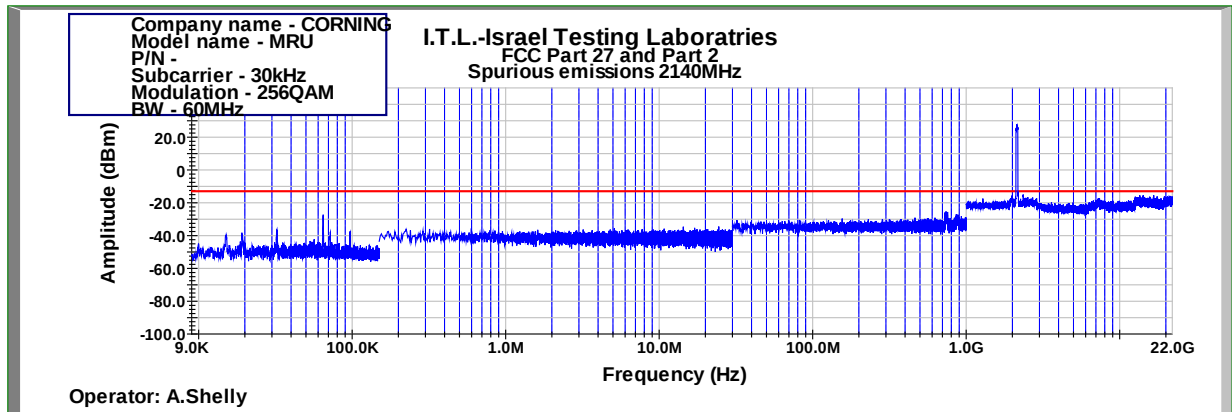
Figure 993: Spurious Emissions at Antenna Terminal 256QAM 60MHz B.W.; 2140.0MHz, 30kHz
