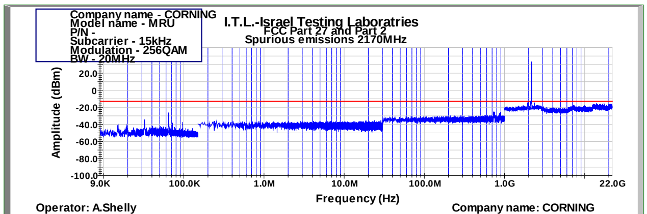
Figure 959: Spurious Emissions at Antenna Terminal 256QAM 20MHz B.W.; 2170.0MHz, 15kHz
