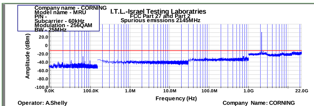
Figure 973: Spurious Emissions at Antenna Terminal 256QAM 25MHz B.W.; 2145.0MHz, 60kHz
