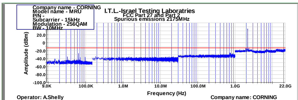
Figure 941: Spurious Emissions at Antenna Terminal 256QAM 10MHz B.W.; 2175.00MHz, 15kHz
