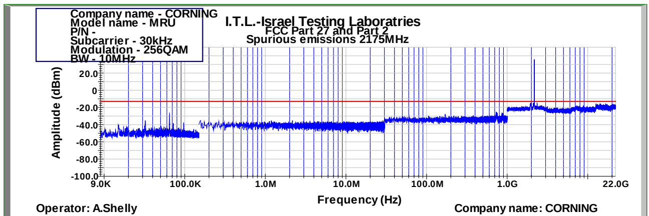
Figure 944: Spurious Emissions at Antenna Terminal 256QAM 10MHz B.W.; 2175.0MHz, 30kHz
