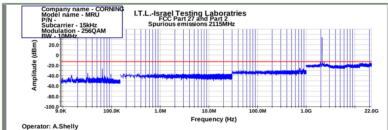
Figure 939: Spurious Emissions at Antenna Terminal 256QAM 10MHz B.W.; 2115.0MHz, 15kHz
