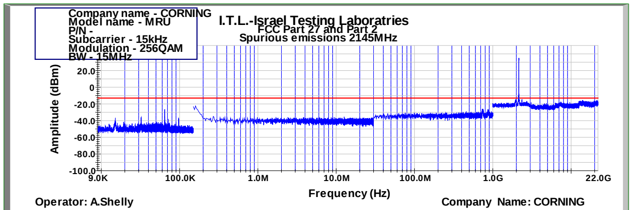
Figure 949: Spurious Emissions at Antenna Terminal 256QAM 15MHz B.W.; 2145.0MHz, 15kHz
