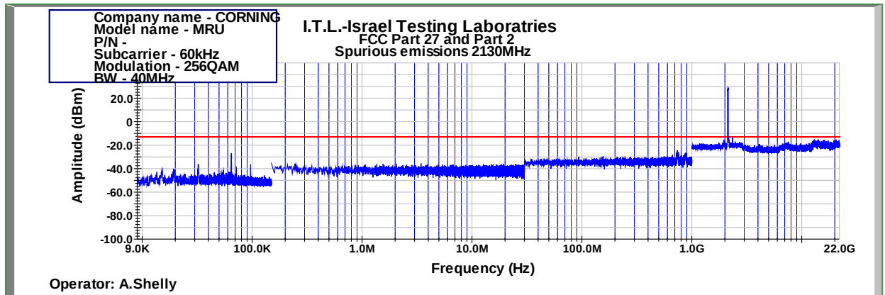
Figure 981: Spurious Emissions at Antenna Terminal 256QAM 40MHz B.W.; 2130.0MHz, 60kHz
