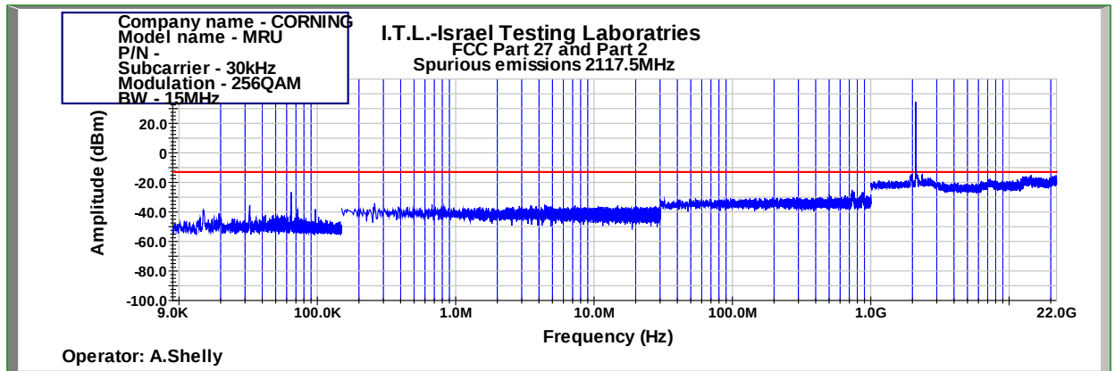
Figure 951: Spurious Emissions at Antenna Terminal 256QAM 15MHz B.W.; 2117.5MHz, 30kHz
