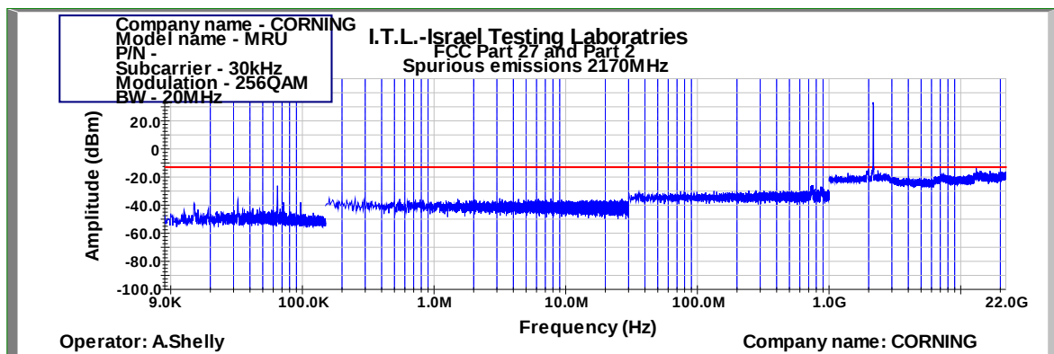
Figure 962: Spurious Emissions at Antenna Terminal 256QAM 20MHz B.W.; 2170.0MHz, 30kHz
