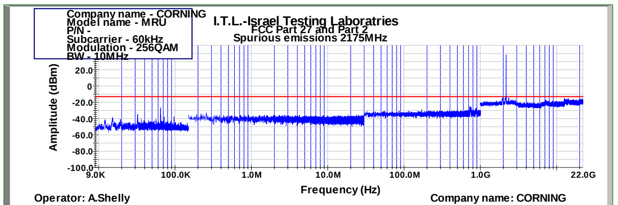
Figure 947: Spurious Emissions at Antenna Terminal 256QAM 10MHz B.W.; 2175.0MHz, 60kHz
