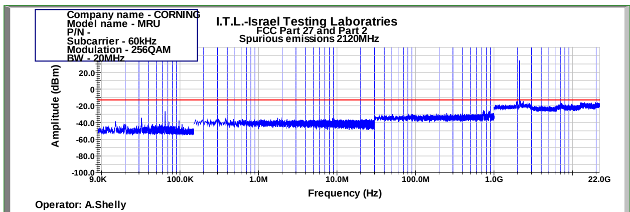
Figure 963: Spurious Emissions at Antenna Terminal 256QAM 20MHz B.W.; 2120.0MHz, 60kHz
