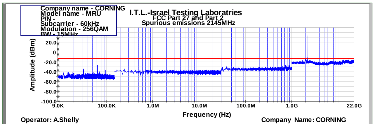
Figure 955: Spurious Emissions at Antenna Terminal 256QAM 15MHz B.W.; 2145.0MHz, 60kHz
