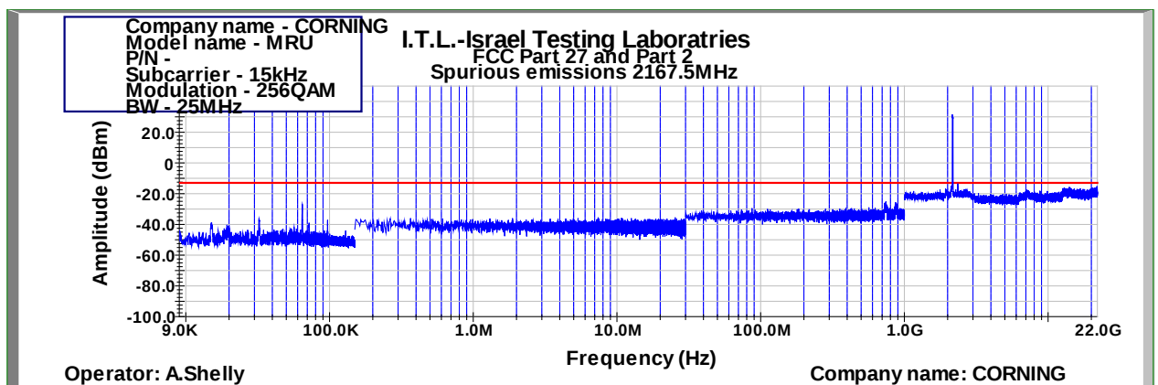
Figure 968: Spurious Emissions at Antenna Terminal 256QAM 25MHz B.W.; 2167.5MHz, 15kHz
