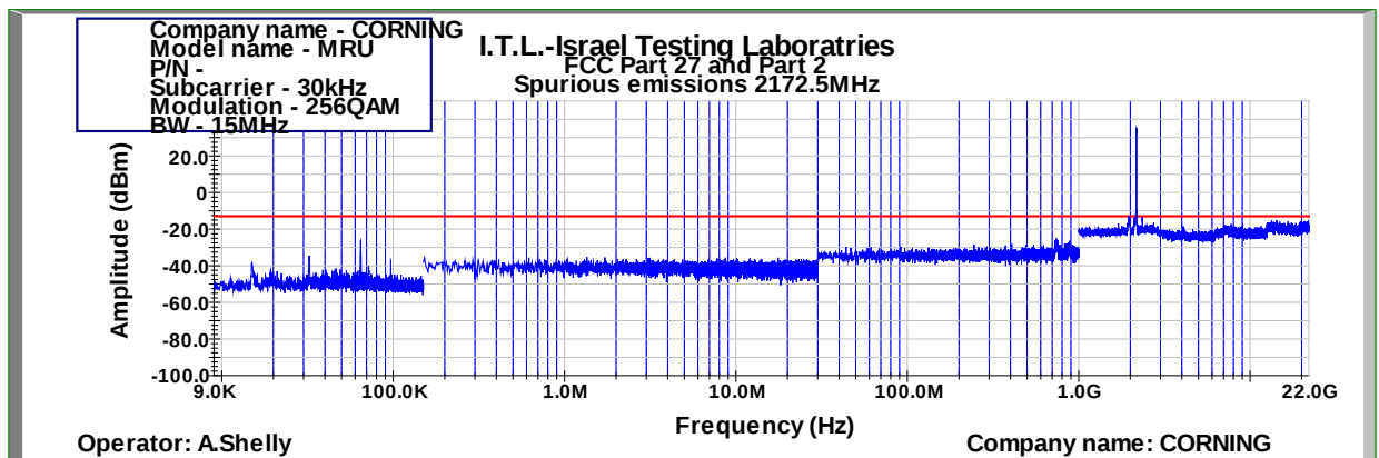
Figure 953: Spurious Emissions at Antenna Terminal 256QAM 15MHz B.W.; 2172.5MHz, 30kHz
