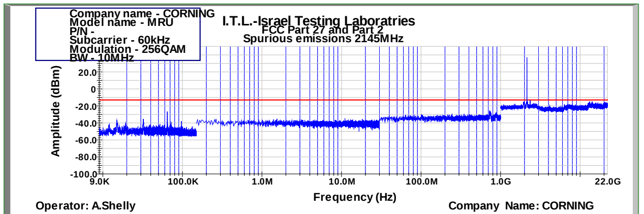
Figure 946: Spurious Emissions at Antenna Terminal 256QAM 10MHz B.W.; 2145.0MHz, 60kHz
