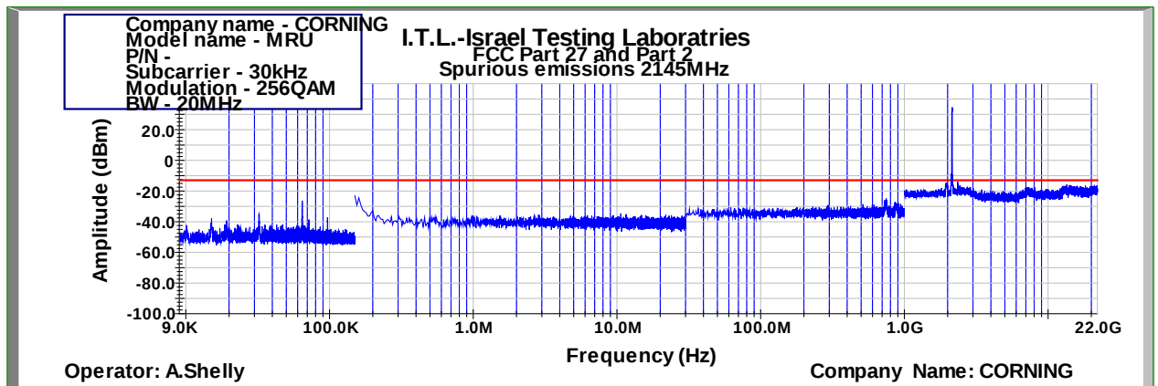
Figure 961: Spurious Emissions at Antenna Terminal 256QAM 20MHz B.W.; 2145.0MHz, 30kHz
