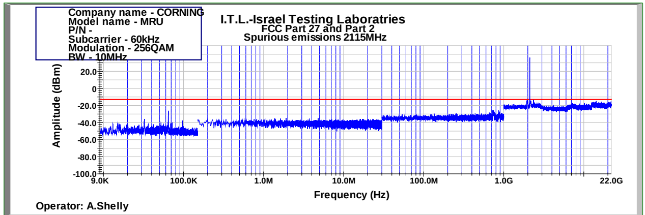
Figure 945: Spurious Emissions at Antenna Terminal 256QAM 10MHz B.W.; 2115.0MHz, 60kHz
