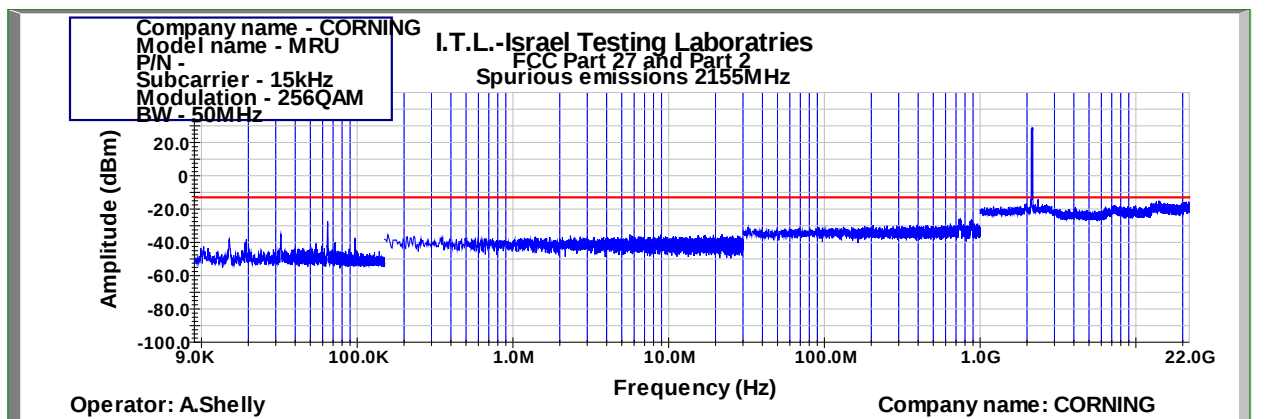
Figure 986: Spurious Emissions at Antenna Terminal 256QAM 50MHz B.W.; 2155.0MHz, 15kHz
