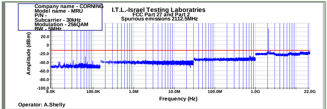
Figure 936: Spurious Emissions at Antenna Terminal 256QAM 5MHz B.W.; 2112.5MHz, 30kHz
