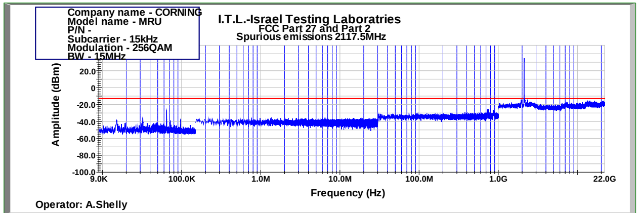
Figure 948: Spurious Emissions at Antenna Terminal 256QAM 15MHz B.W.; 2117.5MHz, 15kHz
