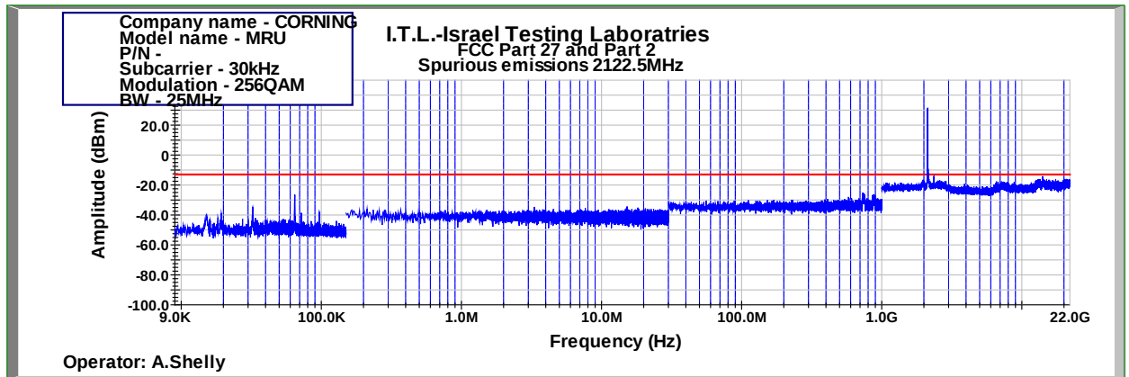
Figure 969: Spurious Emissions at Antenna Terminal 256QAM 25MHz B.W.; 2122.5MHz, 30kHz
