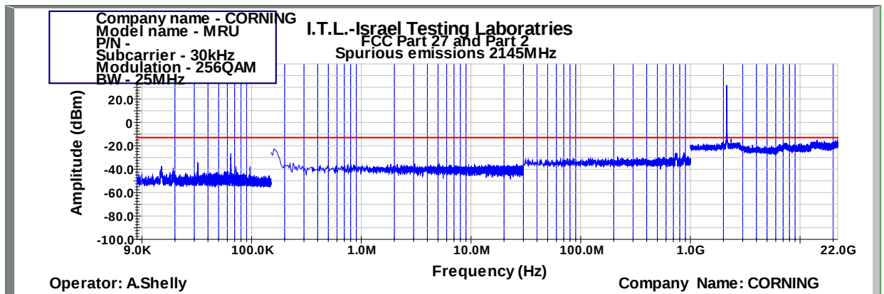
Figure 970: Spurious Emissions at Antenna Terminal 256QAM 25MHz B.W.; 2145.0MHz, 30kHz
