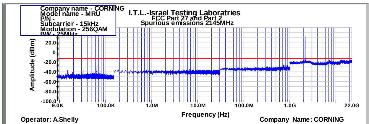
Figure 967: Spurious Emissions at Antenna Terminal 256QAM 25MHz B.W.; 2145.0MHz, 15kHz
