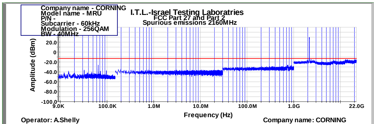
Figure 983: Spurious Emissions at Antenna Terminal 256QAM 40MHz B.W.; 2160.0MHz, 60kHz
