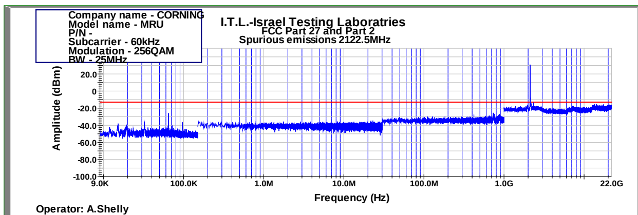
Figure 972: Spurious Emissions at Antenna Terminal 256QAM 25MHz B.W.; 2122.5MHz, 60kHz
