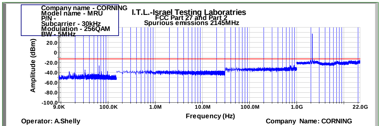
Figure 937: Spurious Emissions at Antenna Terminal 256QAM 5MHz B.W.; 2145.0MHz, 30kHz
