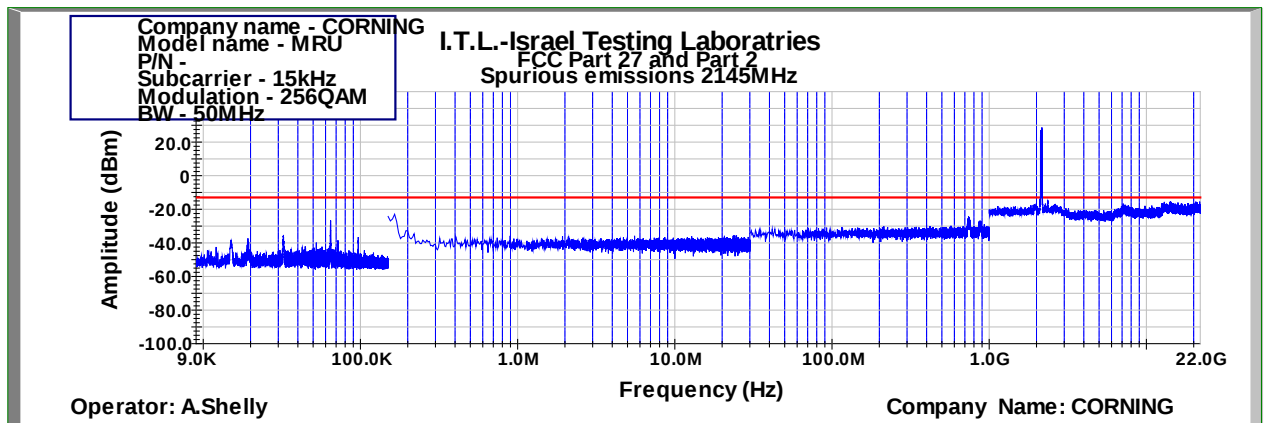
Figure 985: Spurious Emissions at Antenna Terminal 256QAM 50MHz B.W.; 2145.0MHz, 15kHz
