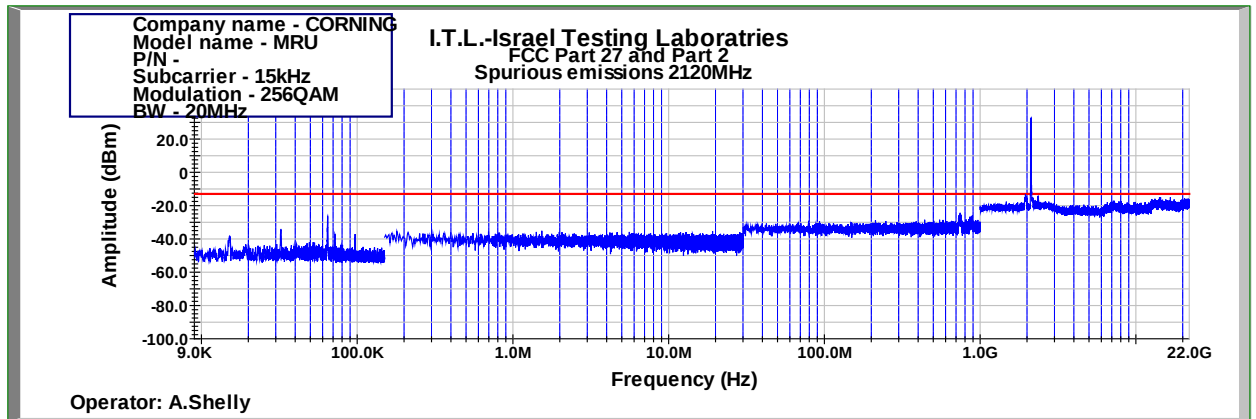
Figure 957: Spurious Emissions at Antenna Terminal 256QAM 20MHz B.W.; 2120.0MHz, 15kHz
