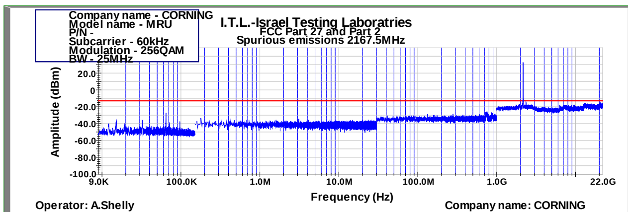
Figure 974: Spurious Emissions at Antenna Terminal 256QAM 25MHz B.W.; 2167.5MHz, 60kHz
