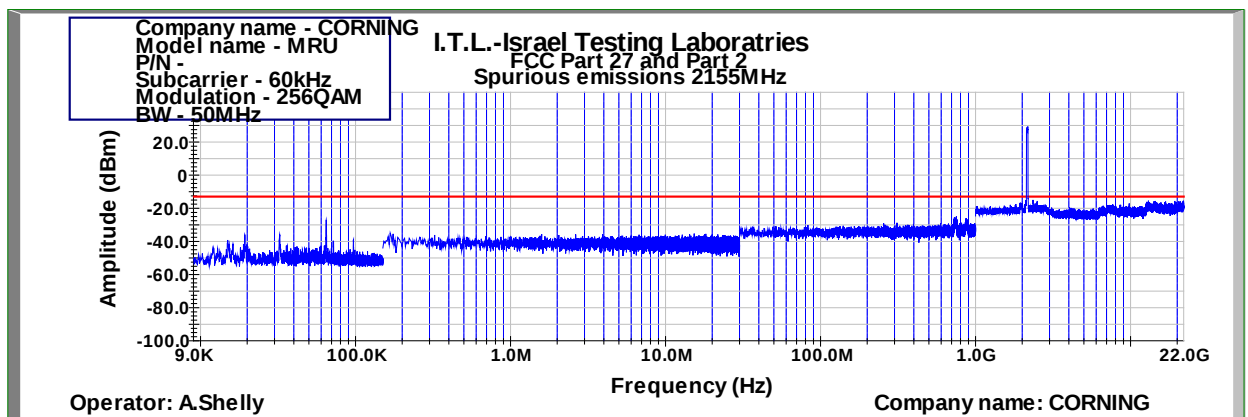
Figure 992: Spurious Emissions at Antenna Terminal 256QAM 50MHz B.W.; 2155.0MHz, 60kHz
