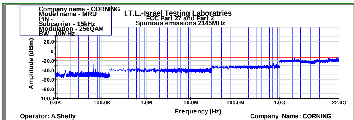
Figure 940: Spurious Emissions at Antenna Terminal 256QAM 10MHz B.W.; 2145.0MHz, 15kHz
