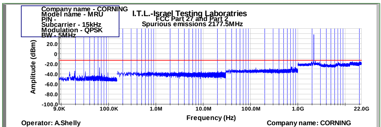
Figure 1001: Spurious Emissions at Antenna Terminal QPSK 5MHz B.W.; 2177.5MHz, 15kHz
