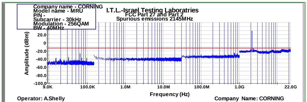
Figure 979: Spurious Emissions at Antenna Terminal 256QAM 40MHz B.W.; 2145.0MHz, 30kHz
