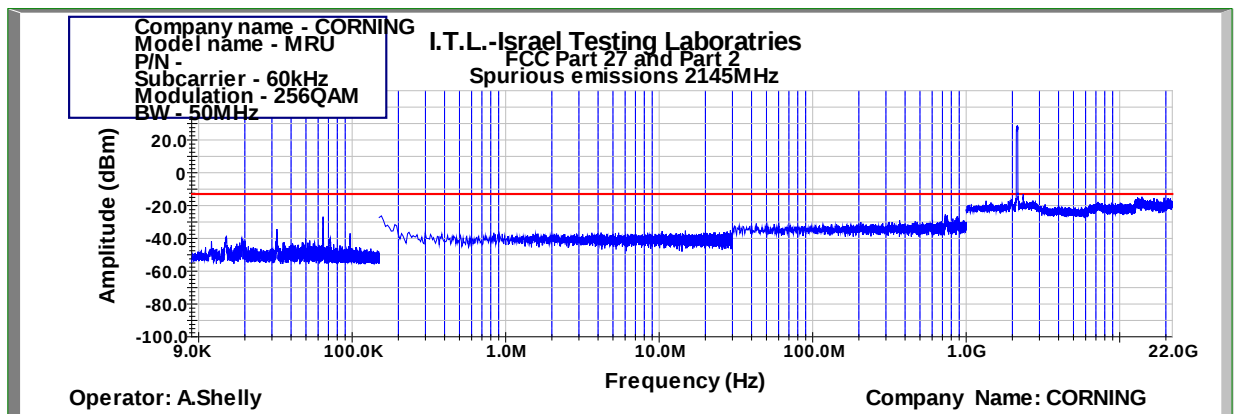
Figure 991: Spurious Emissions at Antenna Terminal 256QAM 50MHz B.W.; 2145.0MHz, 60kHz
